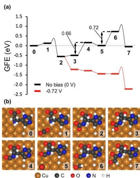
Figure 5 a) Gibbs free energy diagram and b) snapshots of the first few surface intermediates in the histidine-assisted CO 2 RR mechanism. Adapted with permission from Nat. Commun. , 2023, 14 , 335.
