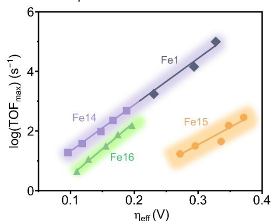
Figure 7 Scaling relationships for iron hangman porphyrins Fe14–Fe16 and Fe1 showing the effect of phenol (PhOH) concentration. For Fe14–Fe16 , [PhOH] = 2, 4, 10, 20, and 40 mM were tested. For Fe1 , [PhOH] = 0.1, 0.75, 3.0 M were used. In all cases, a higher phenol concentration led to a higher \text{TOF}_{\text{max}} . The slopes of the linear regions are 15.58, 11.65, and 18.08 dec V -1 for Fe1/Fe14 , Fe15 , and Fe16 , respectively.
