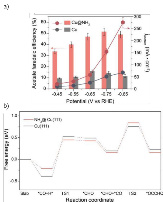
Figure 4 a) Acetate FE and partial current density for CO reduction on \text{Cu@NH}_2 and Cu recorded in CO-saturated 1.0 M KOH solution. b) Free energy diagram of the CO reduction mechanism showing ^*\text{CO} hydrogenation to ^*\text{CHO} and the subsequent coupling with another ^*\text{CO} to ^*\text{OCCHO} on \text{Cu@NH}_2(111) and Cu (111). Adapted with permission from ACS Catal. 2023, 13 , 3532–3540. Copyright 2023 American Chemical Society.
