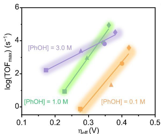
Figure 8 Scaling relationships for Fe21–Fe23 and Fe1 at different concentrations of phenol. \diamond = Fe1 , \circ = Fe21 , \Delta = Fe22 , \square = Fe23 . The slopes of the lines are purple = 10.3 dec V -1 , green = 28.2 dec V -1 , and orange = 24.10 dec V -1 .
