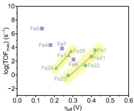
Figure 10 Overcoming linear scaling relations by amide-functionalized catalysts Fe4–Fe7 . All catalysts included in this plot were tested in the presence of 0.1 M PhOH.
