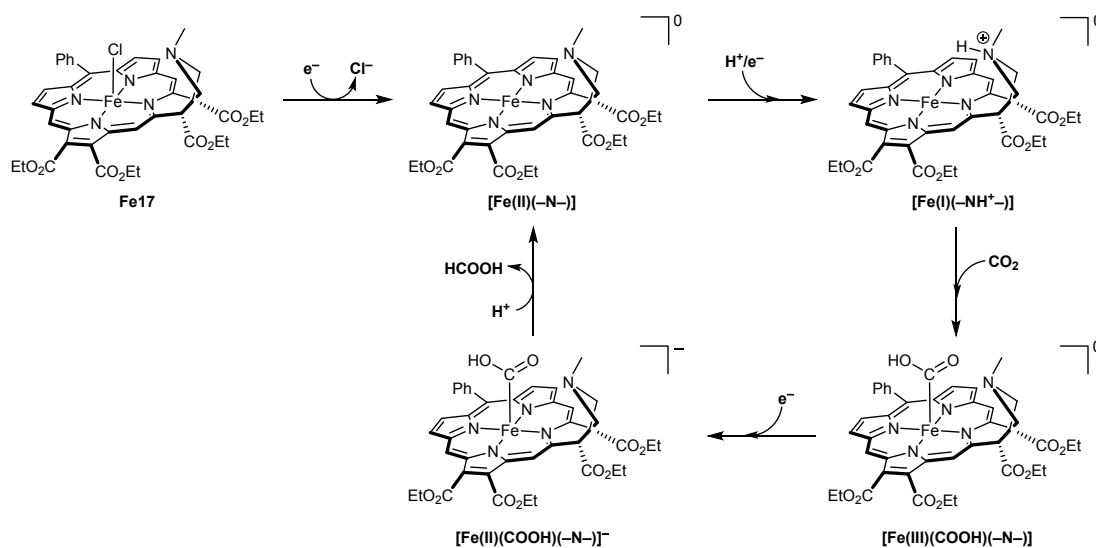
Scheme 6 The mechanistic pathway showing the formation of formate by Fe17 as proposed by Dey and coworkers.
