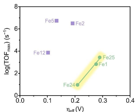
Figure 9 Breaking of the scaling relation set by Fe24 , Fe1 , and Fe25 (green) by functionalized catalysts Fe2 , Fe5 , and Fe12 (purple), all containing hydrogen-bonding/proton-donating organic groups in the second coordination sphere. The slope of the scaling relation set by Fe24 , Fe1 , and Fe25 is 29.7 dec V -1 . Fe1 , Fe24 , Fe25 , and Fe5 were tested in the presence of 0.1 M PhOH, while Fe2 and Fe12 were tested in the presence of 2.0 M and 5.5 M of water, respectively.
