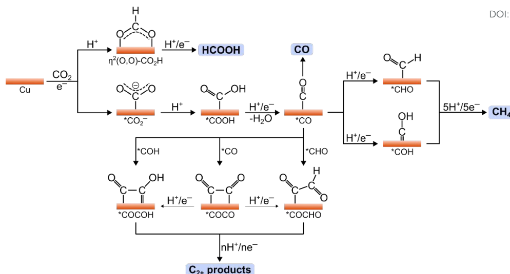
Figure 2 Mechanistic pathways in the CO 2 RR on Cu electrodes showing key intermediates toward HCOOH, CO, CH 4 , and C 2+ products.
