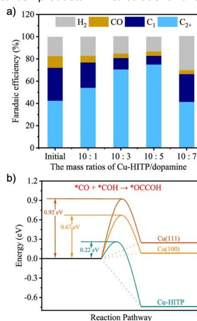
Figure 6 a) Comparison of CO 2 RR performances of Cu-HITP with different PDA coating amounts at –1.2 V vs RHE. b) Free energy diagram for forming the C–C bond on the Cu-HITP model. Adapted with permission from ACS Catal. , 2022, 12 , 7986–7993. Copyright 2022 American Chemical Society.
