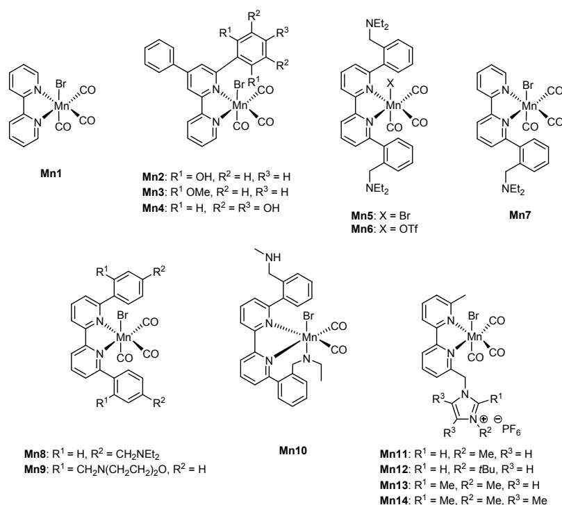
Scheme 9 Mn tricarbonyl bipyridine catalysts.
