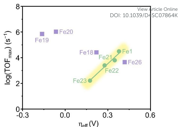
Figure 11 Iron porphyrins with cationic ( Fe18 , Fe19 , Fe20 ) and anionic ( Fe26 ) groups in the second coordination sphere circumventing the linear scaling relationship set by Fe1 and Fe21–Fe23 . The slope of the scaling relation is 28.2 dec V -1 . Fe1 and Fe21–Fe23 were tested in the presence of 1.0 M PhOH, Fe18 , Fe19 , Fe26 were tested in the presence of 0.1 M H 2 O and 3.0 M PhOH, and Fe20 was tested in the presence of 5.55 M H 2 O.
