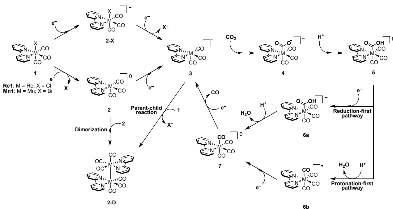
Scheme 2 Proposed CO 2 -to-CO reduction mechanism by rhenium and manganese bipyridine tricarbonyl catalysts, Re1 and Mn1 . DOI: 10.1039/D4SC07864K
