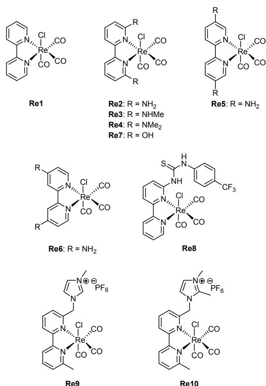
Scheme 8 Re tricarbonyl bipyridine catalysts.
