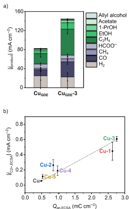
Figure 3. a) Electrocatalytic performance of the best-performing NHC-CDI-modified Cu catalyst ( \text{Cu}_{\text{GDE-3}} ) and a reference Cu catalyst ( \text{Cu}_{\text{GDE}} ) in a GDE-based electrolysis setup at -1.1 V vs RHE, and b) partial current density for multicarbon products, |j_{\text{C}2^+, \text{ECSA}}| , as a function of the accumulated surface charge, Q_{\text{an, ECSA}} , at \Delta E = 1.6 V. Adapted with permission from J. Am. Chem. Soc. 2024, 146 , 13034–13045. Copyright 2024 American Chemical Society.
