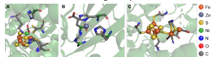
Figure 1. Microenvironments of distinct enzymes. a) [NiFe]-CO dehydrogenase displays a [3Fe-4S] cluster bonded to the Ni-Fe moiety. The Ni apex binds the C atom of the CO 2 substrate, while the acidic Fe center binds to the O atom. (Protein Data Bank identifier: 4UDX). b) Carbonic anhydrase features a Zn(II) atom coordinated to three histidine side-chains and a fourth histidine shuttling protons in and out of the active site via conformational switching (Protein Data Bank identifier: 1CA2). c) [FeFe] hydrogenase contains a cubane-shaped [4Fe4S] cluster coupled to a low valent di-iron center connected by a bridging thiolate ligand. The pendant secondary amine of this ligand can relay protons, facilitating H 2 activation at one of the Fe centers (Protein Data Bank identifier: 4XDC).
