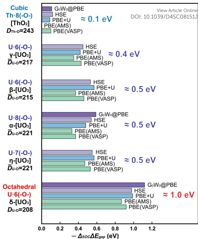
Fig. 2. Reduction of band gap by spin-orbit coupling (SOC), w.r.t. the scalar relativistic approximation.
