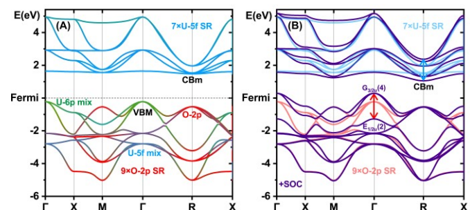
Fig. 6. Band structure of \delta -[UO 3 ] in the O-2p / U-5f6d valence and conduction regions.
