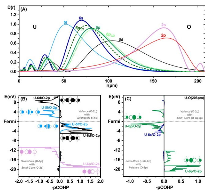
Fig. 3. Bonding analysis of \delta -[UO 3 ].
