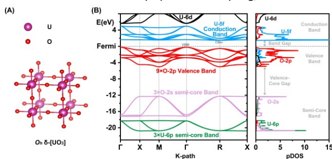
Fig. 1. Geometric and electronic structure of \delta -[UO 3 ].
