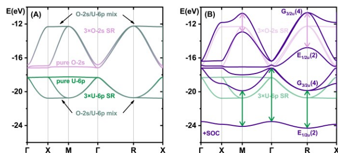
Fig. 5. Band structure of \delta -[UO 3 ] in the U-6p / O-2s semi-core region.
