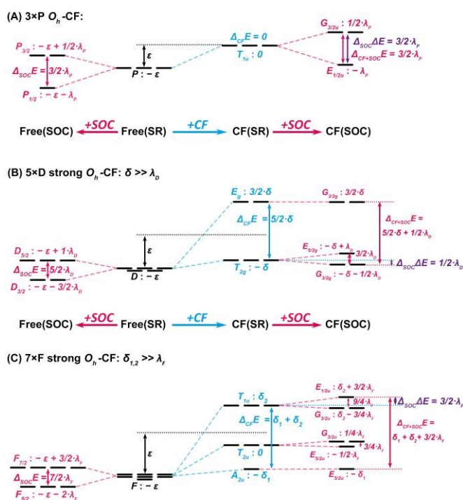
Fig. 4. O_h -Crystal-Field and Spin-Orbit effects on p, d and f orbital levels.
