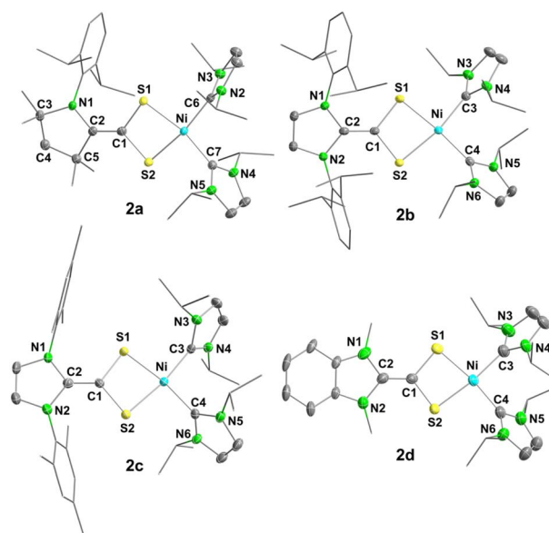
Fig. 1 Molecular structures of [\text{Ni}(\text{I}^t\text{Pr})_2(\text{cAAC}^{\text{Me}}\text{-CS}_2)] ( 2a , top left), [\text{Ni}(\text{I}^t\text{Pr})_2(\text{IDipp-CS}_2)] ( 2b , top right), [\text{Ni}(\text{I}^t\text{Pr})_2(\text{IMes-CS}_2)] ( 2c , bottom left), and [\text{Ni}(\text{I}^t\text{Pr})_2(\text{BIme-CS}_2)] ( 2d , bottom right) in the solid-state (ellipsoids set at the 50% probability level). The hydrogen atoms were omitted for clarity. Selected bond lengths [Å] and angles [°] are provided within Table 1 or in the captions of Fig. S72–S75 of the ESI.†
