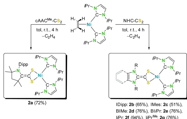
Scheme 4 Synthesis of mono-azolium-2-dithiocarboxylate nickel complexes of the type [\text{Ni}(\text{I}^t\text{Pr})_2(\text{carbene-CS}_2)] ( 2 ).
