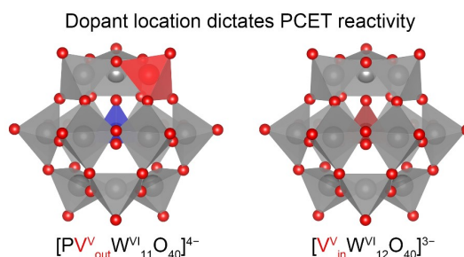
Figure 1. Molecular structure of vanadium-doped Keggin-type polyoxotungstates highlighting differences in accessibility of dopant ion – (left) surface V-substitution [PV_{out}W_{11}O_{40}]^{4-} versus (right) internal V-substitution [V_{in}W_{12}O_{40}]^{3-} studied in this work. Key: O, red spheres; P, blue polyhedra; V, red polyhedra; W, grey polyhedra.
