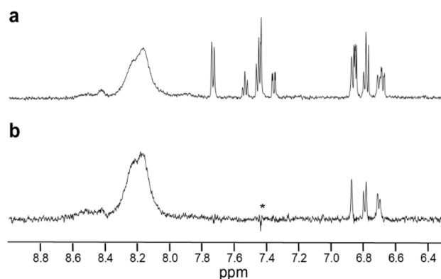
Fig. 6 ^1\text{H} NMR subspectra of 3-MT (50 \mu\text{M} ), hippuric acid (50 \mu\text{M} ), homovanillic acid (50 \mu\text{M} ), vanillic acid (50 \mu\text{M} ) and ProAlaAsp (500 \mu\text{M} , ligand concentration). Conditions: 500 MHz, 25 ^\circ\text{C} , [HEPES] = 1 mM, \text{pD} = 7.0 , \text{H}_2\text{O}/\text{D}_2\text{O} 90:10. (a) ^1\text{H} spectrum (128 scans); (b) HPwSTD spectrum (512 scans). Signals at 8.2 ppm belong to amide protons that receive saturation via chemical exchange with \text{H}_2\text{O} . The asterisk denotes a subtraction artifact. The full HPwSTD spectrum is reported in Fig. S48.†
