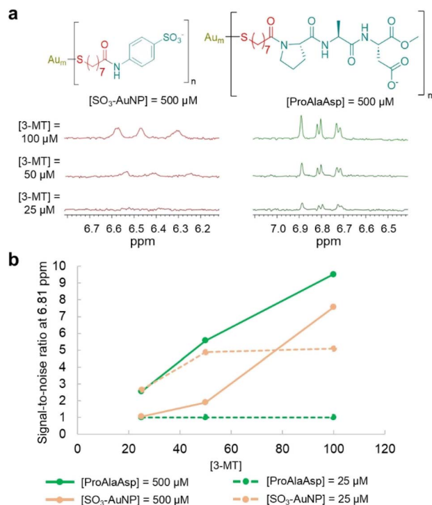
Fig. 5 (a) HPwSTD subspectra of 3-MT (25–100 \mu M) and SO 3 –AuNP or ProAlaAsp (500 \mu M, ligand concentration). Conditions: 500 MHz, 25 ^{\circ} C, [HEPES] = 1 mM, pD = 7.0, H 2 O/D 2 O 90:10, 512 scans. (b) Signal-to-noise ratio of the 3-MT signal at 6.81 ppm ([3-MT] = 25–100 \mu M) with SO 3 –AuNP or ProAlaAsp at 25 \mu M or 500 \mu M. Full spectra are reported in Fig. S47.†
