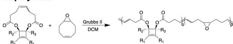
Scheme 1. Synthesis of co-monomers and polymers employed in this work.
