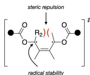
Figure 4. Schematic showing how substituents that are anti to the pulling attachments and on the scissile bond generate increased steric repulsion in a disrotatory process.
