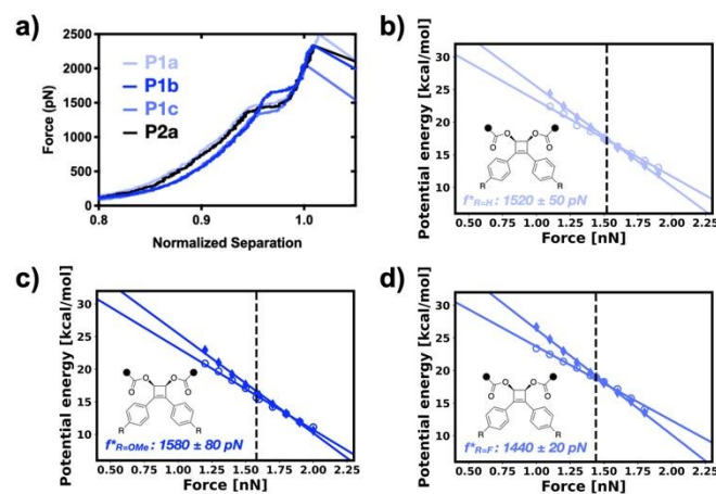
Figure 2. (a) Representative single-molecule force spectroscopy data of cyclobutene mechanophores as a function of alkene substituent. Computed activation energies as a function of force for (b) P1a , (c) P1b , and (d) P1c . The conrotatory reactions are shown in open symbols; disrotatory reactions are shown in filled symbols. Vertical dashed lines correspond to the respective average plateau forces observed experimentally.
