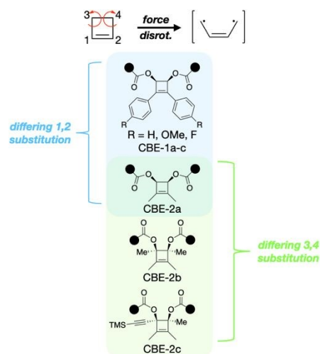
Figure 1. Force applied through ester substituents is used to drive the disrotatory ring opening of a range of cyclobutene mechanophores with different substituents.
