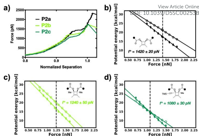
Figure 3. (a) Representative single-molecule force spectroscopy data of cyclobutene mechanophores as a function of substituent on the scissile carbon-carbon bond. Computed activation energies as a function of force for (b) P2a , (c) P2b , and (d) P2c . The conrotatory reactions are shown in open symbols; disrotatory reactions are shown in filled symbols. Vertical dashed lines correspond to the respective average plateau forces observed experimentally.
