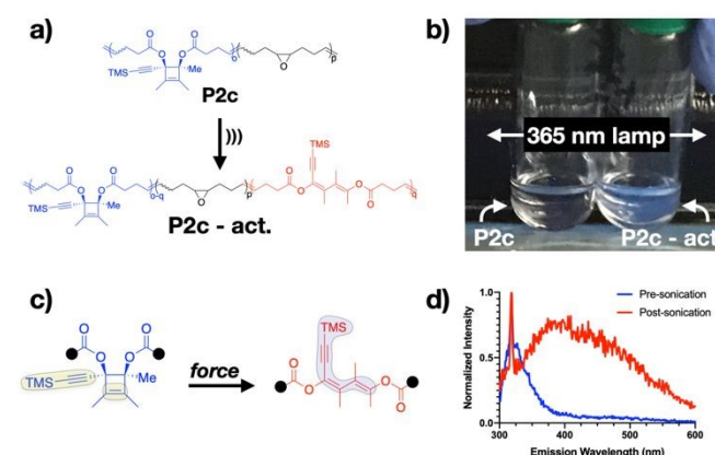
Figure 5. (a) Sonication of P2c opens the cyclobutene ring, leading to observed fluorescence in the post-sonicated solution (b). The fluorescence is attributed to increased conjugation, including that into the alkyne substituent (c). (d) Emission spectrum of pre- and post-sonication solutions of P2c .
