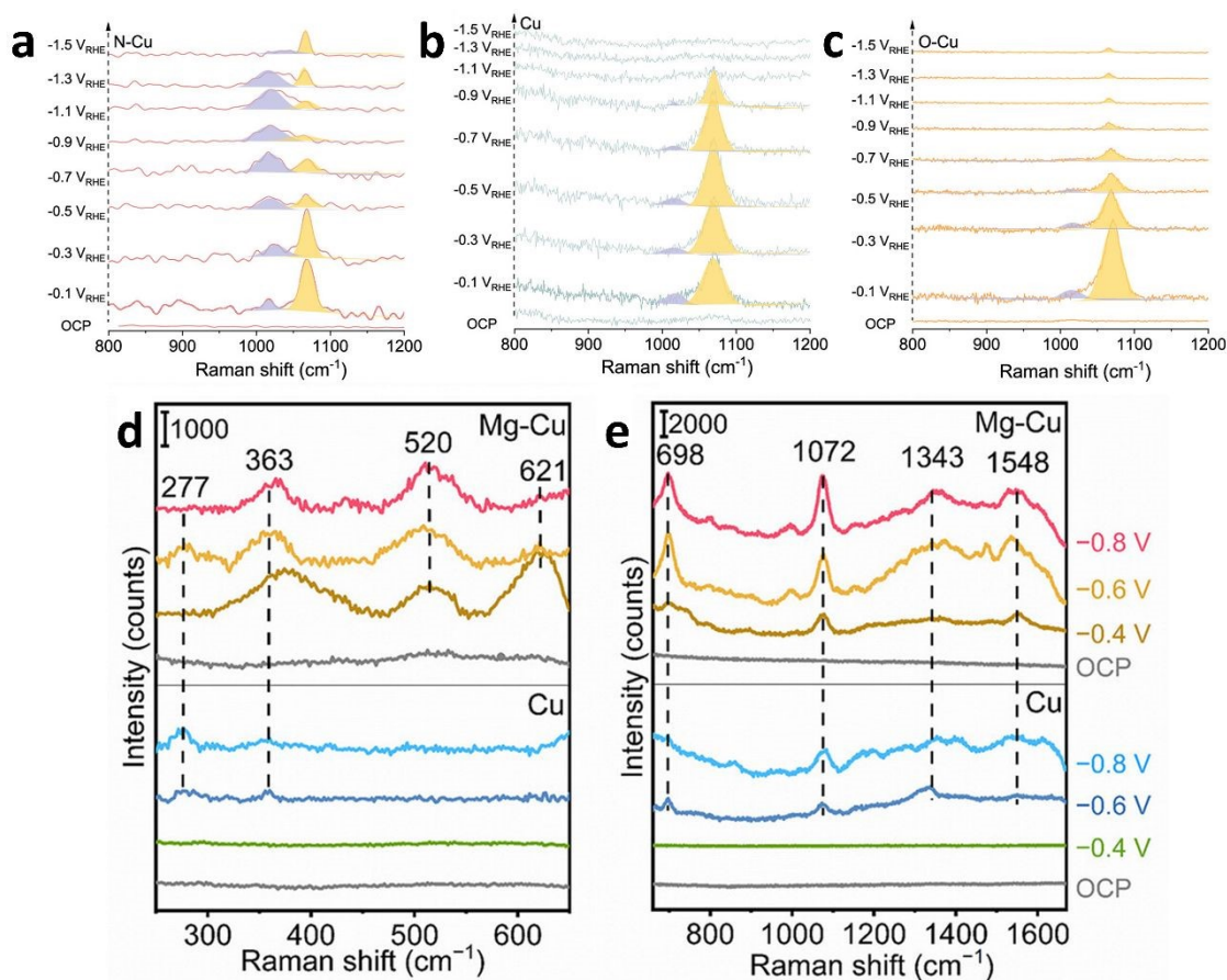
Fig. 7 In situ SERS of different Cu-based catalysts under \text{CO}_2\text{RR} conditions. (a) N-Cu; (b) Cu; (c) O-Cu. (a-c) are reproduced from ref. 124 with permission from American Chemical Society, copyright 2022. (d) Low energy region and (e) high energy region of in situ Raman spectra for Cu and Mg-Cu within a \text{CO}_2 -saturated 0.5 M \text{KHCO}_3 electrolyte at various potentials (V vs RHE). (d) and (e) are reproduced from ref. 128 with permission from Wiley, copyright 2022.
