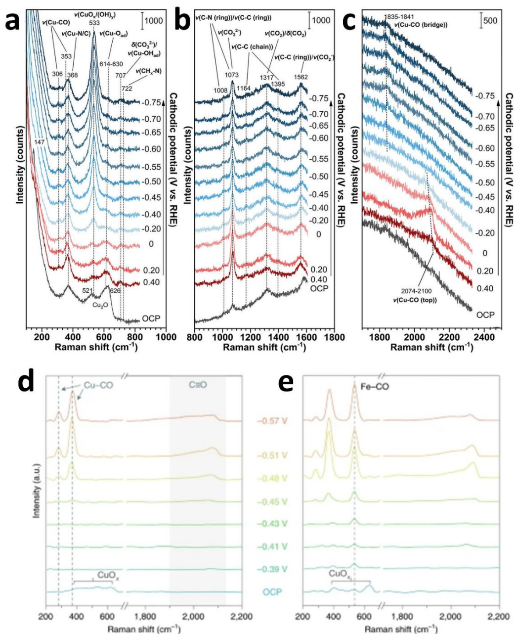
Fig. 9 (a-c) In situ Raman spectra obtained on GDE loaded with Cu 0 @PIL@Cu -5 at various cathodic potentials across different Raman shift ranges. (c) and (d) are reproduced from ref. 134 with permission from Wiley, copyright 2021. In situ Raman spectra of the Cu (d) and FeTPP[Cl]/Cu (e) catalysts under varying applied potentials. (c) and (d) are reproduced from ref. 137 with permission from Springer Nature Links, copyright 2020.
