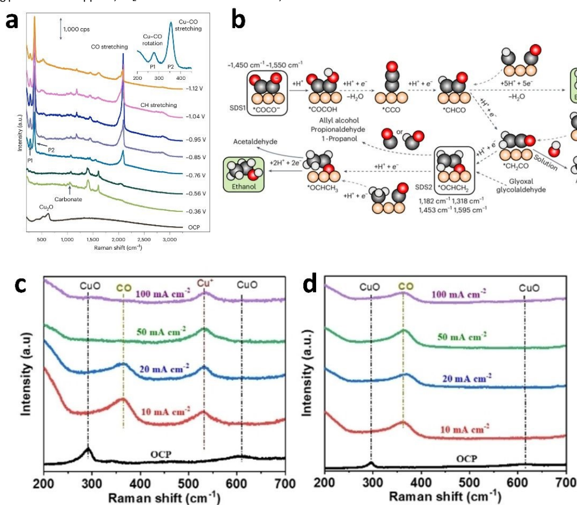
Fig. 6 (a) Raman spectra obtained from electrochemically treated Cu foil during eCO 2 RR within potentials range from the open-circuit potential (OCP) to about -1.1 V vs RHE in a 0.1 M NaClO 4 electrolyte that had been saturated with CO 2 gas. (b) Proposed reaction scheme for the generation of ethylene and ethanol. (a) and (b) are reproduced from ref. 119 with permission from Springer Nature Link, copyright 2024. Operando Raman spectra analysis during CO 2 RR at varying current densities. (c) CuO x @C. (d) CuO x . (c) and (d) are reproduced from ref. 122 with permission from Wiley, copyright 2022.
