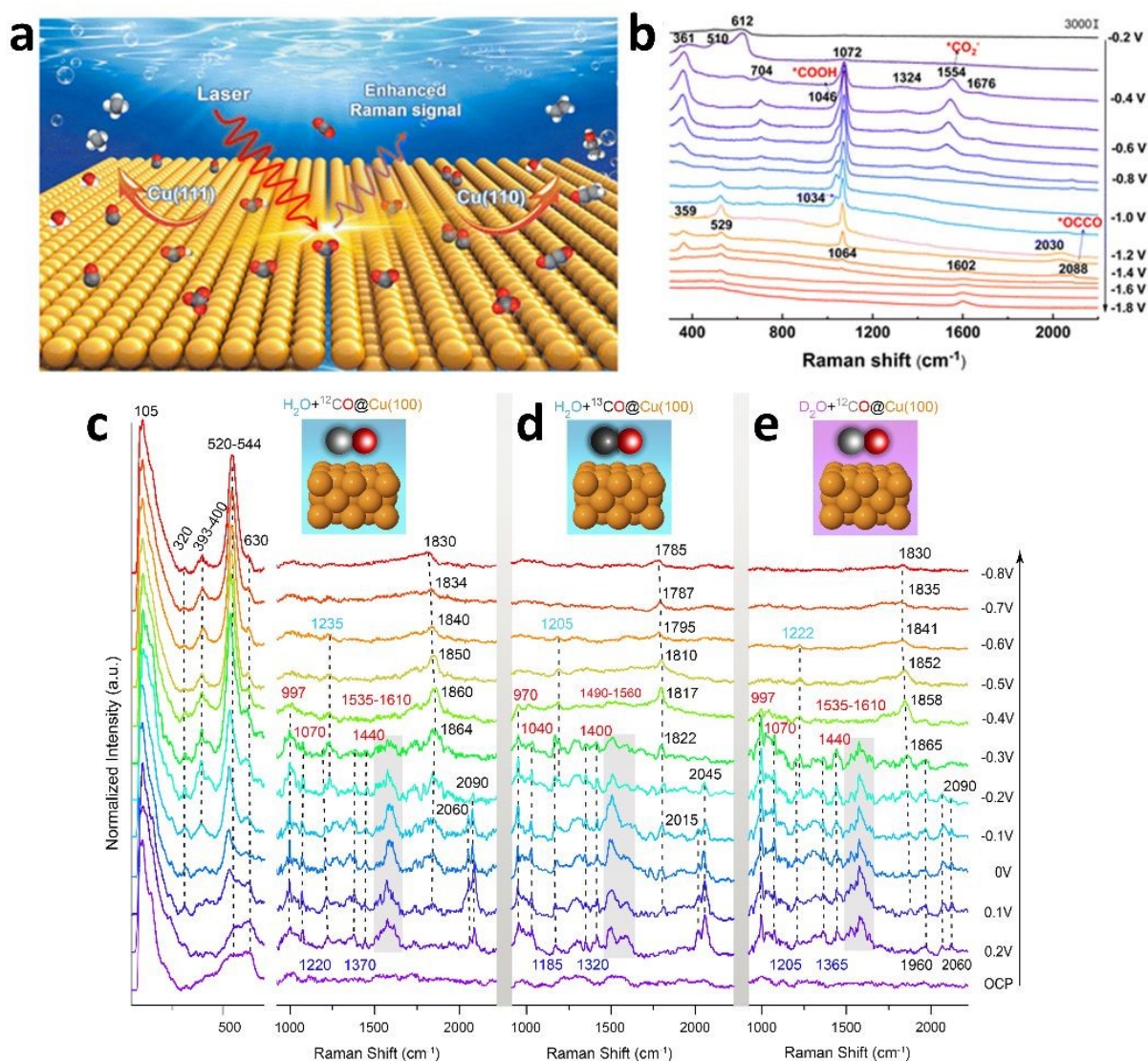
Fig. 5 (a) Diagrams illustrating the capture of intermediate species in \text{eCO}_2\text{RR} on Cu(111) and Cu(110) single-crystals by in situ Raman spectroscopy. (b) In situ Raman spectra of Cu(110) in a 0.5 M \text{KHCO}_3/\text{H}_2\text{O} solution saturated with \text{CO}_2 at various potentials (vs SCE). (a) and (b) are reproduced from ref. 112 with permission from The Royal Society of Chemistry, copyright 2022. (c-e) Potential-dependent EC-SHINERS spectra obtained from Cu(100) single-crystal in the presence of (c) ^{12}\text{CO} and (d) ^{13}\text{CO} and (e) with \text{D}_2\text{O} as electrolyte. The solutions were saturated with ^{12}\text{CO} or ^{13}\text{CO} gases and 0.1 M CsOH/OD electrolyte with a pH of 13. The Cu, ^{12}\text{C} , ^{13}\text{C} , and O atoms are depicted in orange, gray, black, and red colors, respectively. (a) and (b) are reproduced from ref. 116 with permission from the National Academy of Sciences of the United States of America, copyright 2022.
