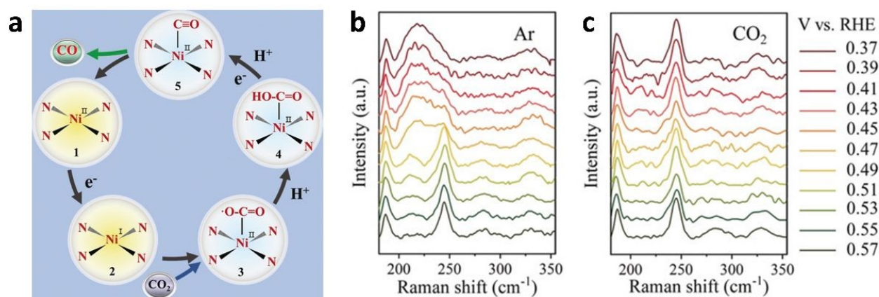
Fig. 4 (a) Proposed \text{CO}_2 reduction to CO pathway on the Ni SAC; Raman spectra of Ni-TAPc obtained on an Au electrode at different potentials (vs RHE) in 0.5 M \text{KHCO}_3 aqueous solution at room temperature under (b) Ar and (c) \text{CO}_2 atmospheres. (a-c) are reproduced from ref. 102 with permission from Wiley, copyright 2019.
