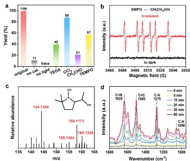
Fig. 4 The characterization of the reaction mechanism. (a) The photocatalytic performance of control experiments over Zr-NDI •− . (b) EPR spectra of Zr-NDI •− in the presence of DMPO as a trapping agent under light irradiation and in the dark. (c) HRMS spectra of the DMPO adduct to the • CH(CH 3 )OH intermediate under the standard conditions ([M + H] + C 8 H 18 O 2 N + : 160.2333, found: 160.1329). (d) In situ DRIFTS of the photocatalytic synthesis of 2MBZ using OPD and ethanol as reactants over Zr-NDI •− .
