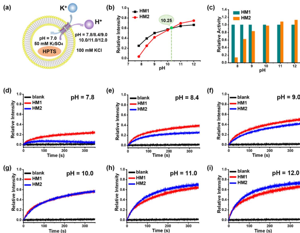
Fig. 5 (a) Schematic representation of transmission experiment in liposome vesicle of HM2 . (b) and (c) The normalized transport activities of HM1 and HM2 at the concentration of 1 \mu\text{M} with pH variation from 7.8 to 12.0. (d)–(i) Normalized \text{K}^+ transport activities of HM1 and HM2 at the concentration of 1 \mu\text{M} at different pH.
