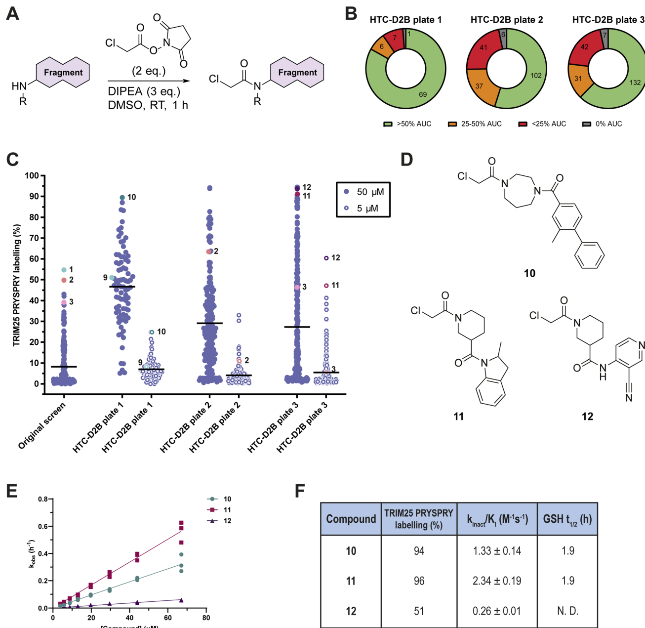
Fig. 2 High-throughput chemistry direct-to-biology (HTC-D2B) optimisation of fragments 1–3 . (A) HTC reaction scheme; 44 (B) pie charts of HTC conversion analysed by LCMS across HTC-D2B plate 1 (83 compounds, based on 1 ), HTC-D2B plate 2 (186 compounds, based on 2 ), and HTC-D2B plate 3 (212 compounds, based on 3 ). % AUC (area under the curve) represents AUC for the product-containing peak relative to the starting material-containing peak, selected on identification of the expected m/z ; 47 (C) comparison of % labelling of TRIM25 PRYSPPY (0.5 \mu M) by the original fragment library (50 \mu M) and each HTC-D2B library (50 \mu M and 5 \mu M) at 4 °C for 24 h. Black lines represent mean % labelling. Fragment 1 was not included in HTC-D2B plate 1, so a close analogue is highlighted instead ( 9 , structure shown in Fig. S4B, ESI†); (D) chemical structures of optimised chloroacetamides selected for progression; (E) k_{\text{obs}} ( \text{h}^{-1} ) plotted against concentration ( \mu M), fitted using a straight line fit. Data are presented as n = 3 ; (F) table of % labelling, k_{\text{inact}}/K_{\text{i}} ( \text{M}^{-1} \text{s}^{-1} ) values (mean \pm SD, n = 3 ), and t_{1/2} (h) (in the presence of 4 mM GSH) for compounds 10 , 11 and 12 .
