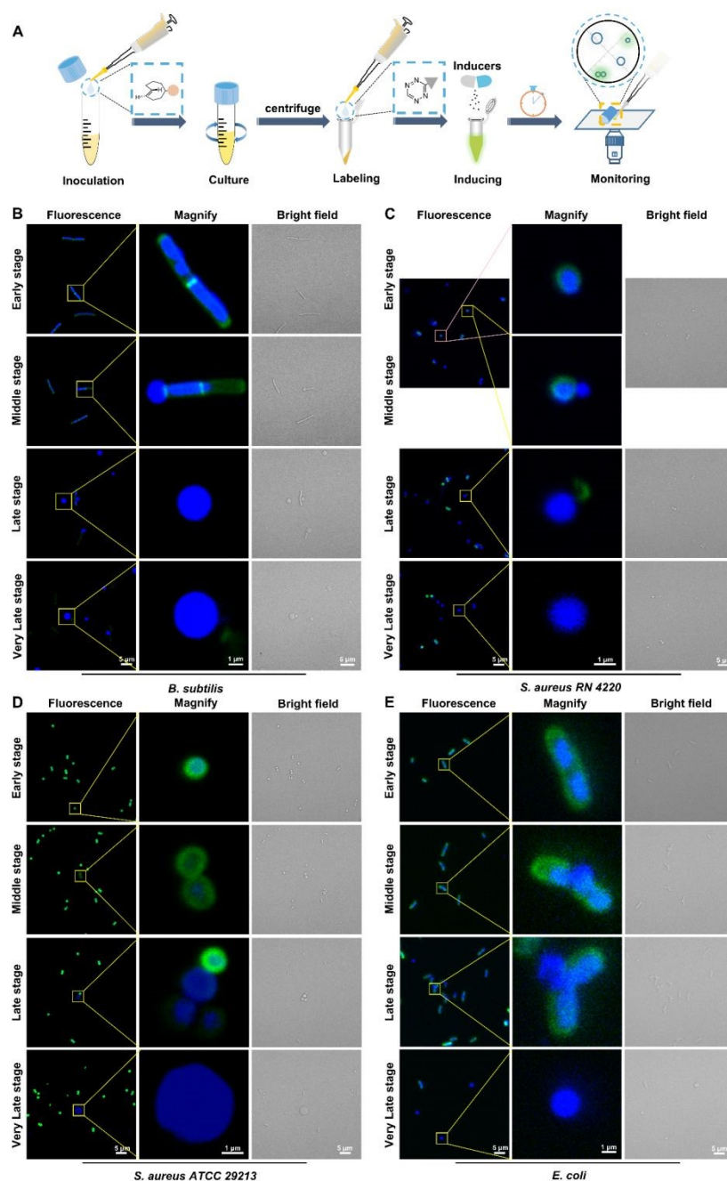
Fig. 3. Fluorescence images of different stages of bacterial L-form conversion. (A) A simplified workflow for monitoring bacterial L-form conversion. Bacteria labeled with Hoechst 33342 and Tz-FL-S were subjected to various induction conditions and monitored by CLSM. (B) Labeled B. subtilis ATCC 6633 were induced with 200 \mu\text{g/mL} penicillin G and 100 \mu\text{g/mL} lysozyme at 30 ^{\circ}\text{C} in NB/MSM medium. (C) Labeled S. aureus ATCC RN 4220 were induced with 200 \mu\text{g/mL} penicillin G and 2 \mu\text{g/mL} lysostaphin at 30 ^{\circ}\text{C} in NB/MSM medium. (D) Labeled S. aureus ATCC 29213 were induced with 400 \mu\text{g/mL} fosfomycin (FOS) at 30 ^{\circ}\text{C} in NB/MSM medium. (E) Labeled E. coli ATCC 25922 were induced with 100 \mu\text{g/mL} penicillin G and 100 \mu\text{g/mL} fosfomycin at 30 ^{\circ}\text{C} in NB/MSM medium. Scale bar: 5 \mu\text{m} . For the magnified images, the scale bar is 1 \mu\text{m} .
