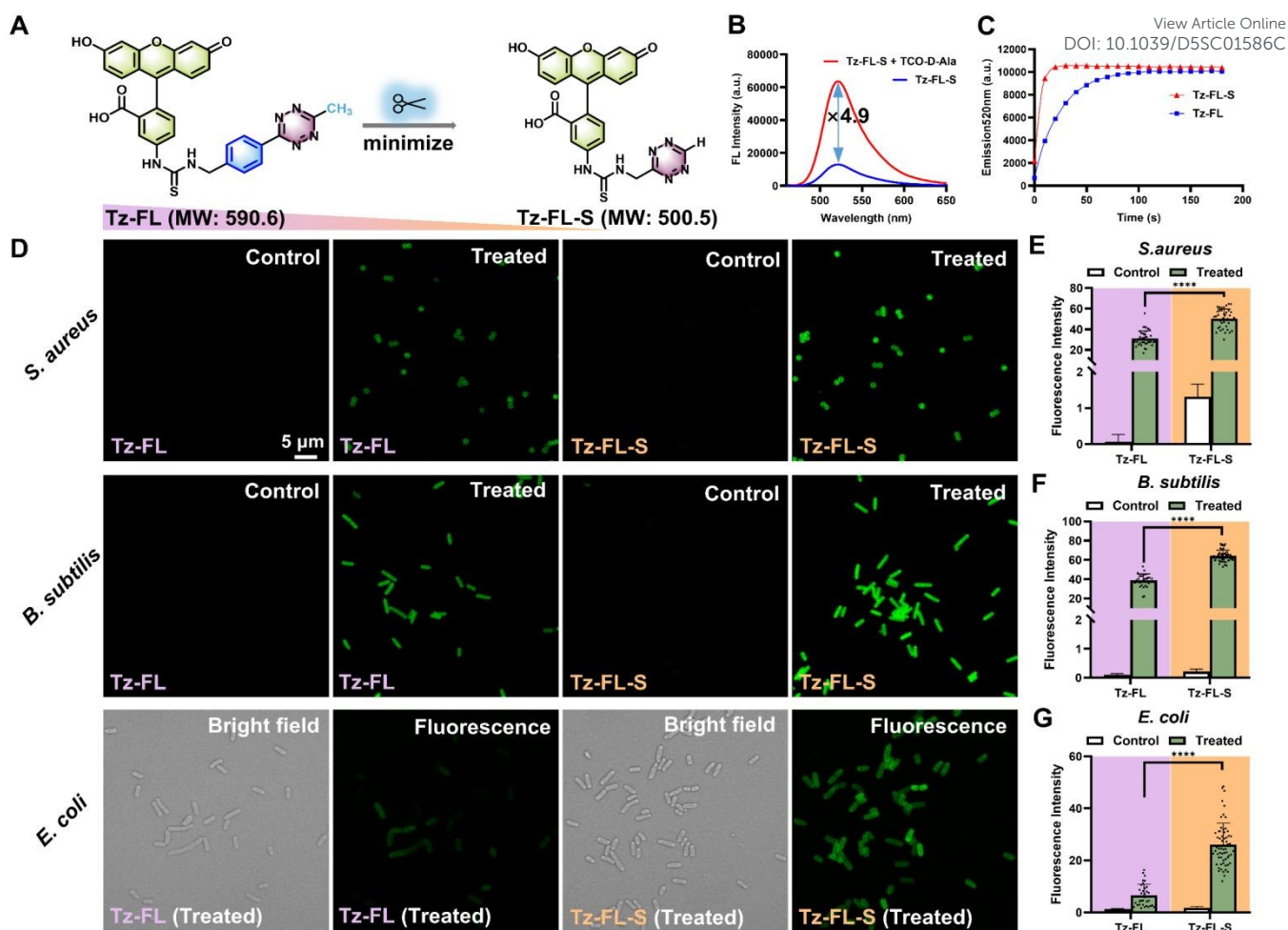
Fig. 2. Probe Optimization. (A) Strategy to optimize Tz-FL into Tz-FL-S by removing the benzene ring in the linker and the methyl group from the tetrazine head. (B) Fluorescence spectra of Tz-FL-S before and after reacting with TCO-D-Ala in pH 7.4 PBS, \lambda_{\text{ex}} = 488 nm. (C) Plot of fluorescence intensity at 520 nm versus time. Tz-FL-S exhibited a faster reaction than Tz-FL . \lambda_{\text{ex}} = 488 nm. (D) Labeling of S. aureus ATCC 29213, B. subtilis ATCC 63501, and E. coli ATCC 25922 with Tz-FL or Tz-FL-S . Green fluorescence images for each strain were collected and processed under the same conditions. For Hoechst staining images in the Tz-FL-S group, see Fig. S3C. Scale bar: 5 \mu\text{m} . (E), (F), and (G) Mean fluorescence intensity of bacteria labeled by Tz-FL and Tz-FL-S from panel (D) ( n \geq 30 ). Data are represented as mean \pm SD and analyzed using a two-tailed Mann-Whitney U test. **** P < 0.0001 .
