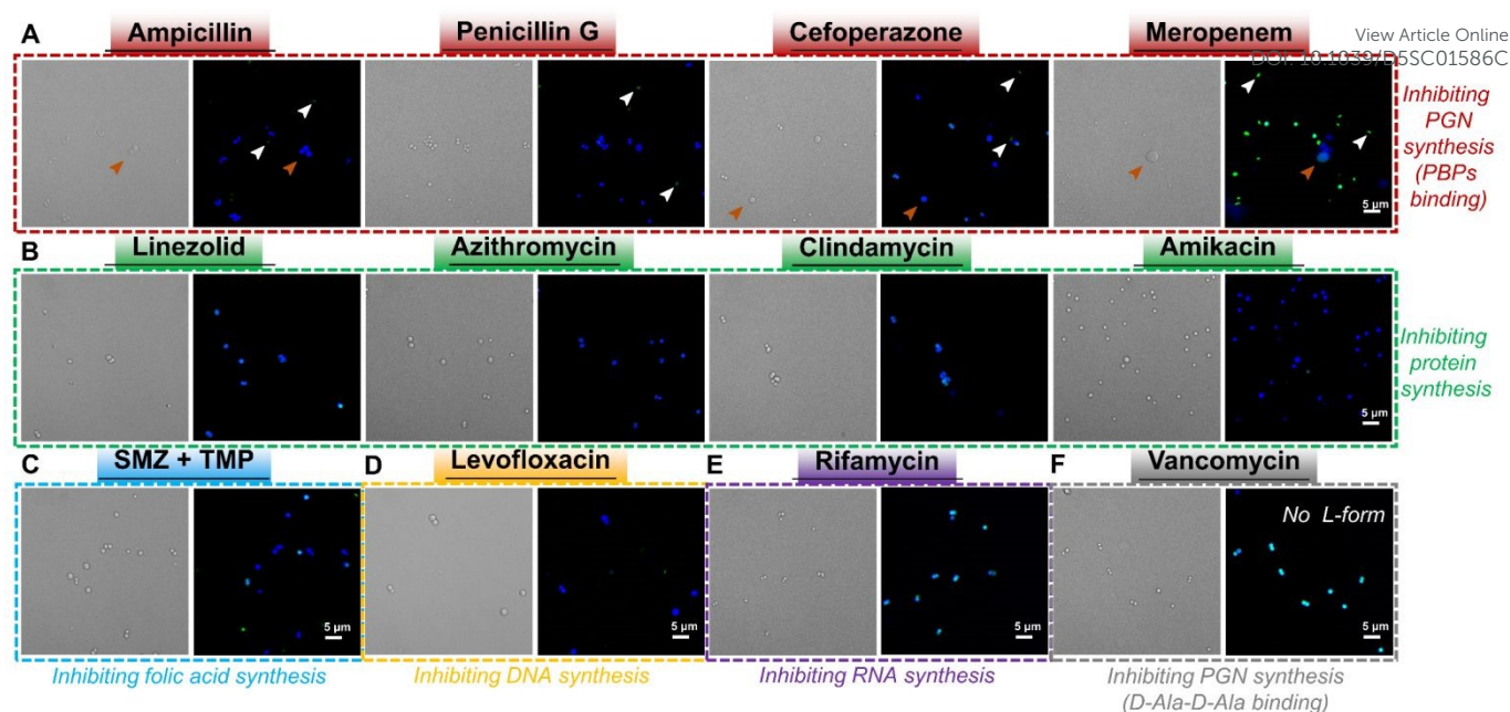
Fig. 4. Confocal fluorescence images of CWDB formation in S. aureus ATCC 29213 after treatment with various inducers. S. aureus cells were pre-labeled with Hoechst 33342 (blue) and Tz-FL-S (green), then exposed to antibiotics at 10 \times MIC in NB/MSM medium at 30^\circ\text{C} for 24 hours. The antibiotics inhibiting: (A) peptidoglycan synthesis via binding PBPs, (B) protein synthesis, (C) folic acid synthesis, (D) DNA synthesis, (E) RNA synthesis, (F) peptidoglycan synthesis via binding D-Ala-D-Ala terminus. White arrows indicate fusiform peptidoglycan shells or fragments, and orange arrows highlight swollen cells. SMZ: sulfamethoxazole, TMP: trimethoprim. Scale bar: 5\ \mu\text{m} .
