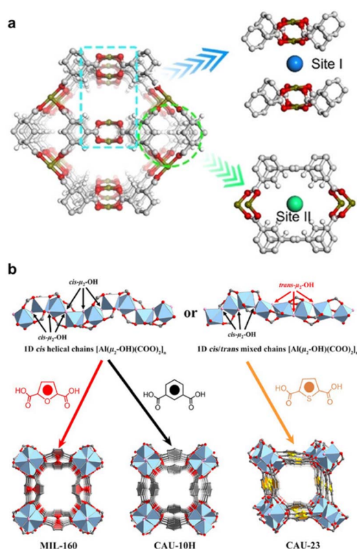
Fig. 10 (a) The channel structure of ATC-Cu and the two primary \text{C}_2\text{H}_2 binding sites within the framework. Reproduced with permission. 200 Copyright 2021, American Chemical Society. (b) 1D chains [\text{Al}(\mu_2\text{-OH})(\text{COO})_2]_n and V-shaped ligands ( \text{H}_2\text{FDC} , m\text{-H}_2\text{BDC} , and \text{H}_2\text{TDC} ) assemble into three isostructural 3D frameworks of MIL-160, CAU-10H, and CAU-23, respectively. Hydrogen atoms are omitted for clarity. Color code, Al: pale blue; O, red and rose; C, 50% gray. Reproduced with permission. 201 Copyright 2021, American Chemical Society.
