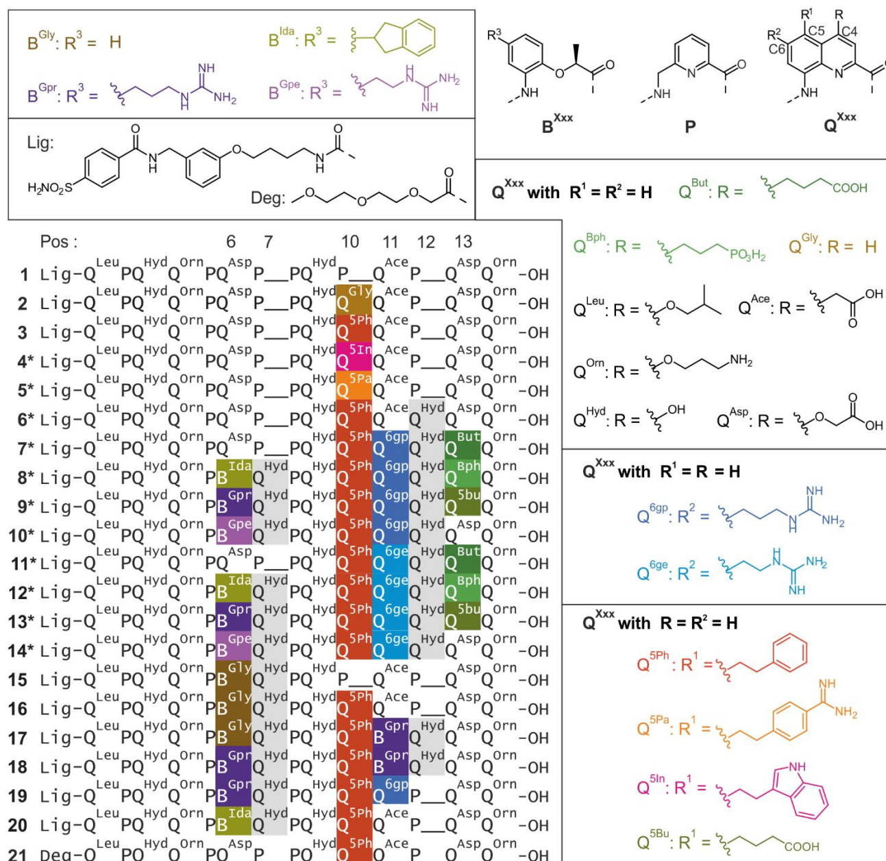
Fig. 3. Structural formulas of P, Q Xxx , and B Xxx δ-amino acids and of N-terminal Lig and Tail functional groups. Carbon atoms in position 4, 5, and 6 of Q Xxx are indicated and carry R, R 1 , and R 2 side chains, respectively. The Xxx three letter code used for the side chains is sometimes inspired by the three letter code of α-amino acids bearing similar side chains, even when they may not exactly match. The three letter code also indicates when the side chain is in position 5 or 6 of the quinoline ring. Sequences 1-21 are defined with the letter code
