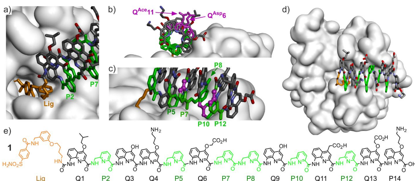
Fig. 2. a), b), c) and d) show different views of the solid state structure of the complex between HCAII and AOF 1 . 9 Only the surface of the protein is shown. The foldamer is shown in stick representation. Pyridine units (P) are shown in green and the HCAII ligand is shown in gold. In b), two residues of interest are shown in purple. In c) three carbon atoms of three P residues are shown in purple balls. These carbons would belong to the additional benzenic ring when implementing a P→Q mutation at these positions. Hydrogen atoms have been omitted for clarity. e) Structural formula of 1 .
