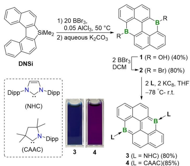
Scheme 1. Synthetic routes to 3 and 4 (Photographs of the solutions of 3 and 4 in o -difluorobenzene ( o -DFB) under room light). NHC = 1,3-bis(2,6-diisopropylphenyl)imidazol-2-ylidene, CAAC = 1-(2,6-diisopropylphenyl)-3,3,5,5-tetramethylpyrrolidin-2-ylidene.
