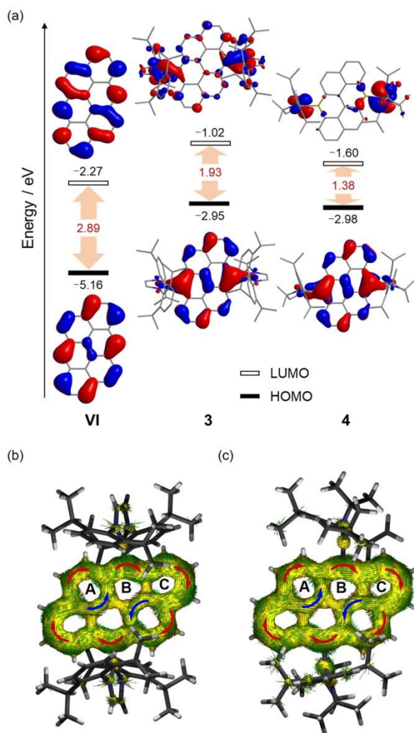
Figure 4. Plots of the HOMO and LUMO of 3 , 4 and all-carbon anthanthrene VI (hydrogen atoms are omitted for clarity, isovalue = 0.03) (a), and the ACID plots ( \pi -electron only) of 3 (b) and 4 (c) (the external magnetic field is applied orthogonal to the plane, and the red and blue arrows indicate the clockwise (diamagnetic) and counter-clockwise (paramagnetic) current flow, respectively).
