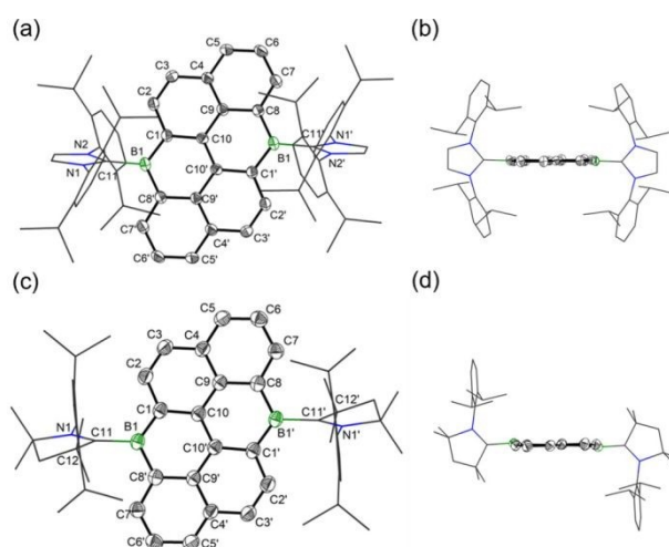
Figure 2. Molecular structures of 3 : top view (a) and side view (b), and 4 : top view (c) and side view (d). Thermal ellipsoids are set at the 50% probability. Hydrogen atoms and solvent molecules are omitted for clarity. Selected bond lengths (Å) and angles (°). 3 : B1-C11: 1.590(3), B1-C1: 1.485(4), C1-C10: 1.456(3), C10-C10': 1.431(4), C10'-C9': 1.443(3), C9'-C8': 1.444(3), C8'-B1: 1.515(4); C11-B1-C1: 120.6(2), C1-B1-C8': 119.4(2), C11-B1-C8': 120.0(8). 4 : B1-C11: 1.610(3), B1-C1: 1.491(4), C1-C10: 1.460(3), C10-C10': 1.435(4), C10'-C9': 1.442(3), C9'-C8': 1.440(3), C8'-B1: 1.517(4); C11-B1-C1: 122.8(2), C1-B1-C8': 117.8(2), C11-B1-C8': 118.4(2).
