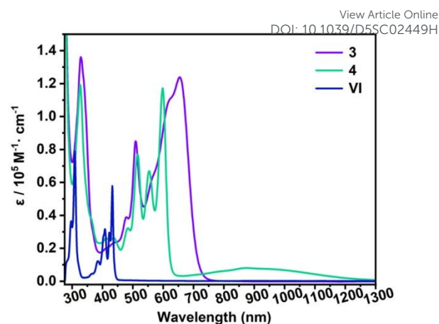
Figure 3. UV-Vis absorption spectra of 3 , 4 and all-carbon anthanthrene ( VI ) in o -difluorobenzene.
