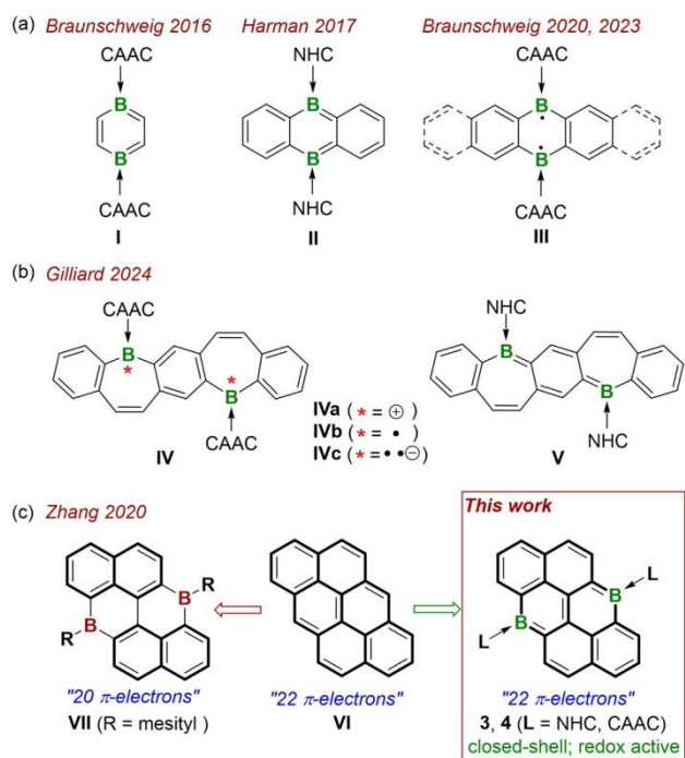
Figure 1. (a) Neutral 1,4-diborabenzene I and its lateral extended acenes II and III . (b) Bis-borepin IV with various redox states and dibora-quinone V . (c) all-carbon anthanthrene VI , boron-doped anthanthrene VII and 6,12-diboraanthanthrenes 3 and 4 (this work).
