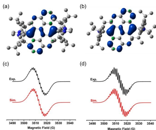
Figure 7. Spin density distribution of 6 (a) and 7 (b) at UB3LYP/6-311G(d, p) level (isovalue = 0.002, H atoms omitted for clarity), and experimental CW X-band (black trace) and simulated (red trace) EPR spectra of 6 (c) and 7 (d) in o -difluorobenzene at room temperature.
