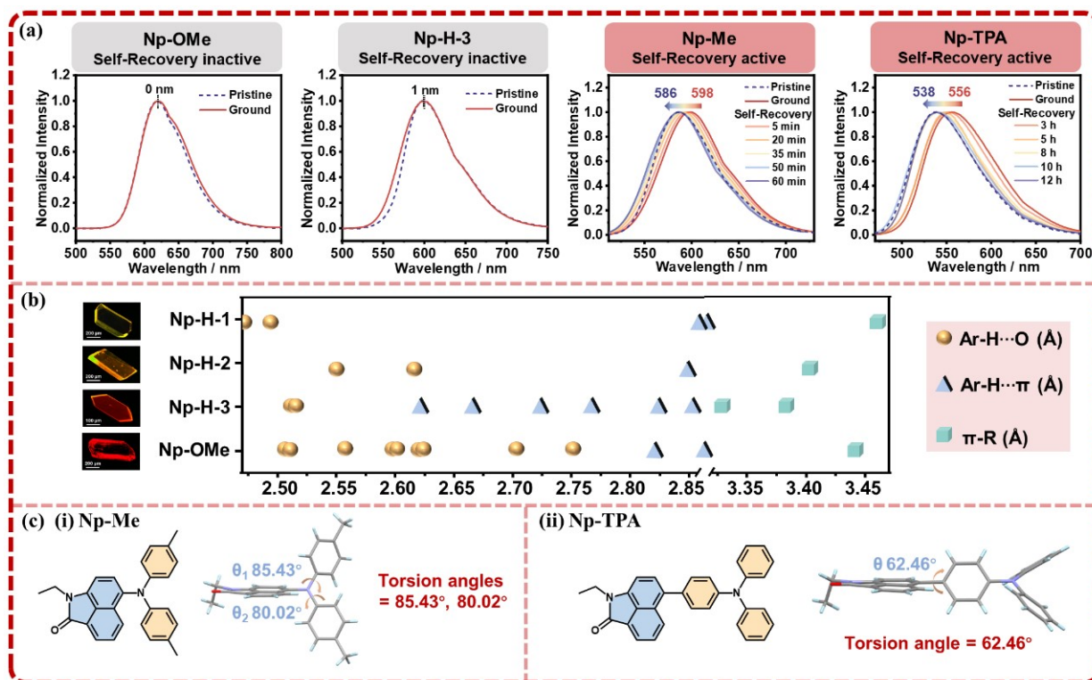
Fig. 4 (a) Normalized PL spectra of pristine Np-OMe, Np-H-3, Np-Me, and Np-TPA microcrystals (dotted line) during the grinding-recovering (solid line) process. (b) Statistical chart of intermolecular interactions for locking the phenyl rotations. (c) The molecular formula and conformation of i) Np-Me, ii) Np-TPA.
