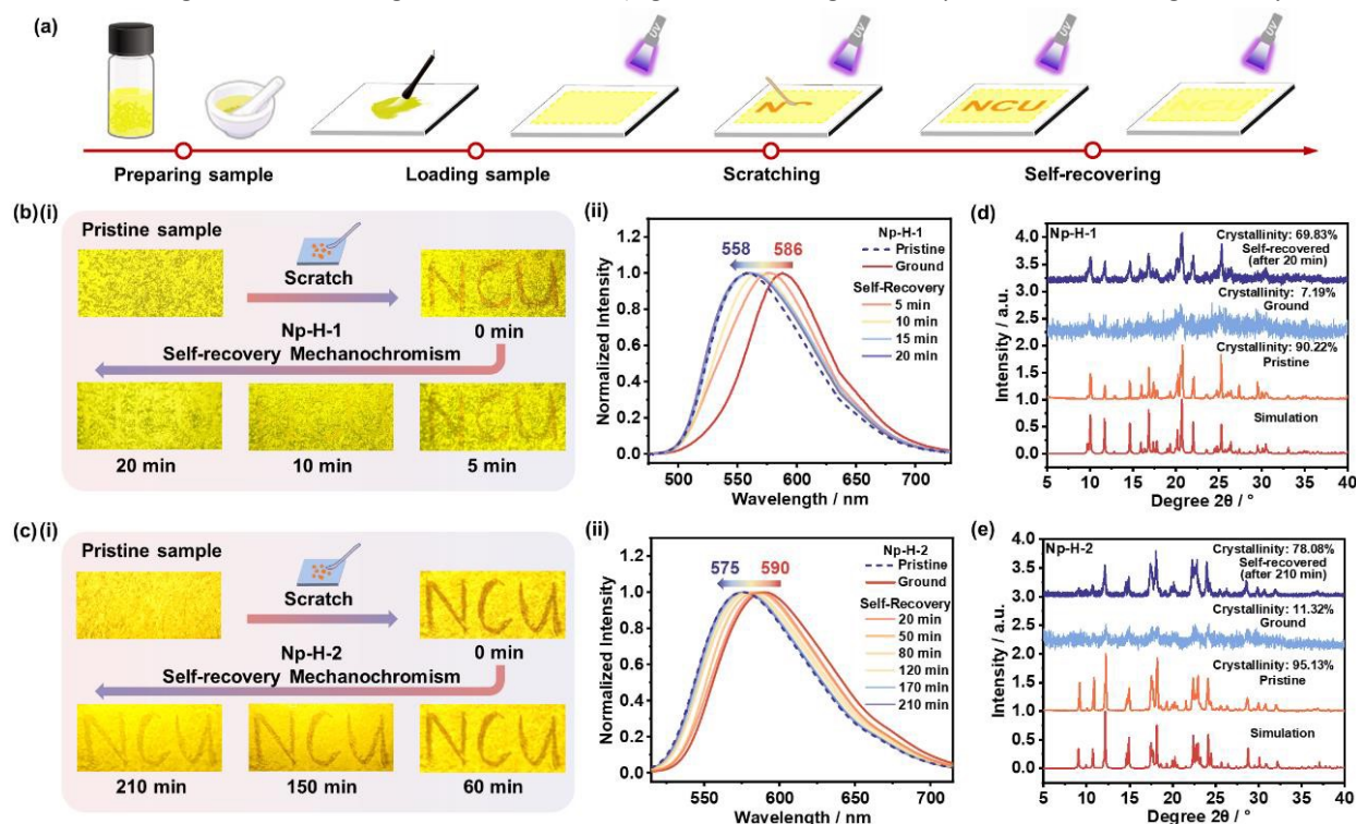
Fig. 3 (a) Schematic representation of the self-recovering MCF process based on the representative compound Np-H-1. (b-c) (i) Fluorescence photographs of pristine and treated Np-H microcrystals under UV light illumination (365 nm). (ii) Normalized PL spectra of pristine Np-H microcrystals (dotted line) during the grinding-recovering (solid line) process. PXRD patterns of pristine, ground and self-recovered (d) Np-H-1, (e) Np-H-2 microcrystals.
