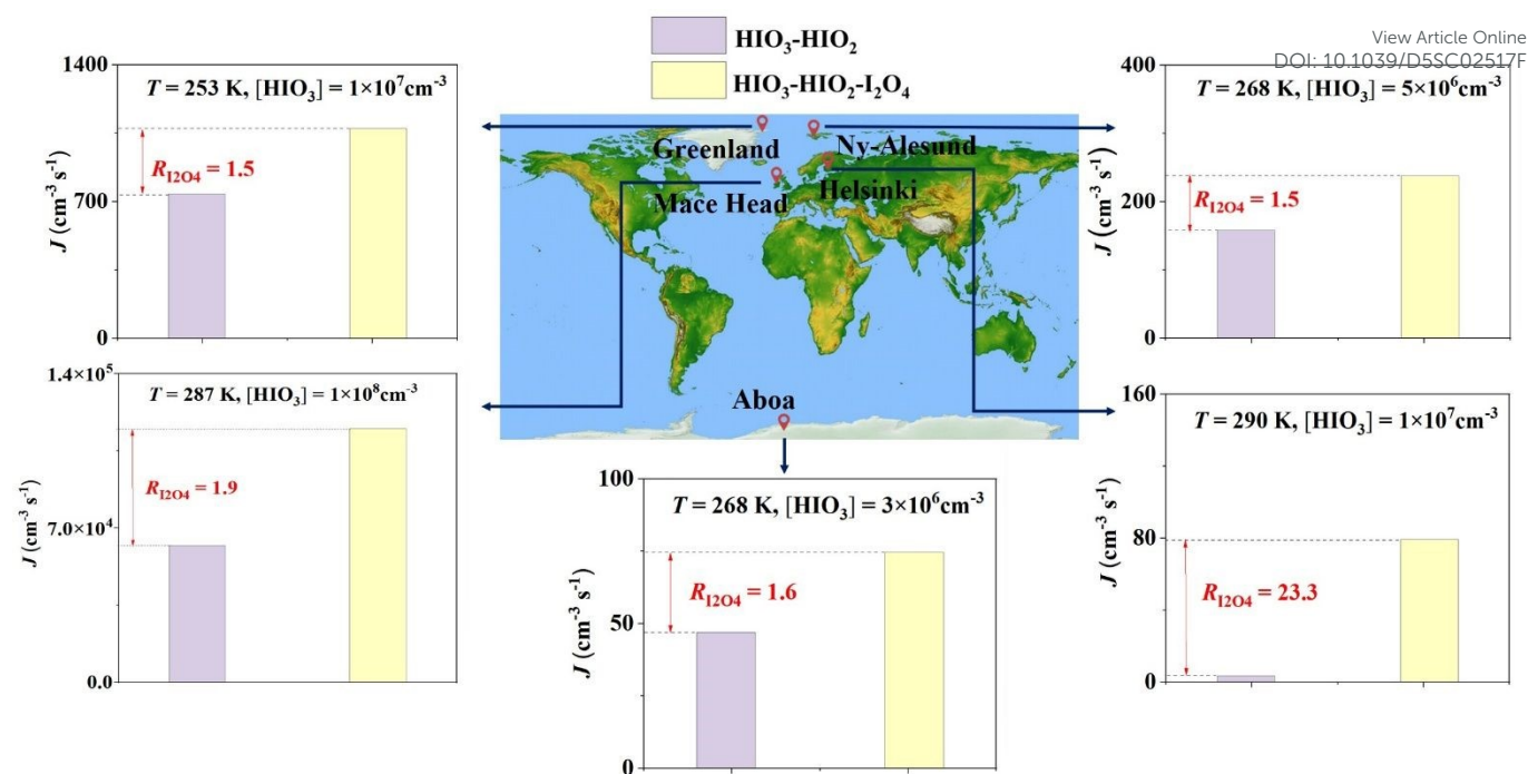
Figure 6. Cluster formation rate ( J ) ( \text{cm}^{-3} \text{s}^{-1} ) of the \text{HIO}_3\text{-HIO}_2\text{-I}_2\text{O}_4 and \text{HIO}_3\text{-HIO}_2 systems and the enhancement coefficient ( R_{12\text{O}4} ) in different areas with different temperatures ( T ) and [\text{HIO}_3] . The T and [\text{HIO}_3] in different areas were obtained from He et al. 38 The k_{\text{coag}} in Helsinki and Mace Head was set to 2 \times 10^{-3} \text{s}^{-1} , 55 and k_{\text{coag}} in Aboa, Greenland, and Ny-Ålesund was set to 1 \times 10^{-4} \text{s}^{-1} . 38
