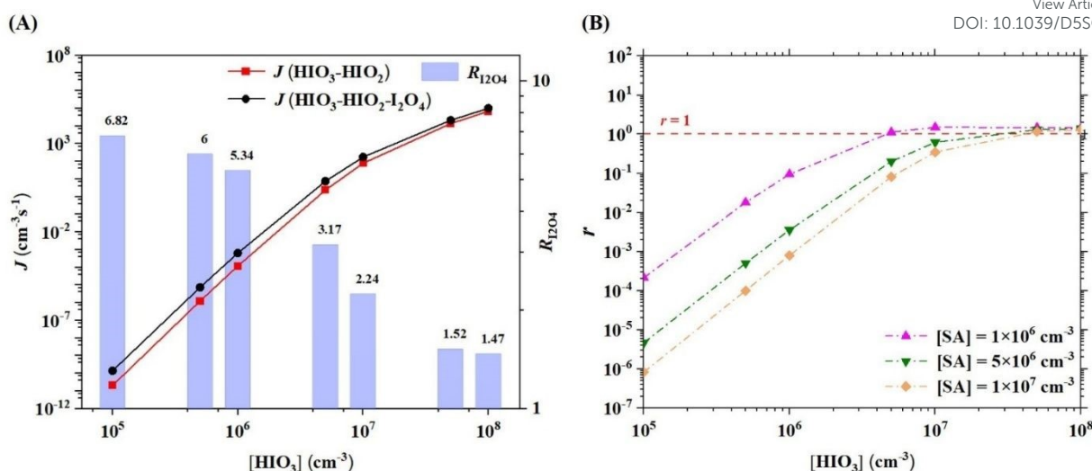
Figure 4. Cluster formation rates ( J ) ( \text{cm}^{-3} \text{s}^{-1} ) of the \text{HIO}_3\text{-HIO}_2 and \text{HIO}_3\text{-HIO}_2\text{-I}_2\text{O}_4 systems and enhancement coefficient ( R_{\text{I}_2\text{O}_4} ) (the ratio of the J value of the \text{HIO}_3\text{-HIO}_2\text{-I}_2\text{O}_4 system relative to that of the \text{HIO}_3\text{-HIO}_2 system) (A) and comparison coefficient ( r ) (the ratio of the J value of the \text{HIO}_3\text{-HIO}_2\text{-I}_2\text{O}_4 system relative to that of the \text{SA-HIO}_3\text{-HIO}_2 system) (B) as a function of precursor concentration at 278.15 K, 1 atm and k_{\text{coag}} = 0.002 \text{ s}^{-1} .
