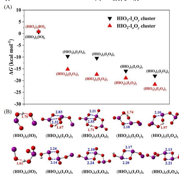
Figure 1. Formation free energy ( \Delta G ) (A) and global minimum configurations (B) of \text{I}_x\text{O}_y\text{-HIO}_{2-3} dimers at the DLPNO-CCSD(T)/aug-cc-pVTZ(-PP)//M06-2X/aug-cc-pVTZ(-PP) level of theory at 298.15 K. The red balls represent oxygen atoms, purple ones are for iodine atoms, and white ones are for hydrogen atoms. The red dashed lines in the configurations represent hydrogen bonds (HBs), and the blue dashed lines represent XBs. The red and blue numbers indicate the bond lengths of HBs and XBs, respectively. The bond lengths are given in Å.
