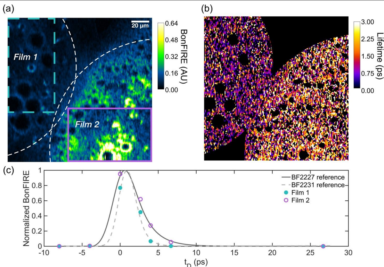
Figure 5. Vibrational lifetime multiplex imaging. (a) BonFIRE image of overlapping BF2227 and BF2231 films at \omega_{IR} = 2229\text{ cm}^{-1} and \omega_{probe} = 11,930\text{ cm}^{-1} (white dashed lines mark the approximate edges of the films). (b) Vibrational lifetime image of overlapping BF2227 and BF2231 films (low-intensity regions are masked). Film 2 exhibits systematically larger vibrational lifetimes. (c) Overlay of reference temporal profiles of BF2227 (dark grey solid curve) and BF2231 (light grey dashed curve) and temporal profiles of Films 1 (turquoise dots) and 2 (purple circles) in the regions of interest marked in panel (a). The temporal profiles of Films 1 and 2 align with the solution spectra of BF2231 and BF2227, respectively.
