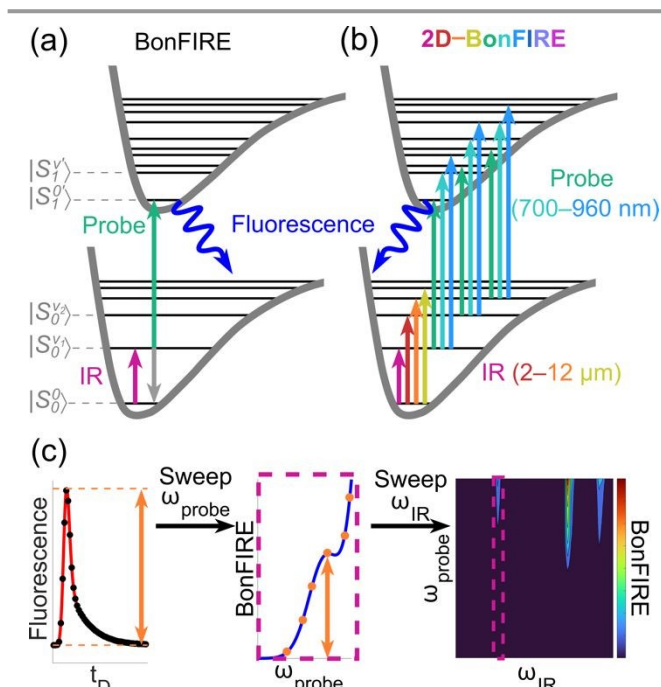
Figure 1. Overview of 2D-BonFIRE. (a) Principle of BonFIRE, comprising two narrowband excitations. Vibronic states are labelled |S_n^v\rangle , where n describes the electronic state and v describes the vibrational state. Vibrational states are labelled with an apostrophe (') in the S_1 manifold. (b) Principle of 2D-BonFIRE, where narrowband pulses are tuned across broad frequency ranges. (c) Picosecond-scanning methodology of 2D-BonFIRE. 2D spectra are constructed from a series of 1D sweeps, where BonFIRE intensity is measured by the peak height in a sweep of the time delay ( t_D ) between the IR and probe pulses.
