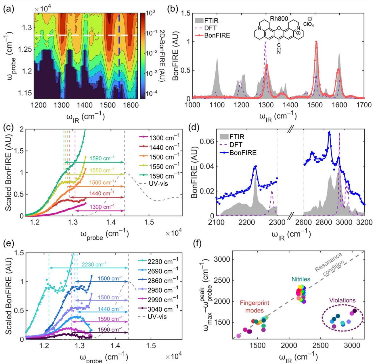
Figure 2. 2D-BonFIRE frequency-domain spectroscopy. (a) 2D-BonFIRE fingerprint spectrum of Rh800 at 100 \mu\text{M} in DMSO- d_6 . (b) 2D-BonFIRE intensity as a function of \omega_{IR} at \omega_{probe} = 12,820 \text{ cm}^{-1} (Rh800 structure inset). 2D-BonFIRE aligns well with the FTIR spectrum (grey, 100 mM in DMSO) and the predicted IR absorption by DFT (purple; scaled by 0.975). We note that the absence of certain peaks in BonFIRE compared to FTIR is due to solvent interference from DMSO and dye aggregation due to the high concentrations needed for FTIR, as we have discussed previously. 38, 40 (c) Relative 2D-BonFIRE intensity as a function of \omega_{probe} for Rh800 at \omega_{IR} = 1300 (pink), 1440 (red), 1500 (orange), 1550 (yellow) and 1590 (green) \text{cm}^{-1} . Because these signals vary over orders of magnitude, the spectra have been scaled to facilitate a visual comparison. Vertical dashed line positions are defined relative to the UV-vis absorption maximum. (d) 2D-BonFIRE of Rh800 in the nitrile and CH-stretching regions at \omega_{probe} = 12,120 \text{ cm}^{-1} . Due to strong anharmonicity, the frequency of the nitrile-stretch is over-estimated in harmonic DFT. The CH-stretching absorptions predicted by DFT (purple; scaled by 0.975) disagree with the FTIR (grey) and 2D-BonFIRE (blue) spectra. (e) Scaled 2D-BonFIRE \omega_{probe} -dependence of Rh800 for the high-frequency
