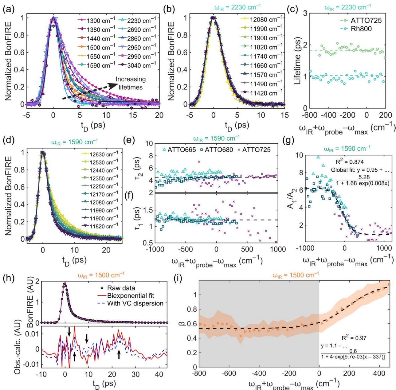
Figure 3. 2D-BonFIRE time-domain spectroscopy. (a) Representative normalized time-domain spectra of major modes of Rh800. (b) Normalized time-domain spectra of the nitrile-stretch of ATTO725 at \omega_{\text{IR}} = 2230 \text{ cm}^{-1} and varying \omega_{\text{probe}} . (c) \omega_{\text{probe}} -dependence of the nitrile lifetimes of Rh800 (blue) and ATTO725 (green) at \omega_{\text{IR}} = 2230 \text{ cm}^{-1} . The nitrile lifetimes are constant, characteristic of a local oscillator mode. (d) Normalized time-domain spectra of ATTO725 at \omega_{\text{IR}} = 1590 \text{ cm}^{-1} and varying \omega_{\text{probe}} . (e-g) \omega_{\text{probe}} -dependence of (e) \tau_2 (dashed line at 4.5 ps), (f) \tau_1 (dashed line at 1.2 ps), and (g) A_1/A_2 (trendline is a sigmoidal global fit) for ATTO665, ATTO680, and ATTO725 at \omega_{\text{IR}} = 1590 \text{ cm}^{-1} . (h) Rh800 time-domain BonFIRE at \omega_{\text{IR}} = 1500 \text{ cm}^{-1} and \omega_{\text{probe}} = 12,950 \text{ cm}^{-1} . Judging by the oscillating residuals of the fit (Obs.-calc.; bottom panel), the observed decay is not described by a pure biexponential (red solid line; residual oscillations highlighted by black arrows). Modelling VC rate dispersion with a KWW function (blue dashed line) yields improved fitting. (i) \beta as a function of probing energy for \omega_{\text{IR}} = 1500 \text{ cm}^{-1} (trendline is a sigmoidal fit). \beta transitions from its initial value of \sim 0.5 to \sim 1 as \omega_{\text{probe}} increases.
