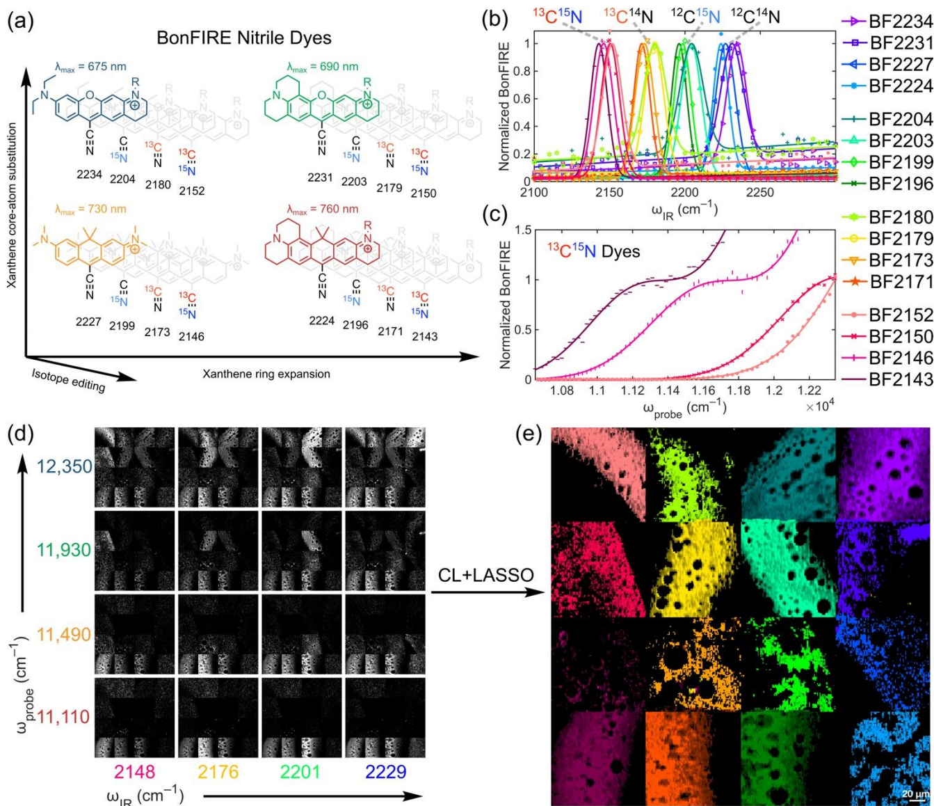
Figure 4. 16-colour chemical imaging by 2D-BonFIRE. (a) Structures of BonFIRE nitrile dyes for super-multiplex imaging ( \text{R} = (\text{CH}_2)_3\text{CO}_2^- ). Dye scaffolds are colour-coded by electronic absorption and labelled with their absorption maxima, 71 and individual dyes are labelled by their nitrile IR frequency in \text{cm}^{-1} . (b) Lifetime-weighted IR reference spectra for BF dyes. (c) Probe reference spectra for ^{13}\text{C}^{15}\text{N} BF dyes (other isotopologues shown in Fig. S16). (d) Stitched BonFIRE images of labelled PS films acquired with varying \omega_{\text{IR}} and \omega_{\text{probe}} (contrast scaled for each \omega_{\text{probe}} for visual comparison). (e) Unmixed 16-colour BonFIRE image of labelled PS films by adding conditional logic to the least absolute shrinkage and selection operator (CL+LASSO). Unmixed component images are provided for reference in Fig. S18.
