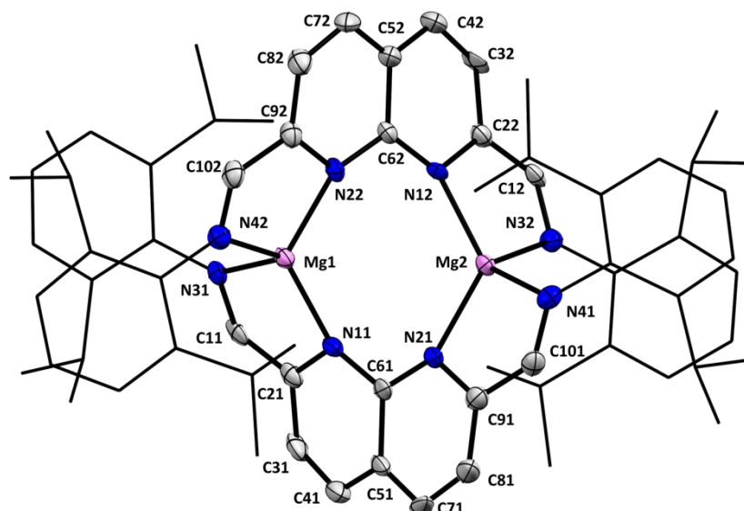
Figure 1: Displacement ellipsoid plot of 1 at 50% probability. Hydrogen atoms and minor disorder components are omitted for clarity. The dipp substituents are depicted as wireframe for clarity.
