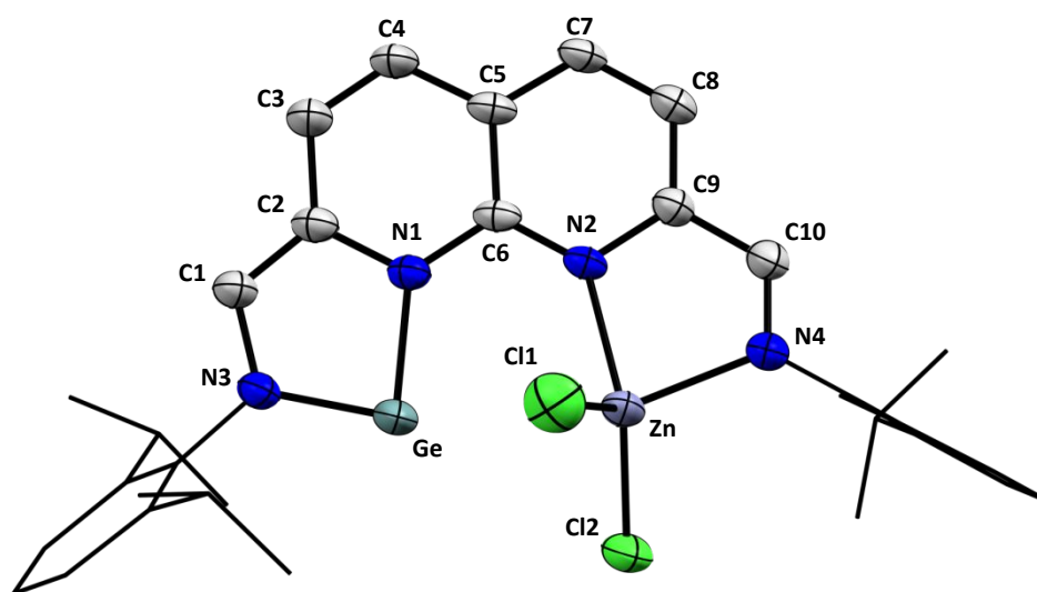
Figure 2: Displacement ellipsoid plot of 3 at 50% probability. Co-crystallised 1,4-dioxane molecules, hydrogen atoms and disordered components are omitted for clarity. The dipp substituents are depicted as wireframe for clarity.
