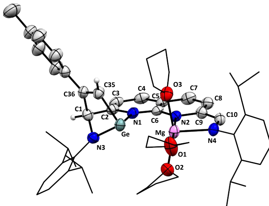
Figure 4: Displacement ellipsoid plot of 5 at 50% probability. Hydrogen atoms and minor disorder components are omitted for clarity. The dipp substituents and the carbon backbones of the THF molecules are depicted as wireframe for clarity.
