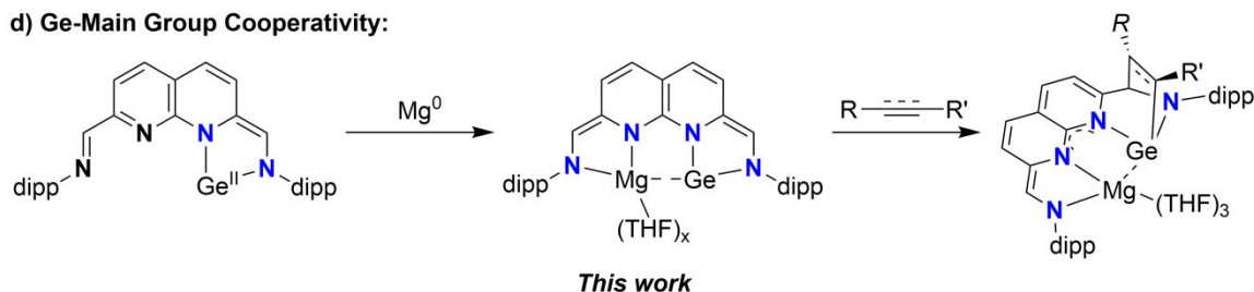
Scheme 1: a-c) The various types of reactivity modes described for germylenes and d) the Ge-Main group cooperativity described in this work.
