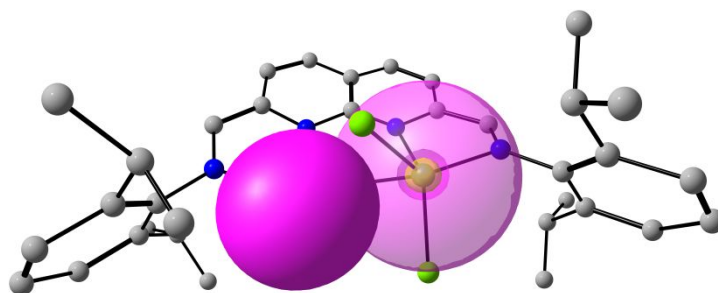
Figure 3: Overlap of the Ge-based lone pair donor NBO (filled) with the Zn-based acceptor NBO (translucent) of 3b , where the Ge–Zn distance was kept frozen to the value obtained from the solid-state structure. 2 nd Order perturbation analysis revealed that the Ge–Zn interactions are weak.
