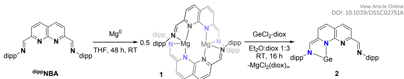
Scheme 2: Syntheses of 1 and 2 starting from the redox-active \text{dipPNBA} ligand.
