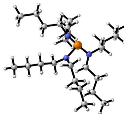
B Ligand conformer
