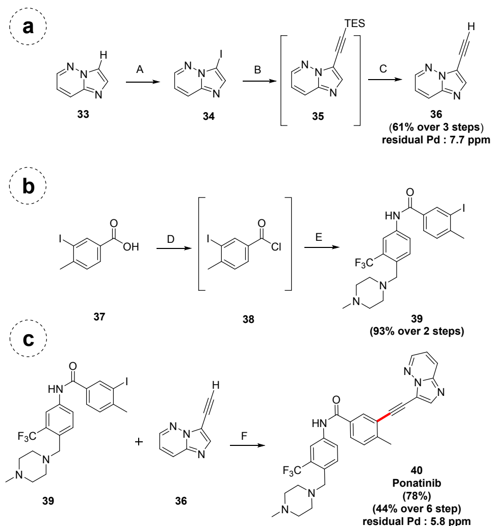
Scheme 2. Multi-step synthesis of ponatinib ; reaction conditions: a) Step A: 33 (1 equiv), NIS (3 equiv), I 2 (5 equiv), ACN (1.8 M), 80 °C, Ar, 30 min. Step B: 34 (1 equiv), TES-acetylene (1.5 equiv), Pd(OAc) 2 (0.5 mol %), L4 (2 mol %), NEt 3 (3 equiv), 2 wt % SDS/H 2 O (0.5 M), CPME (20 v/v %), 70 °C, Ar, 16 h. Step C: 35 (1 equiv), TBAF (1 equiv), THF (0.02 M), 0 °C to rt, 16 h. b) Step D: 37 (1 equiv), (COCl) 2 (3 equiv), EtOAc (0.25 M), 0 °C to rt, 2 h. Step E: 38 (1 equiv), 4-[(4-methyl-1-piperazinyl)methyl]-3-(trifluoromethyl)aniline (1 equiv), EtOAc (0.18 M), NEt 3 (3 equiv), 0 °C to rt, 2 h. c) Step F: 39 (1 equiv), 36 (2 equiv), Pd(OAc) 2 (0.75 mol %), L4 (3 mol %), NEt 3 (3 equiv), 2 wt % SDS/H 2 O (0.5 M), CPME (20 v/v %), 70 °C, Ar, 16 h.
