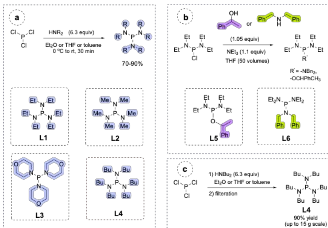
Scheme 1. Synthesis of aminophosphine ligands based on \text{PCl}_3
