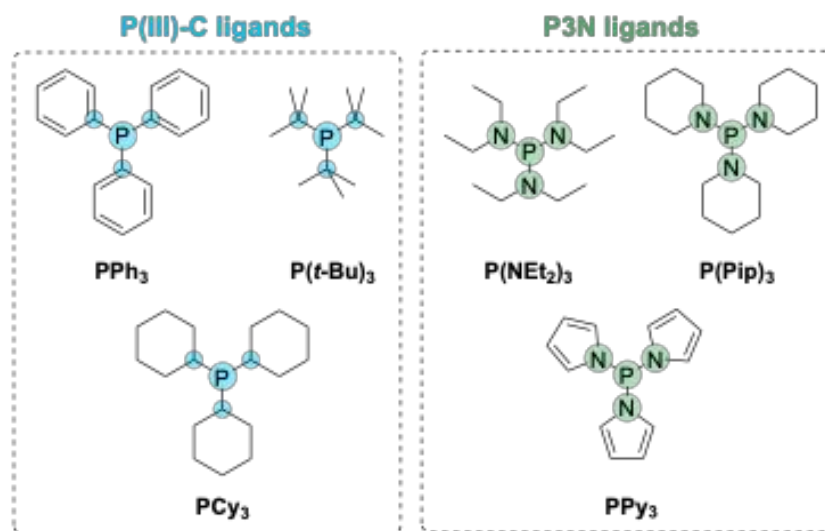
Figure 3. Representative examples of P-C and P-N ligand frameworks
