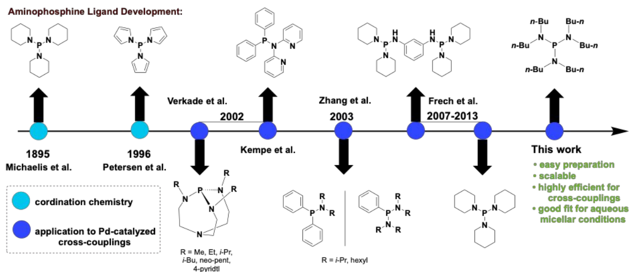
Figure 4. Evolution of aminophosphines as ligands.
