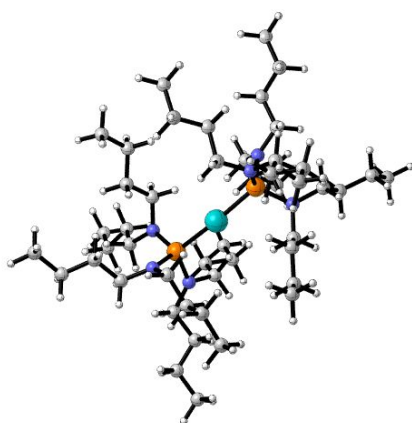
PdB 2 Two P3N ligands on Pd
