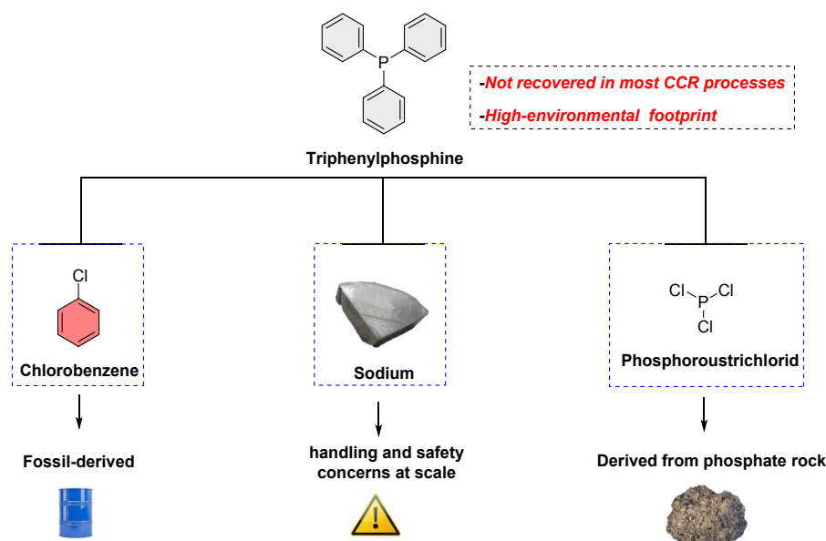
Figure 2. Conventional synthetic and sustainability issues involving triphenylphosphine
