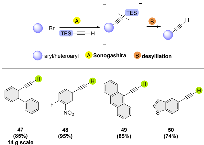
Scheme 4. Synthetic approach to terminal alkynes using L4 as the ligand; reaction conditions: Step A: aryl bromide (1 equiv), TES acetylene (1.2 equiv), \text{Pd}(\text{OAc})_2 (0.5 mol %), L4 (2 mol %), \text{NEt}_3 (3 equiv), 2 wt % SDS/ \text{H}_2\text{O} (0.5 M), CPME (20 v/v %), 70 °C, Ar, 16 h. Step B: TBAF (1 M in THF, 1.5 equiv), DCM (0.1 M), 0 °C to rt, 2 h.
