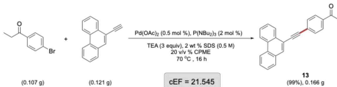
Scheme 5. Complete E-Factor for the preparation of 13
