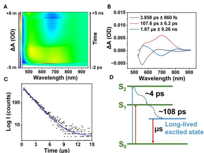
Figure 4. (A) Femtosecond transient absorption spectrum of 3d excited at 340 nm. (B) Three lifetime components simulated from global analysis that model the overall transient absorption spectrum. (C) Emission (775 nm) decay trace and fitting to a mono exponential decay of 3d . (D) Jablonski diagram of electronic excitation and excited state dynamics involved in the relaxation of 3d .
