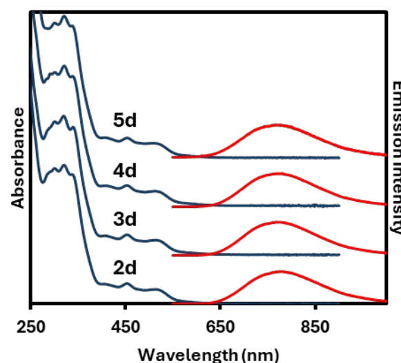
Figure 3. UV-Vis absorption spectra of clusters 2d , 3d , 4d , and 5d (blue) and their respective emission spectra excited at 453 nm (red). All spectra were taken in EtOH except for 5d which was taken in MeOH due to solubility issue.
