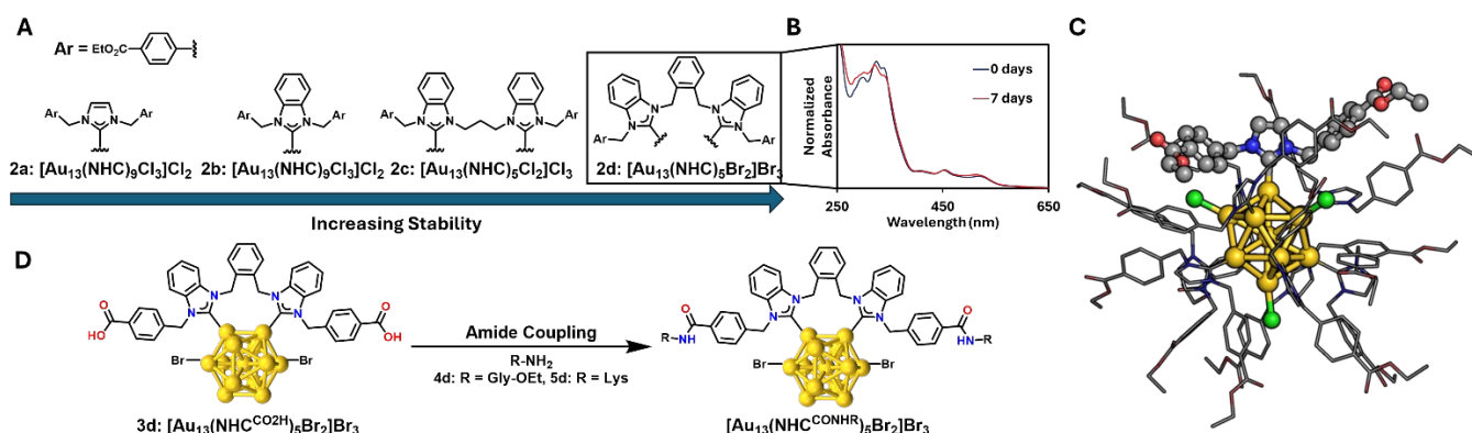
Figure 1. (A) Ligand dependent stability trends of -CO 2 Et functionalized Au 13 clusters ( 2a-d ). (B) Absorption spectra of 2d taken before and after heating at 90 °C for 4 days in 1:1 EtOH:H 2 O with 30 eq. KOH followed by 3 days in H 2 O with 30 eq. KOH, with absorbances normalized at 453 nm. (C) Coordination structure of 2a[PF 6 ] 2 , only one NHC ligand is highlighted for clarity (Grey = Carbon; Yellow = Gold; Red = Oxygen; Blue = Nitrogen; Green = Chlorine). (D) Amide coupling procedure for bioconjugation of amino acids to 3d .
