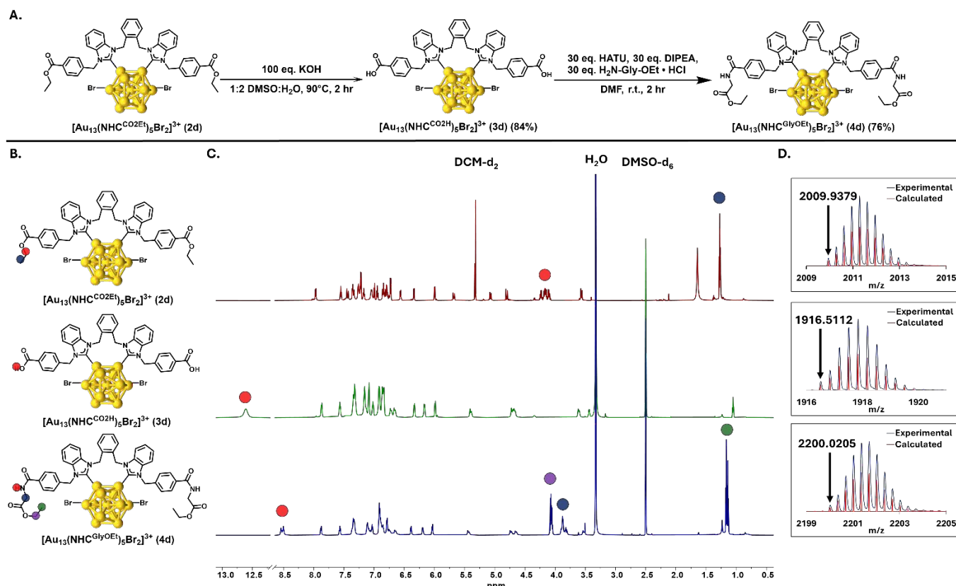
Figure 2. (A) Synthesis of 3d and 4d . (B) Structures of 2d , 3d , and 4d , highlighting key wingtip protons observable in 1 H NMR experiments. (C) 1 H NMR spectra of 2d in DCM-d 2 , and 3d and 4d in DMSO-d 6 depicting key signals on the wingtip groups. (D) ESI-MS spectra showing the experimental (blue) and calculated (red) isotope patterns of 2d , 3d , and 4d .
