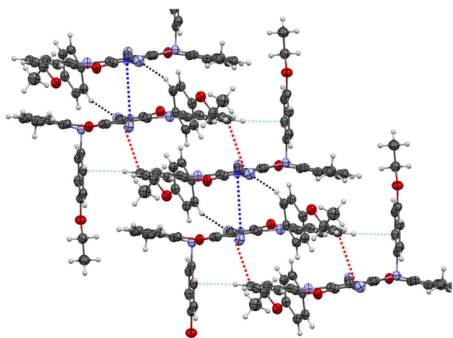
Fig. 4 Excerpt of the packing diagram depicting C–H \cdots\pi , \pi\cdots\pi and C–H \cdots N interactions between the Y2 molecules. Displacement ellipsoids are displayed at 50% probability levels. Non-covalent intermolecular interactions: 3.383 Å (blue); 3.335 Å (red); 2.558 Å (black); 2.594 Å (light green).
