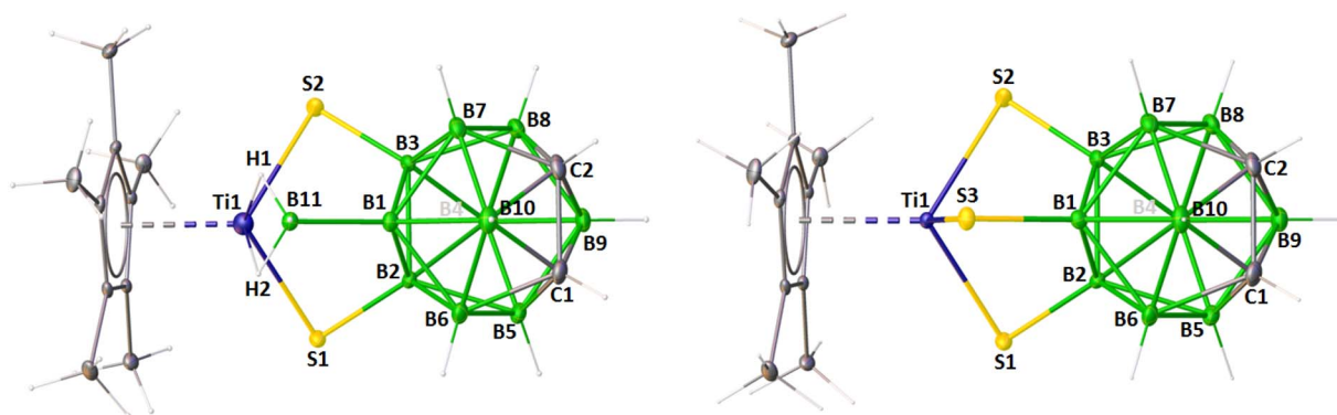
Fig. 5 Molecular structure and labelling diagram of 3 (left) and 4a (right). Selected bond lengths ( \text{\AA} ) and bond angles ( ^\circ ): 3 : Ti1–S1 2.3321(9) , Ti1–S2 2.3214(9) , Ti1⋯B11 2.259(4) , Ti1–H1 2.00(3) , Ti–H2 1.93(3) , B11–H1 0.90(3) , B11–H2 1.03(4) , B1–B11 1.750(5) , B2–S1 1.851(4) , C1–C2 1.626(6) , Ti1–S1–B2 81.17(11) , B2–B1–B11 121.9(3) . 4a : Ti1–S1 2.3095(12) , Ti1–S3 2.3231(12) , B1–S3 1.849(5) , B1–B2 1.829(5) , C1–C2 1.635(7) , C1–B10 1.713(7) , Ti1–S1–B2 80.72(14) .
