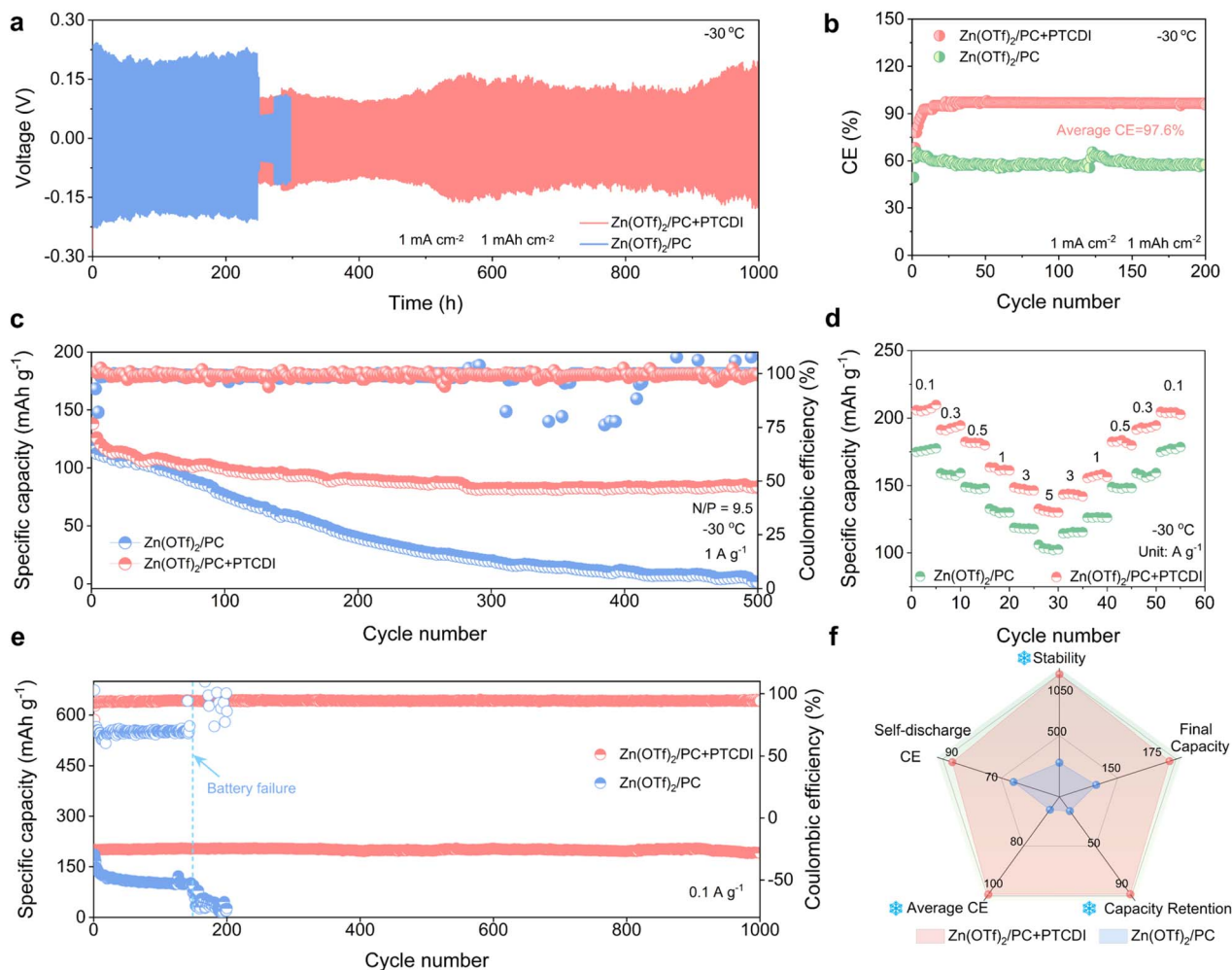
Fig. 5 Electrochemical performance of full cells and anode free \text{Cu}||\text{ZnMn}_2\text{O}_4 batteries. (a) Voltage profiles of Zn symmetric cells assembled with \text{Zn}(\text{OTf})_2/\text{PC} + \text{PTCDI} electrolytes at -30\text{ }^{\circ}\text{C} . (b) The CE of \text{Zn}||\text{Ti} cells in \text{Zn}(\text{OTf})_2/\text{PC} electrolytes with/without PTCDI at -30\text{ }^{\circ}\text{C} . (c) Long cycling stability performance of the \text{Zn}||\text{MnO}_2 full cell in \text{Zn}(\text{OTf})_2/\text{PC} and \text{Zn}(\text{OTf})_2/\text{PC} + \text{PTCDI} electrolytes at -30\text{ }^{\circ}\text{C} . (d) Rate performance of the \text{Zn}||\text{MnO}_2 full cell in \text{Zn}(\text{OTf})_2/\text{PC} and \text{Zn}(\text{OTf})_2/\text{PC} + \text{PTCDI} electrolytes at -30\text{ }^{\circ}\text{C} . (e) Cycling performance of anode-free \text{Cu}||\text{ZnMn}_2\text{O}_4 batteries. (f) Performance comparison of \text{Zn}||\text{MnO}_2 cells in \text{Zn}(\text{OTf})_2/\text{PC} and \text{Zn}(\text{OTf})_2/\text{PC} + \text{PTCDI} electrolytes.
