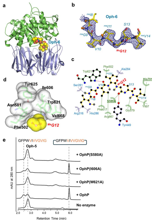
Fig. 7 Structure of the P1 recognition site of OphP. (a) OphP S580A complex with peptide substrate Oph-6 is shown in spheres (the color scheme is as in Fig. 6a). (b) The \sigma_A -weighted 2Fo-DFc map (contoured at 1 \sigma ) for Oph-6 (c) LigPlot diagram 45 showing interactions of Oph-6 with OphP. (d) Surfaces of Me Gly12 and its surrounding hydrophobic pocket in the Oph-6 complex. The pocket is composed of Tyr625, Trp621, Val668, Phe502, Asn581 and Ile606. (e) HPLC analysis of assays using 7-methylated Oph-5 as substrate for OphP and its variants. The control reaction without OphP shows the absorption profile of the starting material. While the W621A mutation abolished macrocyclization, I606A showed an activity comparable to wildtype OphP. The reactions were performed at 25 °C in buffer containing 50 mM HEPES pH 7.0, 100 mM NaCl and 5 mM DTT at a concentration of 20 \mu M enzymes and 200 \mu M Oph-5.
