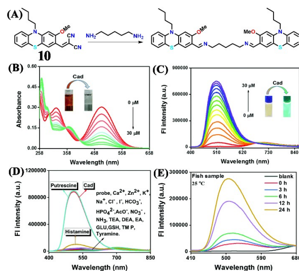
Fig. 11. (A) The structure of sensor 10 and its reaction with cadaverine. The observed changes in (B) absorption and (C) fluorescence emission spectra of 10 upon the addition of cadaverine in increased concentrations (Inset: corresponding visual colour changes). (D) The fluorescence spectra of 10 in the presence of cadaverine and other competing analytes. (E) The fluorescence spectra of 10 after mixing cadaverine extracts from fish samples exposed at 25 °C at different times. Reproduced with permission from ref. 48. Copyright 2022, Royal Society of Chemistry.
