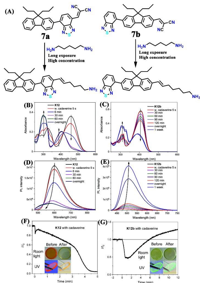
Fig. 8. (A) Sensors 7a and 7b and their aza-Michael addition reaction with cadaverine at high concentration. The change in (B) electronic absorption and (C) fluorescence emission spectra of 7a (labeled as K12) were recorded at different exposure intervals after cadaverine addition. The change in (D) electronic absorption and (E) fluorescence emission spectra of 7b (labeled as K12b) were recorded at different exposure intervals after cadaverine addition. The change in photoluminescence peak intensity of (F) 7a (labeled as K12) and (G) 7b (labeled as K12) loaded thin films after exposure to cadaverine vapours at different exposure times (Inset: corresponding photographs imaged in daylight and under UV light). Reproduced with permission from ref. 45. Copyright 2020, Royal Society of Chemistry.
