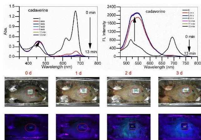
Fig. 5. The time-dependent UV-visible absorption (top left) and fluorescence emission (top right) spectra for sensor 4a in the presence of cadaverine (40 equiv.) in dioxane. The fish spoilage monitoring using 4a -loaded filter paper. Reproduced with permission from ref. 41. Copyright 2020, Elsevier.
