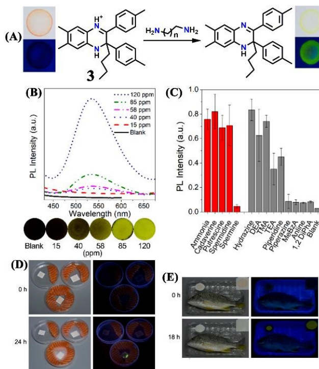
Fig. 3. (A) The conversion of the protonated form of sensor 3 to its deprotonated form after exposure to BAs (Inset: the original red colour of 3 changed to bright yellow after exposure to BAs). (B) The photoluminescence spectra of 3 loaded filter paper strips exposed to different concentrations of ammonia vapours and the corresponding photographs were imaged under UV light irradiation. (C) The turn-on photoluminescence responses of 3 loaded filter paper strips after exposure to different amine vapours (red bar = BAs, grey bar = other amines). (D) The observed fluorescence emission enhancement for 3 (after 24h exposure) sealed with salmon sashimi. (E) Turn-on fluorescence responses were observed for 3 after 18h exposure in a sealed package of yellowfin seabream. Reproduced with permission from ref. 40. Copyright 2017, Wiley.
