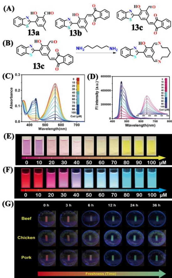
Fig. 14. (A) The structure of sensors 13a-c and (B) the proposed cadaverine sensing mechanism cyclic Schiff base formation. (C) The UV-visible absorption and (D) fluorescence emission spectra of 13c at different concentrations of cadaverine and their corresponding visual colour changes were imaged under (E) daylight and (F) UV light. (G) Photographs of 13c tags used for monitoring the freshness of beef, chicken, and pork stored at 25 °C recorded at different exposure times. Reproduced with permission from ref. 51. Copyright 2024, Elsevier.
