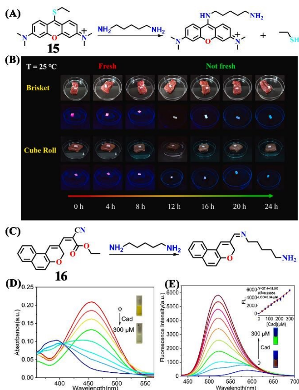
Fig. 16. (A) The proposed mechanism of cadaverine sensing by 15 and (B) 15 loaded fluorescent paper was used to monitor the freshness of beef at 25 °C and at different exposure times. (C) The structure of sensor 16 and its reaction with cadaverine resulted in Schiff base formation. The observed changes in (D) UV-visible absorption and (E) fluorescence emission spectra of 16 upon increased addition of cadaverine (Inset: the photographs of colour changes observed before and after the mixing of cadaverine). Reproduced with permission from ref. 53 and 54. Copyright 2024, Elsevier.
