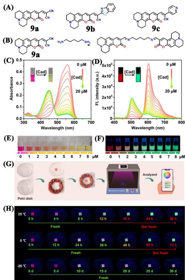
Fig. 10. (A) The structure of sensors 9a-c and (B) mechanism of cadaverine sensing by sensor 9a . The changes in (C) UV-visible absorption and (D) fluorescence emission for 9a upon the gradual mixing of cadaverine (Inset: corresponding colour changes). The visual colour changes were seen for sensor 9a in the presence of cadaverine at different concentrations, imaged (E) in room light and (F) under UV-light irradiation. (G) The schematic representation of the procedure used for monitoring the beef freshness. (H) The fluorescence images of 9a -loaded test strips sealed with beef were imaged at different temperatures at different times and under UV-light irradiation. Reproduced with permission from ref. 47. Copyright 2022, American Chemical Society.
