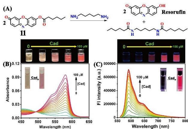
Fig. 12. (A) The structure of sensor 11 and its reaction with cadaverine yield red-emissive Resorufin dye. The changes in (B) absorption and (C) fluorescence emission spectra of 11 upon the addition of cadaverine in increased concentrations (Inset: corresponding visual colour changes). The above images correspond to colour changes for different concentrations of cadaverine. Reproduced with permission from ref. 49. Copyright 2023, Elsevier.
