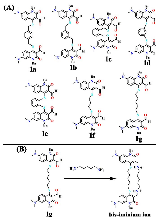
Fig. 1. (A) The structure of quinolone aldehyde-based sensors 1a–g and (B) the proposed reactivity-based sensing of cadaverine by sensor 1g .
