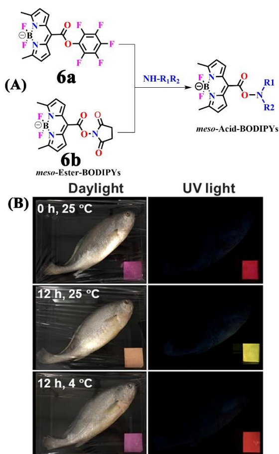
Fig. 7. (A) Sensors 6a and 6b and the proposed BA sensing mechanism through ester-to-amide conversion. (B) Monitoring white croaker fish freshness using 6a led filter paper imaged (in daylight and under UV light) at different time intervals and incubation temperatures. Reproduced with permission from ref. 44. Copyright 2020, American Chemical Society.
