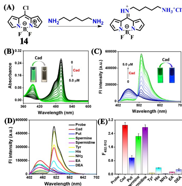
Fig. 15. (A) The structure of sensor 14 and its reaction with cadaverine yield a blue-emitting product. The ratiometric UV-visible absorption (B) and fluorescence emission (C) changes were observed for 14 after the gradual addition of cadaverine (Inset: the photographs of colour changes observed). (D) The differential fluorescence sensing properties of 14 for different amine analytes and (E) corresponding histogram. Reproduced with permission from ref. 52. Copyright 2023, Elsevier.
