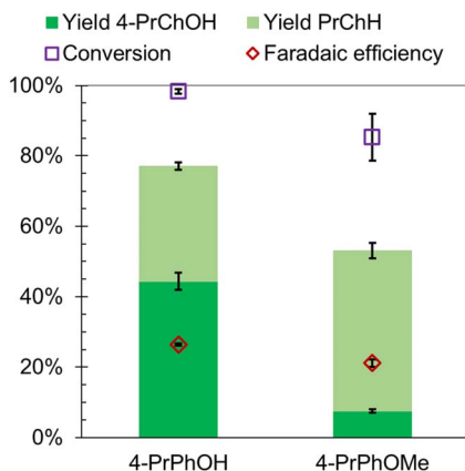
Fig. 5 ECH of 4-PrPhOMe and 4-PrPhOH. Product yields, substrate conversion and faradaic efficiency. Experimental conditions: current = 60 mA; (mol \text{e}^- )/(mol substrate) = 20 (4-PrPhOH and 4-PrPhOMe); temperature = 60 °C. Error bars represent standard errors.
