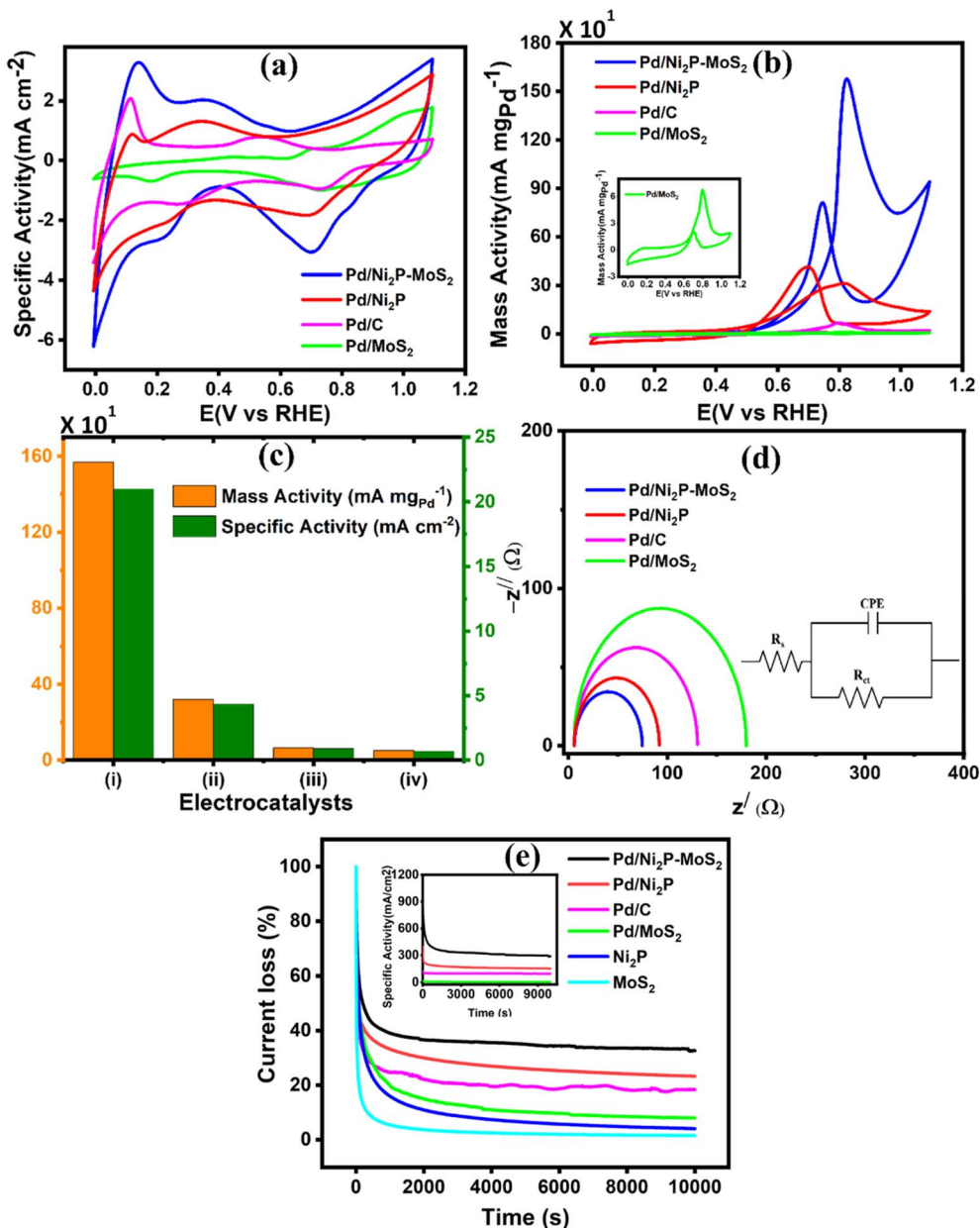
Fig. 5 (a) Cyclic voltammograms in 1 M KOH, (b) ethanol oxidation at a scan rate of 50 \text{ mV s}^{-1} , (c) the maximum mass activity and specific activity for (i) Pd/Ni 2 P–MoS 2 , (ii) Pd/Ni 2 P, (iii) Pd/C and (iv) Pd/MoS 2 , (d) Nyquist plots at 0.55 V in 1 M KOH + 0.5 M CH 3 CH 2 OH, and (e) chronoamperometric curves measured at 0.59 V vs. RHE).
