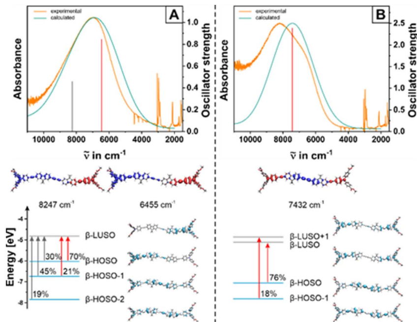
Fig. 6 Top: Comparison between experimental NIR spectra of 2^{\text{Me}+} (orange line in panel A) and 2^{\text{Me}2+} (green line in panel B) in 1,2- \text{CH}_2\text{Cl}_2 (0.1 M \text{NBu}_4^+ [ \text{BAR}^{\text{F}24} ] ^- as the supporting electrolyte) and TD-DFT calculated electronic spectra of model compound 2^{\text{Me}+} (panel A, turquoise line) and 2^{\text{Me}2+} (panel B, violet). Computed transitions are provided as red and grey vertical bars. Bottom: Contour diagrams of the acceptor and donor MOs involved in the NIR transitions together with their contributions to the respective transition and corresponding electron density difference maps (EDDMs). Blue color indicates electron density loss and red color an increase in electron density. Isosurface values for the MO plots are set as \pm 0.02 .
