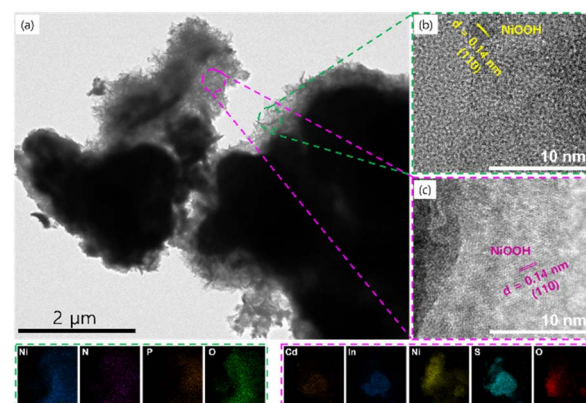
Fig. 6 (a) TEM image of the \text{NH}_4\text{NiPO}_4 \cdot \text{H}_2\text{O}/\text{CdIn}_2\text{S}_4/\text{Ni}_3\text{S}_2 heterostructure after the UOR process, highlighting the overall morphology and nanoscale features. (b and c) HRTEM images illustrating the formation of the NiOOH phase via surface reconstruction during UOR. The bottom panel displays TEM elemental mappings, confirming the uniform distribution of elements within the \text{NH}_4\text{NiPO}_4 \cdot \text{H}_2\text{O}/\text{CdIn}_2\text{S}_4/\text{Ni}_3\text{S}_2 heterostructure and validating the formation of NiOOH at the reconstructed regions.
