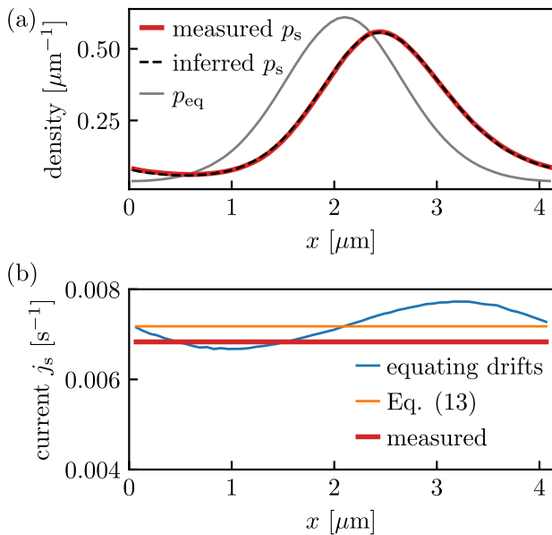
Fig. 4 (a) p_s(x) in Eq. (11) inferred from equilibrium (passive) experiments and using the value v_0 = 0.053 \mu\text{m/s} of the experimentally fixed velocity, where we deduced U(x)/k_B T up to a constant offset from \ln p_{\text{eq}} , where p_{\text{eq}} was estimated as a histogram of the equilibrium dynamics with 60 bins in [0, L) (setting a limited spatial resolution for the rest of the analysis). Note that for our experimental setting, U is technically known but involves a convolution with a Bessel function 75,76 and is prone to experimental inaccuracies. We thus prefer to infer U directly from the equilibrium data. The diffusion coefficient D = 0.04 \mu\text{m}^2/\text{s} was fitted from \text{var}(dx_\tau)/2d\tau averaged over [0, t] and over all trajectories, see Eq. (14). The equilibrium density p_{\text{eq}} is only shown for comparison and we stress that it, as expected, does not agree with p_s(x) . (b) Probability current inferred from the equilibrium data using the value v_0 = 0.053 \mu\text{m/s} of the experimentally prescribed velocity as described in Eq. (13) and below. The comparison to the measured value in the driven data, see Eq. (15), shows slight deviations.
