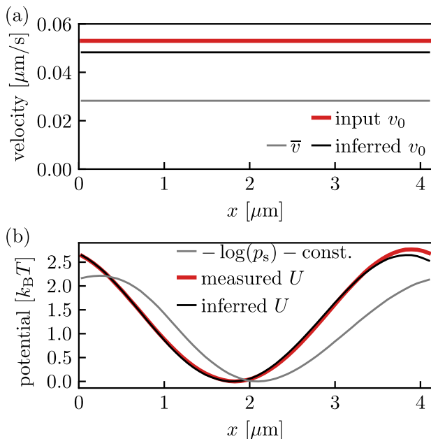
Fig. 5 (a) Inferred v_0 from driven experimental data compared to the desired input value v_0 . Though there are some statistical deviations in the values for v_0 (related to Fig. 4b), both obtained values for v_0 are well distinguishable from the mean velocity \bar{v} (grey line). (b) The potential U(x) inferred from the driven data via Eq. (17) (black line) matches the potential measured from the equilibrium data projected on one period [0, L] using U(x) = -\ln(p_{\text{eq}}(x)) - \text{const.} (red line) quite well. The barrier height (difference between minimum and maximum) is 2.76 k_B T in the red line and 2.65 k_B T in the black line, respectively. It deviates from -\log(p_s) (grey line) since the driven data set does not obey a Boltzmann density [see Eqs. (2) and (3)].
