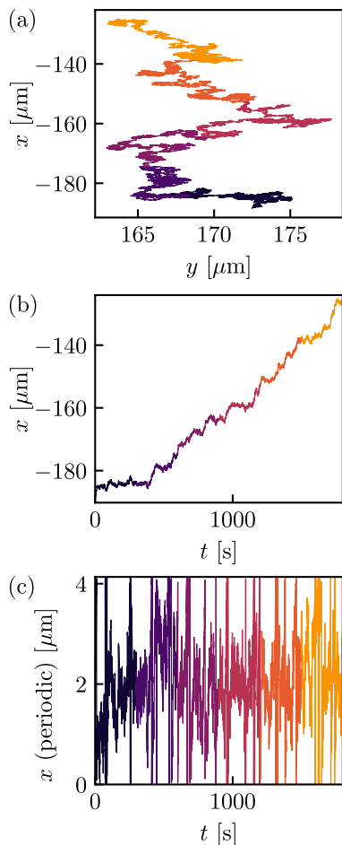
Fig. 3 Example of a trajectory that is driven by v_0 , see Eq. (2), (a), and corresponding projection onto the x -axis (b,c) where time runs from dark to bright. (c) The period is always chosen as L = 4.135 \mu\text{m} . The dataset comprises 1168 such trajectories.
