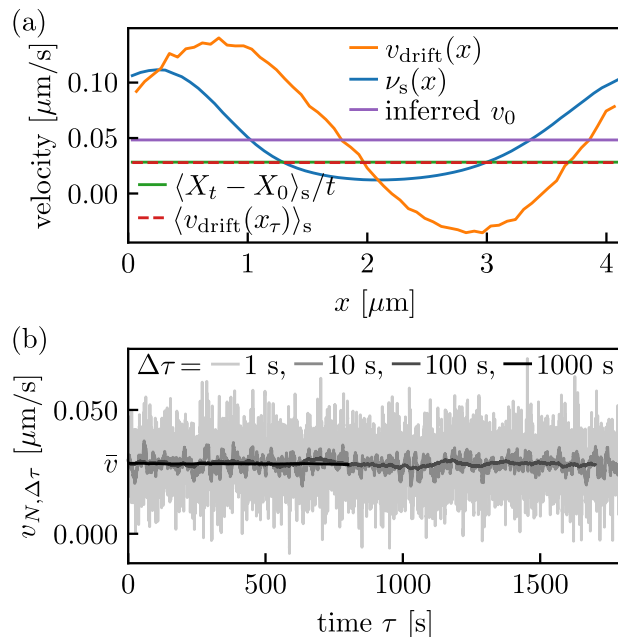
Fig. 6 (a) Different space-dependent and constant velocities in the NESS. See Eq. (9) for different representations of the mean velocity \bar{v} . In equilibrium, only v_{\text{drift}}(x) deviates from zero. Quantities denoted by averages over x_\tau are independent of \tau in the steady state and are here, for practical reasons to improve statistics, averaged over all \tau \in [0, t] . (b) While \bar{v} = \langle (x_{\tau+\Delta\tau} - x_\tau)_s \rangle / \Delta\tau for all \tau and \Delta\tau , see Eq. (9), the approximation \bar{v}_{N, \Delta\tau}(\tau) = \frac{1}{N} \sum_{i=1}^N (x_{\tau+\Delta\tau}^i - x_\tau^i) / \Delta\tau of this quantity over the finite number of trajectories N = 1168 as a function of \tau , as expected, exhibits large fluctuations for small \Delta\tau .
