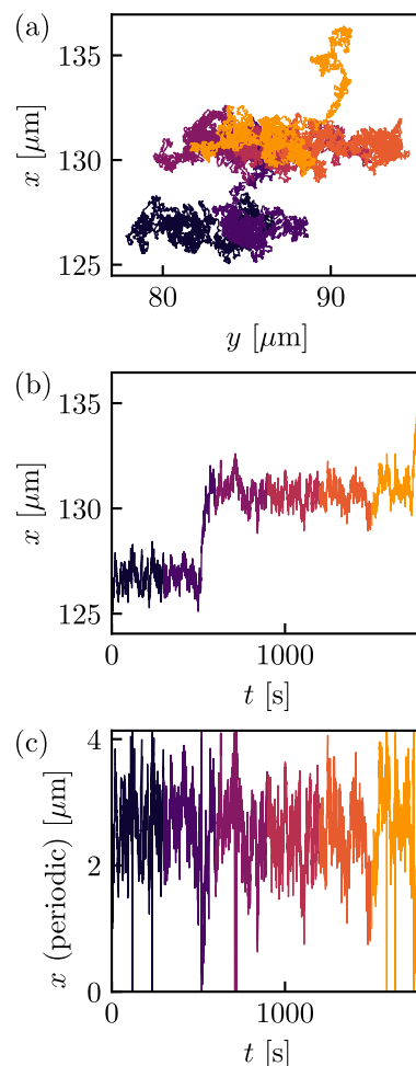
Fig. 2 Exemplary trajectory (a), and corresponding projection onto the x -axis (b,c) where time runs from dark to bright. (c) The period is always chosen as L = 4.135 \mu\text{m} . The dataset comprises 2448 such trajectories.
