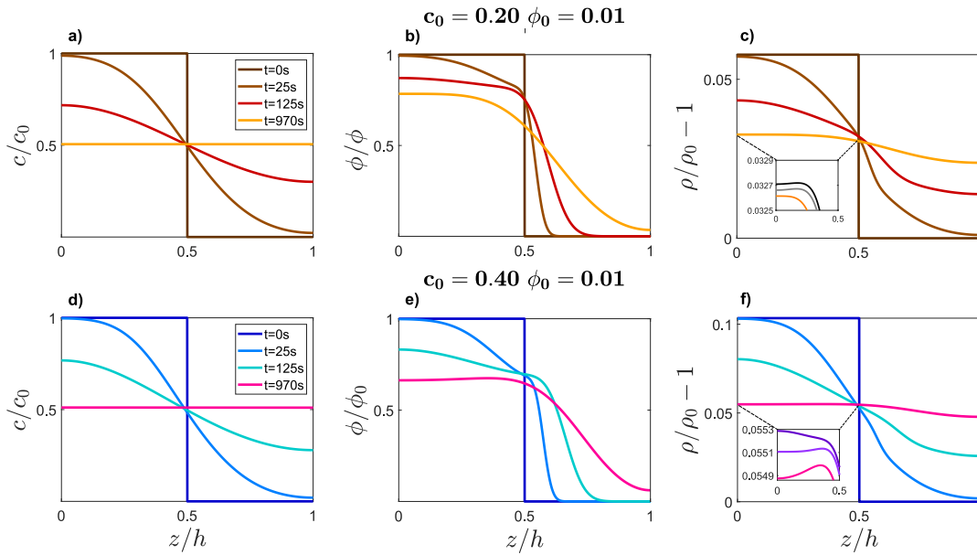
Fig. 4 Vertical profiles of glycerol mass fraction c/c_0 (a, d), colloid volume fraction \phi/\phi_0 (b, e) and density \rho/\rho_0 - 1 computed via Eq. (5) (c, f) at several times t (see legend). Profiles of c and \phi have been obtained by solving Eqs. (3) and 4 at fixed diffusiophoretic coupling \alpha = 125 , with initial conditions \phi_0 = 0.01 - c_0 = 0.2 (a, b, c) leading to a gravitationally stable configuration, and \phi_0 = 0.01 - c_0 = 0.4 (d, e, f), leading to an unstable configuration. The insets of panels (c) and (f) show the temporal evolution of the density profile in the region 0 \leq z/h \leq 0.5 , at times t = 633, 700, 970 s. In this interval of time, \rho starts displaying a critical local inversion of its slope in case c_0 = 0.4 (f) while no critical inversion occurs in the case c_0 = 0.2 (c).
