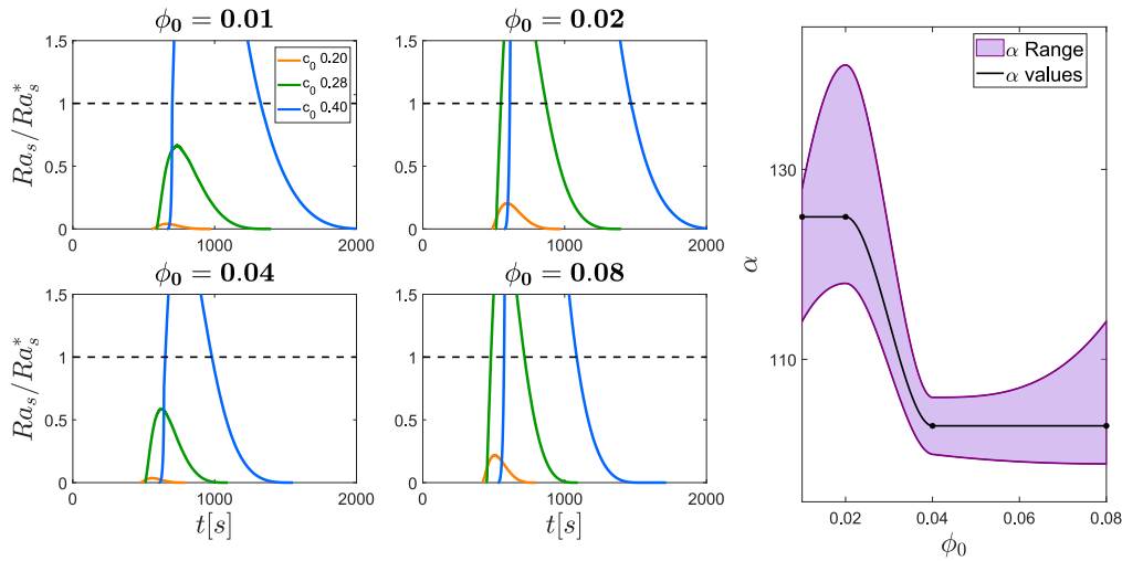
Fig. 5 a-d): Time evolution of the solutal Rayleigh number associated to the density profile of the base state (fig. 4) for the four volume fractions \phi_0 of colloid. When Ra_s exceeds the threshold value Ra_s^* (dashed line), the system becomes unstable against convection. In each panel, the Rayleigh number is calculated numerically at three glycerol concentrations c_0 (see legend in a). For each value of \phi_0 , we adjusted the value of the diffusiophoretic coefficient \alpha until the curves in panels a–d) reproduced the experimentally observed threshold of the instability (Fig. 3). Panel e) shows for each concentration of colloid \phi_0 the range of values of \alpha compatible with the range of values of c_0 observed experimentally where the threshold of the instability falls. The black points indicate the \alpha values used to compute Ra_s in panels a–d.
