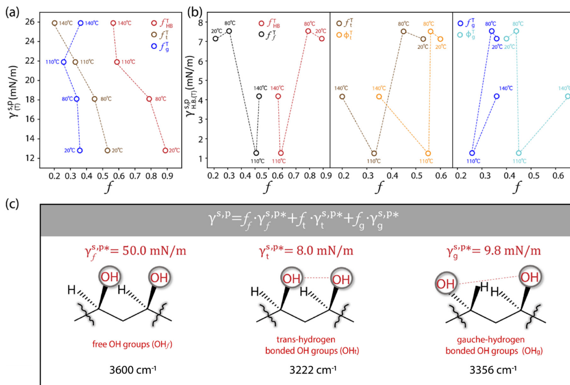
Fig. 3 (a) Plots of the \gamma_{\text{f}}^{\text{sp}} values of the as-prepared L_PVA 2 T thin films versus their f_{\text{HB}}^{\text{T}} , f_{\text{f}}^{\text{T}} , and f_{\text{g}}^{\text{T}} values. (b) Plots of the \gamma_{\text{HB(T)}}^{\text{sp}} values of the as-prepared L_PVA 2 T thin films versus their f_{\text{HB}}^{\text{T}} ( f_{\text{f}}^{\text{T}} ) (left panel), f_{\text{f}}^{\text{T}} ( \phi_{\text{f}}^{\text{T}} ) (middle panel), and f_{\text{g}}^{\text{T}} ( \phi_{\text{g}}^{\text{T}} ) values (right panel). (c) Schematic summarizing the molecular configurations of the surface OH f , OH g , and OH t groups, with the corresponding \gamma_{\text{f}}^{\text{sp}*} , \gamma_{\text{g}}^{\text{sp}*} , and \gamma_{\text{t}}^{\text{sp}*} values marked.
