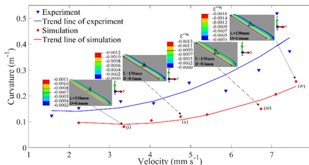
Fig. 10 Comparison between experiments 48,49 and simulations on the relation between heat-induced rolling velocity and curvature of a nylon fibre. The experimental and FE parameters: length 130 mm, diameter 0.6 mm, E = 100 MPa, \rho = 1.1 \times 10^3 kg m -3 .
