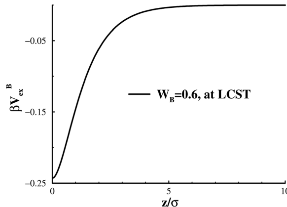
Fig. 2 An illustration of the surface adsorption potential, normalised by thermal energy, with W_B = 0.6 , at the LCST.
