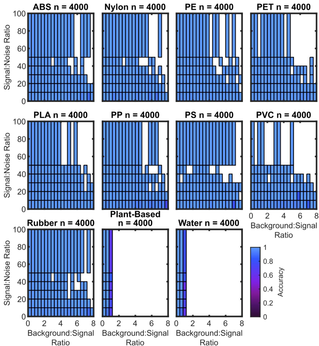
Figure 7 Two-dimensional histogram tiles showing the performance of the cubic SVM model trained on spectral data augmented with both noise and interferents for each plastic, with signal-to-noise ratios (SNR) on the y-axis, interferent-to-signal ratios (BSR) on the x-axis, and accuracy represented by the color scale. White regions have no data.
