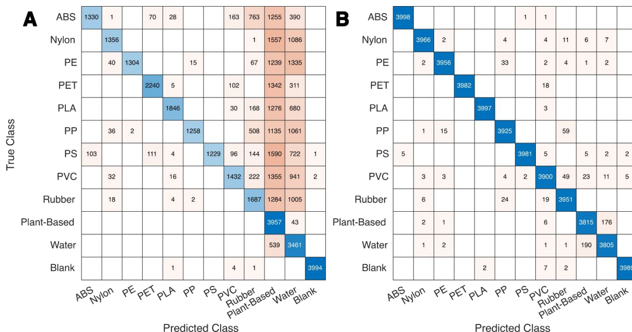
Figure 5 Confusion matrix of the cubic SVM model trained on spectral data augmented with noise only. (Interferents-free model) ( A ), and the cubic SVM model trained on spectral data augmented with both noise and interferents ( B ) tested on the synthetic testing set. The x-axis represents the predicted class, while the y-axis represents the true class. True positives are represented by the diagonal elements, indicating correctly classified samples. False positives are shown as off-diagonal elements in a column, where a sample is incorrectly classified into a certain class. False negatives are represented by off-diagonal elements in a row, where a sample is incorrectly excluded from its true class. The inclusion of interferent data during training in the model B significantly reduces misclassifications compared to the model A.
