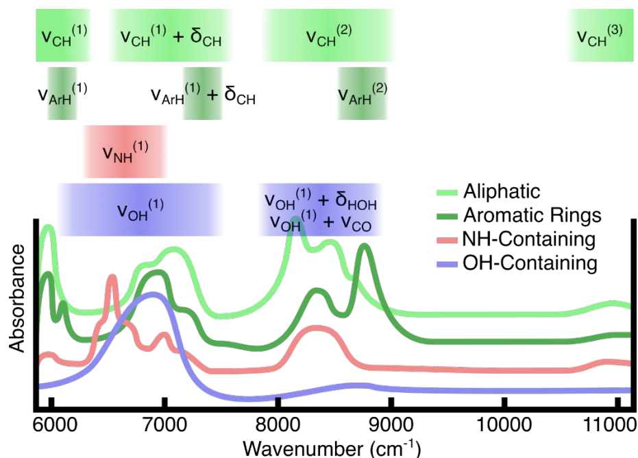
Figure 3 Schematic of the notable peaks in the NIR region. Primary identifying regions for the plastics are the combination band of the CH stretch first overtone and the CH bend ( \nu_{\text{CH}}^{(1)} + \delta_{\text{CH}} ) as well as the CH stretch second overtone ( \nu_{\text{CH}}^{(2)} ). These and the aromatic CH bands are shown in green. The water spectral features are shown in blue, and the NH spectral features are shown in red.
