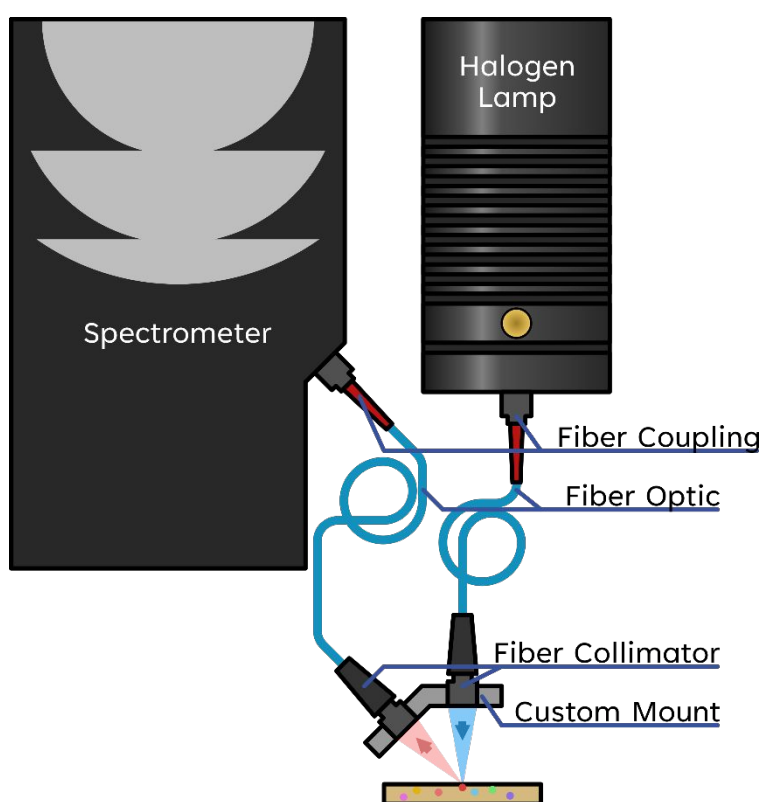
Figure 1 Schematic of the near infrared (NIR) instrument. A broadband light source is focused onto a sample and the remitted light is collected at a 45° angle between the illumination and collection sources. The collected light is sent to a spectrometer for measurement, as described in the text.
