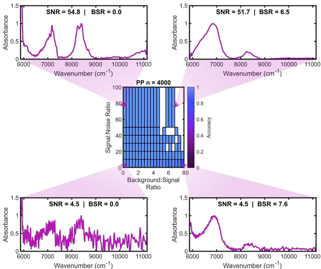
Figure 6. Two-dimensional histogram tiles illustrating the performance of the cubic SVM model trained on spectral data augmented with both noise and interferences for polypropylene. Signal-to-noise ratios (SNR) are shown on the y-axis, interferent-to-signal ratios (BSR) on the x-axis, and accuracy is depicted by the color scale. White regions indicate areas without data. A sample spectrum from each quadrant of the plot is included, with frequency ( \text{cm}^{-1} ) on the x-axis and absorbance on the y-axis. As SNR decreases, spectral features become increasingly unclear by noise, while higher BSR values reflect greater overlap of spectral features by those of water and plant matter.
