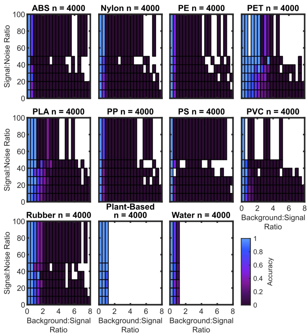
Figure 8 Two-dimensional histogram tiles showing the performance of the cubic SVM model trained on spectral data augmented with noise only for each plastic, with signal-to-noise ratios (SNR) on the y-axis, interferent-to-signal ratios (BSR) on the x-axis, and accuracy represented by the color scale. White regions have no data.
