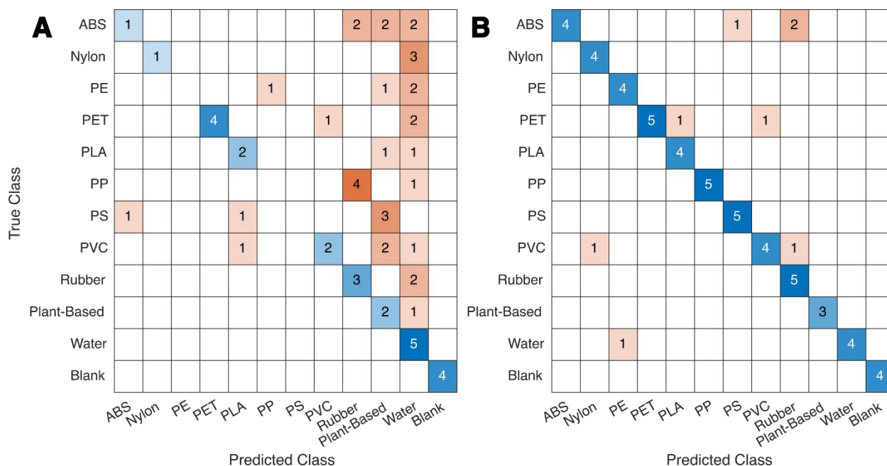
Figure 9 Confusion matrix of the cubic SVM model trained on spectral data augmented with noise only. (Interferents-free model) (A), and the cubic SVM model trained on spectral data augmented with both noise and interferents (B) tested on the authentic testing set. The x-axis represents the predicted class, while the y-axis represents the true class. True positives are represented by the diagonal elements, indicating correctly classified samples. False positives are shown as off-diagonal elements in a column, where a sample is incorrectly classified into a certain class. False negatives are represented by off-diagonal elements in a row, where a sample is incorrectly excluded from its true class. The model B shows the reduced misclassifications compared to the model A.
