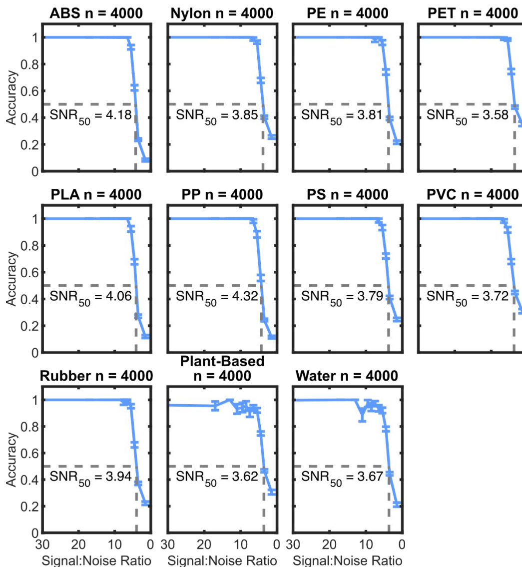
Figure 10 Accuracy of the cubic SVM model trained on interferences evaluated on noisy data with added interferences as the testing dataset, plotted across different signal-to-noise ratios (SNRs). Data is plotted as a line plot of histogram data with the horizontal axis representative of the histogram bin centers. Error bars are standard deviations determined by bootstrapping the accuracy estimates 100 times with 50% of the data each time. Gray dashed lines indicate the SNR at which the model is 50% accurate as determined via linear interpolation.
