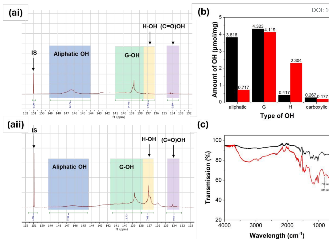
Figure 10. (a) Liquid-state ^{31}\text{P} NMR collected of phosphitylated (i) KL and (ii) and KL-Ph. (b) Graph summarising the amounts of each different OH group present in KL before (black) and after (red) phenolation. (c) FTIR spectra of KL (black) and KL-Ph (red),
