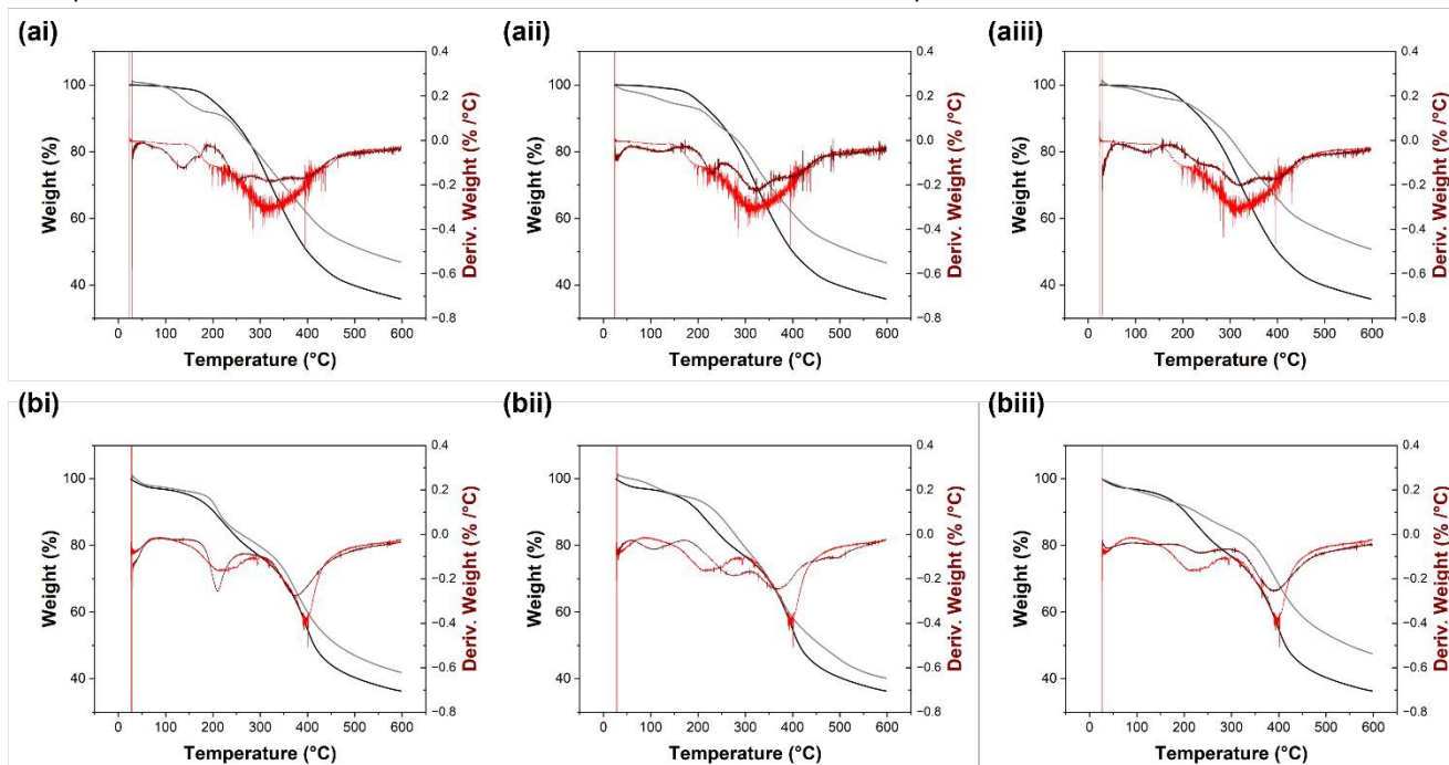
Fig. 15. TGA thermograms collected for (ai) SL-BZ-aniline, (aii) SL-BZ-A, (aiii) SL-BZ-B, (bi) SL-PhBZ-aniline, (bii) SL-PhBZ-A and SL-PhBZ-B (dark red and grey). Thermograms for (a) SL and (b) SL-Ph are shown in light red and black in each graph for comparison.
