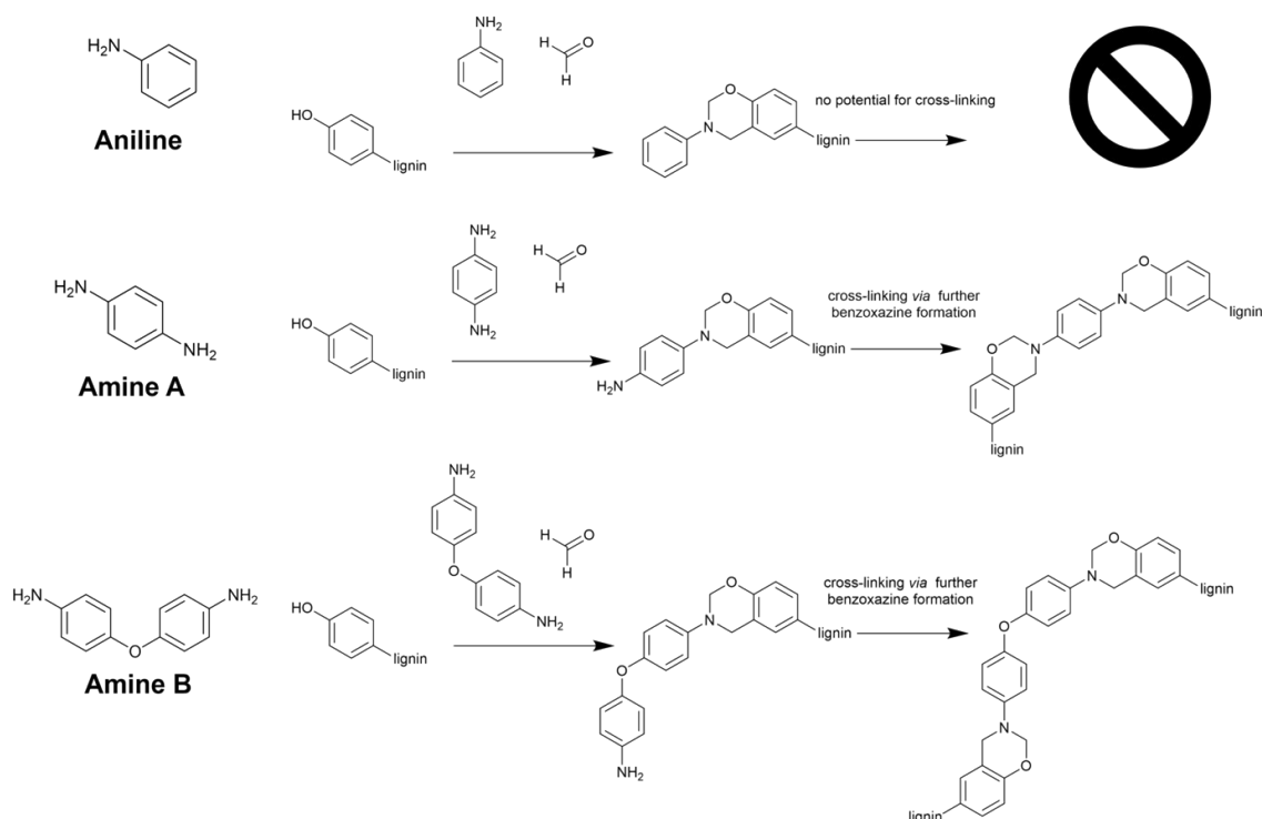
Figure 2. BZ synthesis using lignin as the phenol and aniline, Amine A (para-phenylene diamine) or Amine B (bis-(4-aminophenyl)ether) as the amine. Using diamine compounds,
