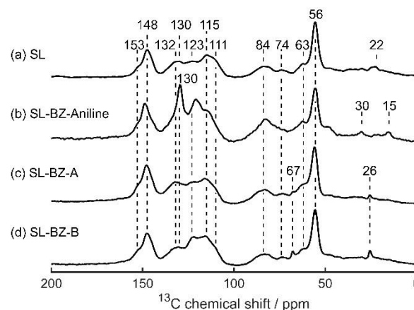
Figure 6. Solid-state ^{13}\text{C} CP MAS NMR spectra of (a) SL, (b) SL-BZ-Aniline, (c) SL-BZ-A, and (d) SL-BZ-B. Chemical shift values (in ppm) of each peak are indicated.
