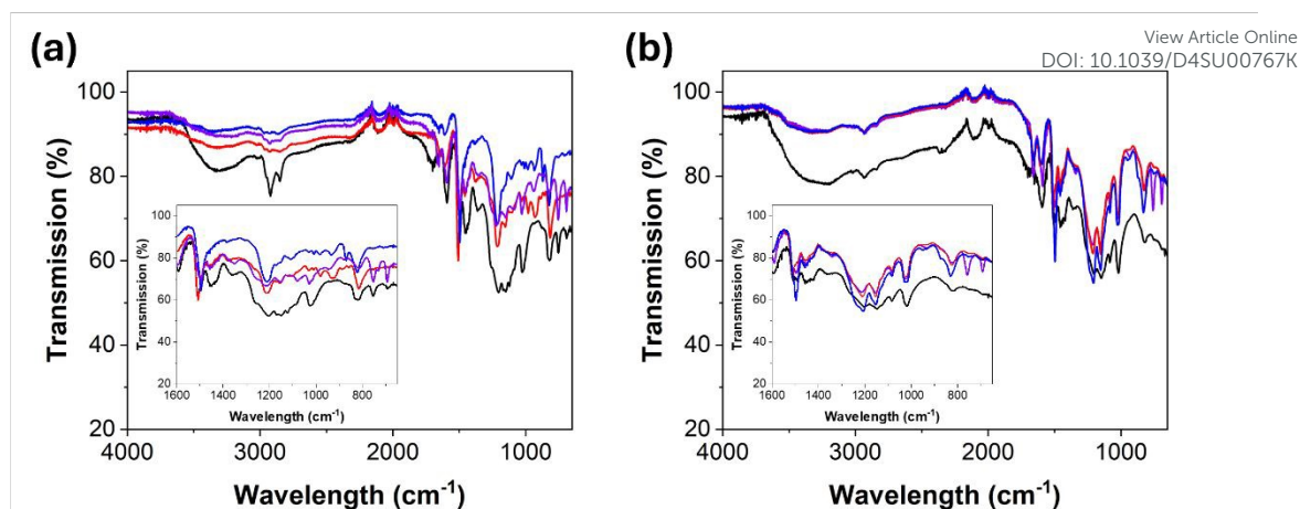
Figure 12. FTIR spectra of unmodified (a) SL-Ph (black), SL-PhBZ-aniline (purple), SL-PhBZ-A (red) and SL-PhBZ-B (blue) and (b) KL-Ph (black), KL-PhBZ-aniline (purple), KL-PhBZ-A (red) and KL-PhBZ-B (blue).
