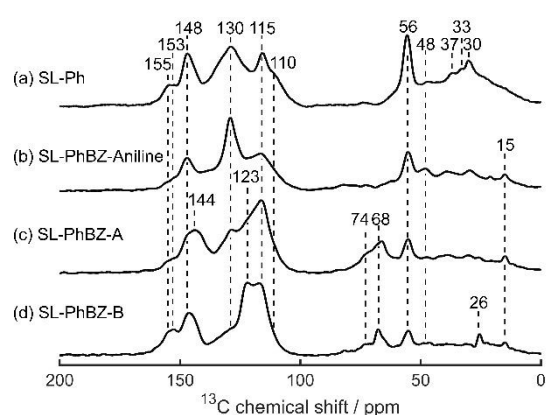
Figure 13. Solid-state ^{13}\text{C} CP MAS NMR spectra of (a) SL-Ph, (b) SL-PhBZ-Aniline, (c) SL-PhBZ-A, and (d) SL-PhBZ-B. Chemical shift values (in ppm) of each peak are indicated.
