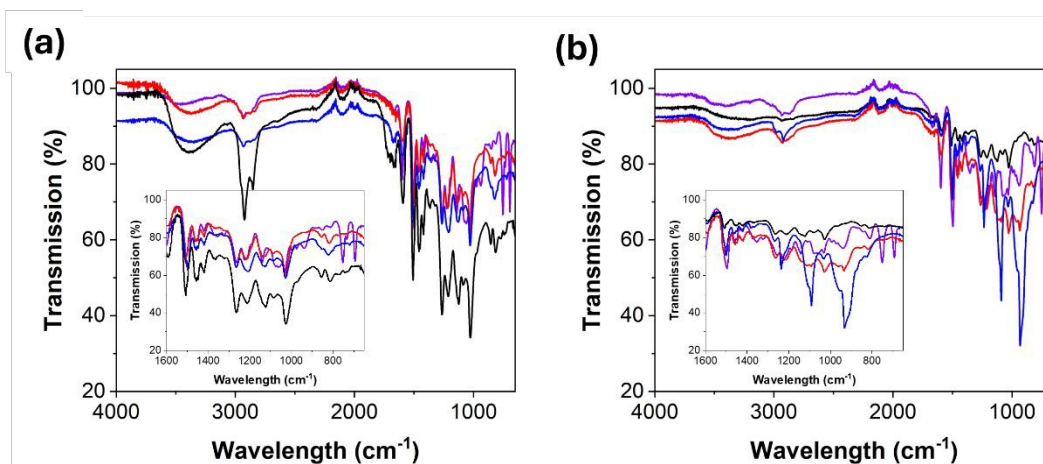
Figure 5. FTIR spectra of unmodified (a) SL (black), SL-BZ-aniline (purple), SL-BZ-A (red) and SL-BZ-B (blue) and (b) KL (black), KL-BZ-aniline (purple), KL-BZ-A (red) and KL-BZ-B (blue).
