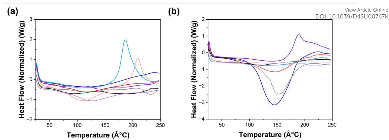
Figure 17. DSC curves collected for (a) SL (black), SL-Ph (grey), SL-BZ-aniline (purple), SL-PhBZ-aniline (pale purple), SL-BZ-A (red), SL-PhBZ-A (pale red), SL-BZ-B (blue), SL-PhBZ-B (pale blue); (b) KL (black), KL-Ph (grey), KL-BZ-aniline (purple), KL-PhBZ-aniline (pale purple), KL-BZ-A (red), KL-PhBZ-A (pale red), KL-BZ-B (blue), KL-PhBZ-B (pale blue)
