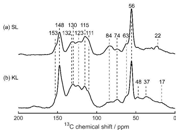
Figure 3. Solid-state ^{13}\text{C} CP MAS NMR spectra of (a) Sonichem lignin and (b) Kraft lignin. Chemical shift values (in ppm) of each peak are indicated.
