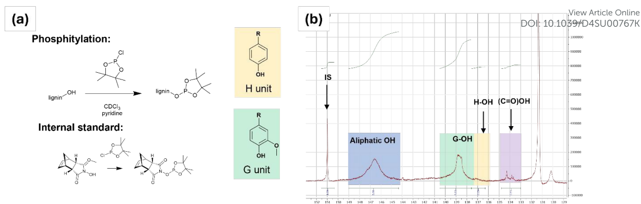
Figure 4. (a) Schematics showing phosphitylation of the OH groups in lignin using the chosen phosphitylating agent, phosphitylation of the internal standard, and the aromatic units present in SL. (b) Liquid-state ^{31}\text{P} NMR spectra recorded of phosphitylated Sonichem lignin.
