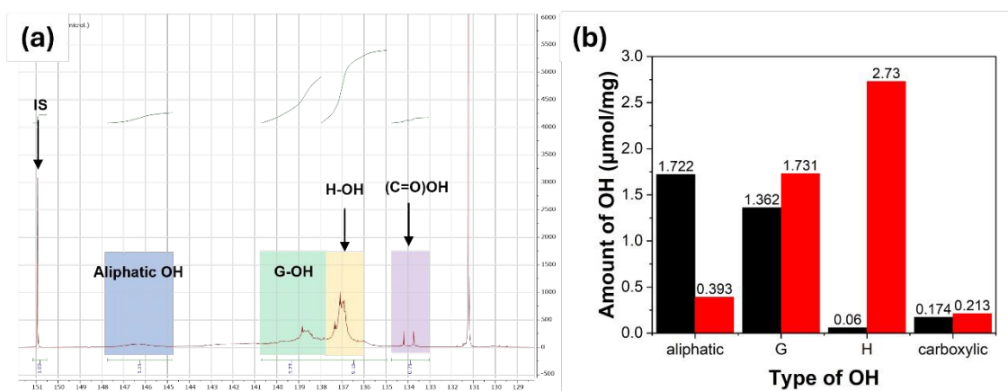
Figure 8. (a) Liquid-state 31 P NMR spectra recorded of SL-Ph. (b) Graph summarising the amounts of each type of OH group in SL before (black) and after (red) phenolation of SL, according to comparison with the internal standard.
