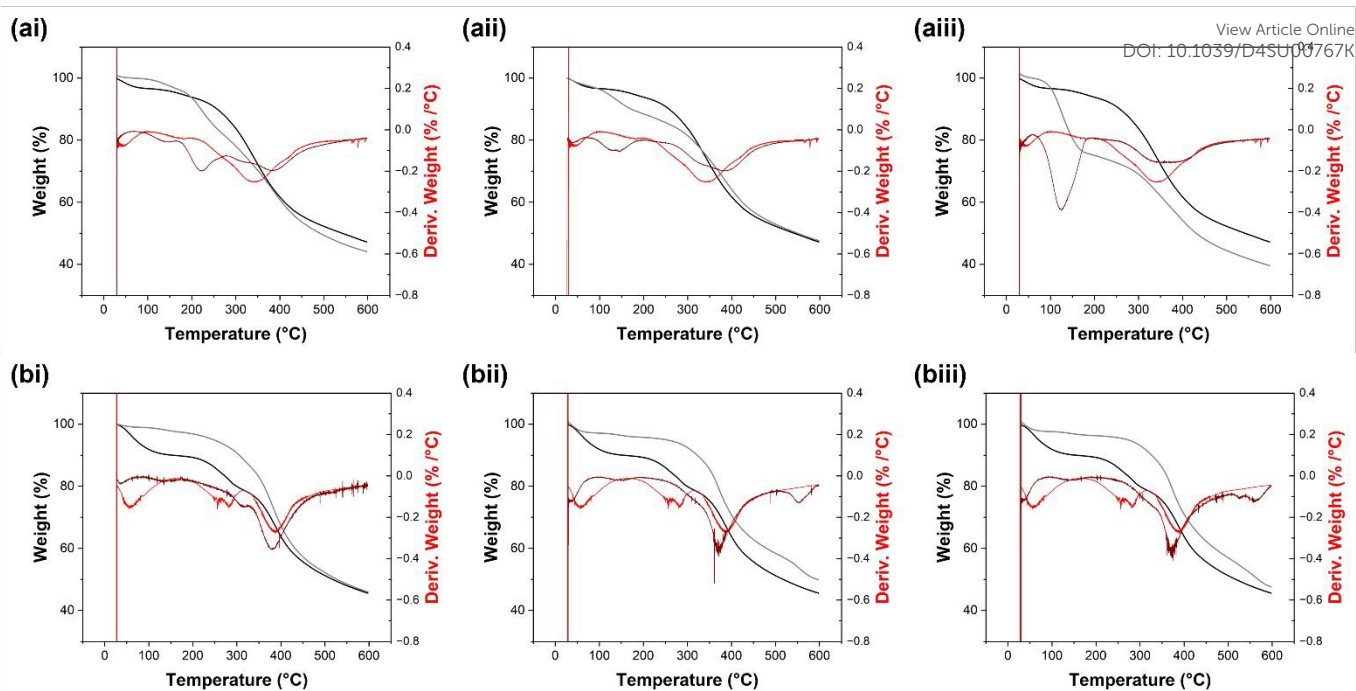
Figure 16. TGA thermograms collected for (ai) KL-BZ-aniline, (aii) KL-BZ-A, (aiii) KL-BZ-B, (bi) KL-PhBZ-aniline, (bii) KL-PhBZ-A and KL-PhBZ-B. Thermograms for (a) KL and (b) KL-Ph are shown in light red and black in each graph for comparison.
