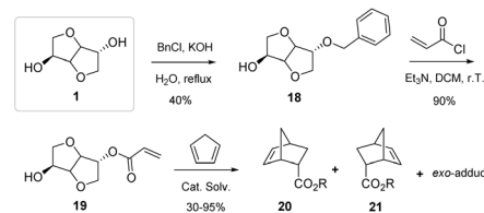
Fig. 17 Diels–Alder reaction of an acrylate derived from exo -mono-benzylated isosorbide and cyclopentadiene. 42
