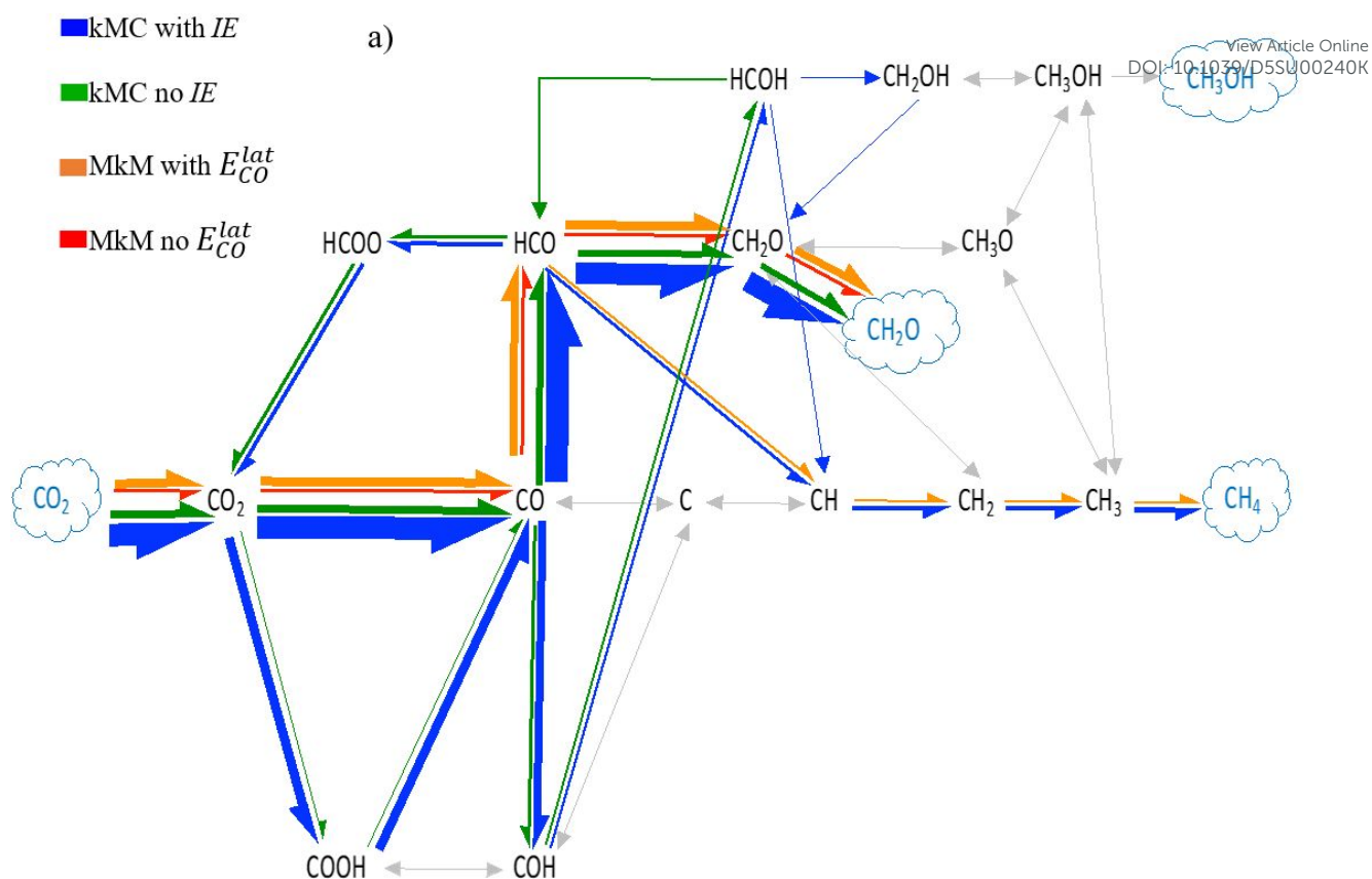
Fig. 3 Schematic representation of the most plausible mechanism for (a) the CO_2 hydrogenation and (b) the
