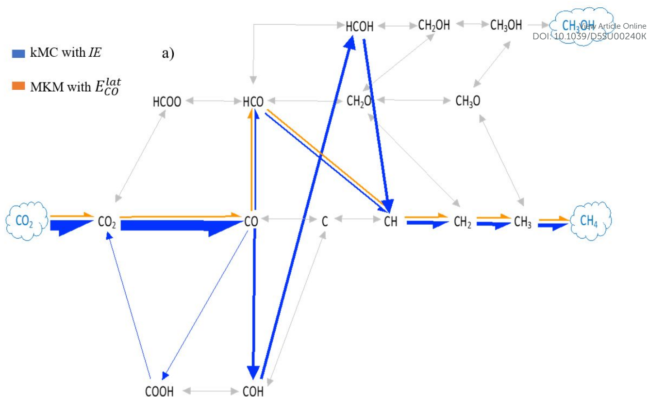
Fig. 4 Schematic representation of the most plausible mechanism for the (a) CO 2 hydrogenation and (b) the H 2(g)
