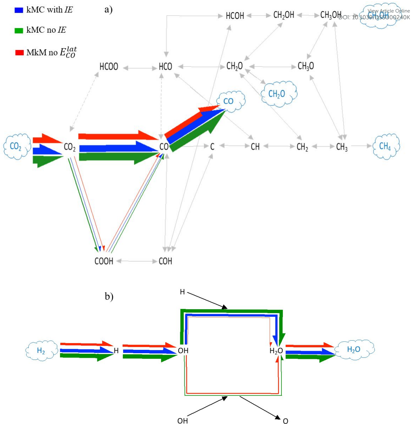
Fig. 2 Schematic representation of the most plausible mechanism for the (a) \text{CO}_2 hydrogenation and (b) the \text{H}_{2(g)} transformation into \text{H}_2\text{O}_{(g)} over Ni(111) at T = 673.15 \text{ K} and P = 10 \text{ bar} with a \text{CO}_2:\text{H}_2 molar ratio of 1:4 for both kMC (blue), MkM (red) and kMC simulations without IE (green). Coloured arrows refer to produced events while grey arrows are for events that do not happen (continuous) or happen at the same rate in both forward and backwards directions (dashed). Arrow's thickness symbolizes the net event frequency of each elementary process. For details on the calculations for the arrow's thickness the reader is referred to Section S5.
