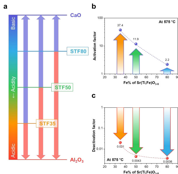
Figure 4. Relative Smith acidity of SrTi_{1-x/100}Fe_{x/100}O_{3-6} (STF x , x = 35, 50, 80 ) specimens and their infiltrates, along with trends in degree of activation. (a) Qualitative relative Smith acidity of the STF x specimens, along with that of CaO, and Al_2O_3 . (b) Activation factor in case of CaO infiltration (c) Deactivation factor in case of Al_2O_3 infiltration.
