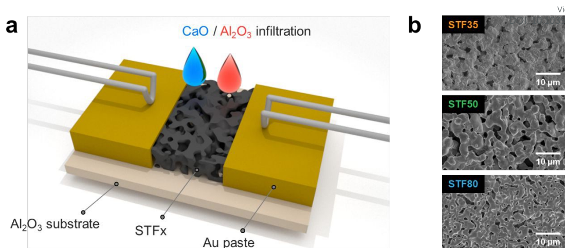
Figure 1. Experimental set-up for measuring surface oxygen exchange coefficient, k_{chem} , of porous specimens. (a) Schematic of dc conductivity measurement set-up and (b) Surface morphology of \text{SrTi}_{1-x/100}\text{Fe}_{x/100}\text{O}_{3-\delta} samples ( x = 35, 50, 80 )
