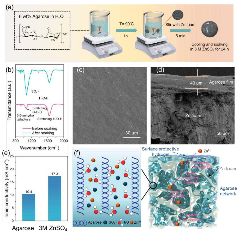
Figure 1. Fabrication and characterization of the interdigitated 3D electrode. (a) Schematic showing the preparation of ZF-Agarose electrode. (b) FTIR spectra of agarose gel before and after soaking into 3M \text{ZnSO}_4 electrolyte. (c) A representative scanning electron microscope (SEM) image of the soaked agarose gel surface. (d) A cross-section SEM image of the ZF-Agarose electrode. (e) The comparison of ionic conductivity between agarose hydrogel and aqueous 3M \text{ZnSO}_4 electrolyte. (f) Schematic demonstration of hydrogel-foam interdigitated electrode for rapid \text{Zn}^{2+} transport.
