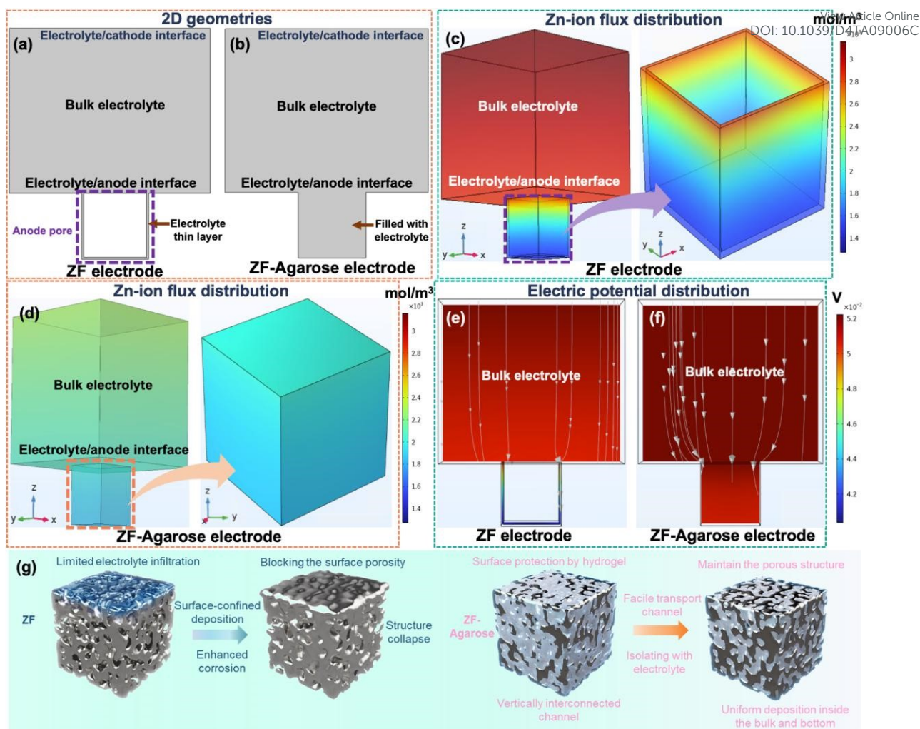
Figure 4. The COMSOL simulation of ion flux and electric field distribution and schematic representation of deposition regimes. The basic 2D simulation model for (a) ZF and (b) ZF-Agarose electrodes. The Zn-ion flux distribution of (c) ZF and (d) ZF-Agarose electrode. The electric potential distribution of (e) ZF and (f) ZF-Agarose electrodes. (g) Schematic diagram of ZF and ZF-Agarose electrode for illustration of different Zn-deposition manners.
