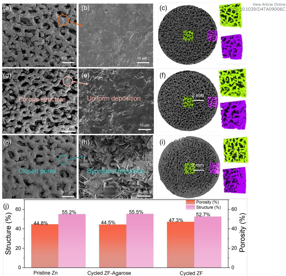
Figure 3. The Zn deposition and corresponding tomographic characterization. Representative SEM images of (a, b) pristine ZF electrode and cycled (d, e) ZF-Agarose and (g, h) ZF electrode after 10 cycles at 2 mA- 2 mAh cm -2 with corresponding tomographic images (c, f, i) revealed by X-ray CT. (j) The comparison of porosity and structure (the volume of metallic Zn) for pristine ZF, cycled ZF-Agarose, and cycled ZF electrode obtained by X-ray CT.
