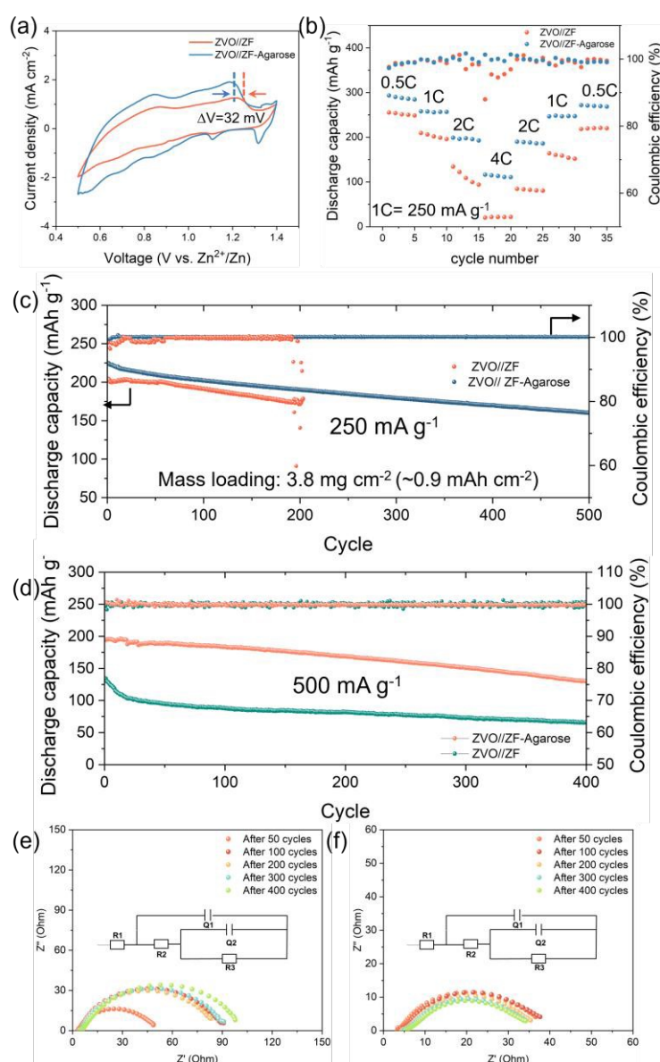
Figure 5. The comparison of full-cell performance for the two electrodes. (a) The CV profiles of ZVO||ZF-Agarose and ZVO||ZF full-cell at a scan rate of 0.5 \text{ mV s}^{-1} . (b) Rate performance of ZVO cathode with ZF and ZF-Agarose electrode under variable current rates. (c) The long-term cyclability for ZVO||ZF-Agarose cell and ZVO||ZF cell at (c) 250 \text{ mA g}^{-1} and (d) 500 \text{ mA g}^{-1} . The evolution of EIS spectra for (e) ZVO||ZF full-cell and (f) ZVO||ZF-Agarose full-cell obtained at 500 \text{ mA g}^{-1} . The inset in (d, e) shows the equivalent circuit model used to fit the impedance data. Further information is provided in the experimental details.
