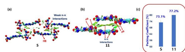
Figure 3. (a) and (b) NCI analysis of 5 and 11 ; (c) Packing coefficient of 5 and 11 .
