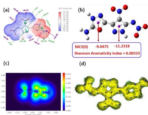
Figure 5: (a) The Electrostatic potential (ESP) maps (isodensity=0.0004 a.u.) of 11 ; (b) NICS(0) values at different position of 11 ; (c) LOL- \pi isosurface of 11 ; (d) AICD plot of 11 (Vectors moving clock-wise direction is indicated by the appropriate blue arrows).
