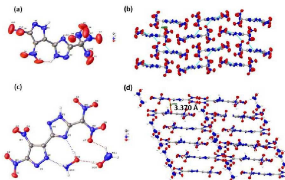
Figure 1. (a, c) Thermal ellipsoid plots (50%) of compounds 5 and 8 , respectively. (b, d) Molecular packing of compounds 5 and 8 , respectively.
