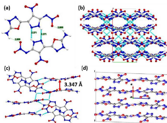
Figure 2. (a) hydrogen bonding interactions with a maximum D-D distance of 2.9 Å and a minimum angle of 120°. (b) Zigzag hydrogen bonding network. (c) Layered packing with π-π stacking interactions (3.347 Å). (d) Compact lattice showing tight molecular interlocking along the b-axis.
