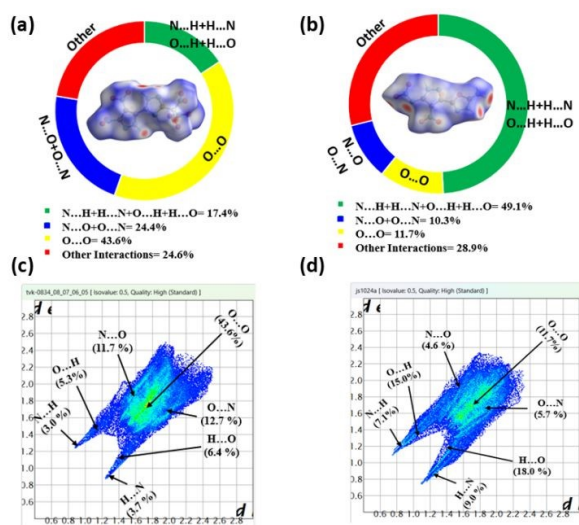
Figure 4. (a and c): Hirshfeld surface graph and 2D fingerprint plots of 5 , and (b and d) Hirshfeld surface graphs and 2D fingerprint plots of 11 .
