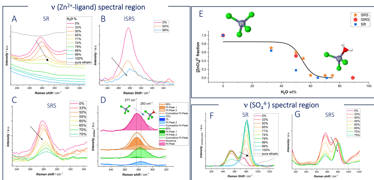
Fig. 4 (A–D) ν(Zn-ligand) and (F and G) ν(SO 4 2- ) spectra for pure anhydrous ethaline and DESEG-H 2 O hybrid electrolytes with the indicated water wt%: (A) spontaneous Raman; (B) Impulsive Stimulated Raman Scattering (ISRS); (C) Stimulated Raman Scattering (SRS); (D) fitted SRS curves. (E) [ZnCl 4 ] 2- fraction estimated for the fitting of the spectra of panels (A–D). (F) Spontaneous Raman. (G) SRS.
