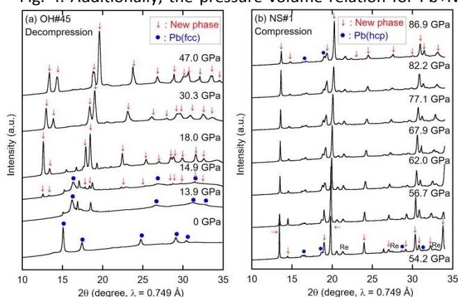
Fig.3 Pressure evolution of X-ray diffraction profiles (OH#45 and NS#1) (a) The XRD profile of the sample (OH#45) acquired during the decompression from 47 GPa. The top profile corresponds to the sample after heating at 47 GPa. Newly appeared peaks are marked with arrows. XRD patterns were acquired along the decompression to ambient pressure at room temperature. (b) The XRD profile of the sample (NS#1) was acquired during the compression from 54.2 GPa. The bottom profile corresponds to the laser-heated sample. The arrows correspond to the peaks of the newly synthesized compound as well as (a). XRD patterns were acquired along the compression to approximately 90 GPa under room temperature. Non-marked peaks might be derived from nitrogen and weak peaks from the rhenium gasket are detected with the labeling of "Re" in (b). There are still a few unidentified peaks that might represent other new compounds, which should be investigated further.
