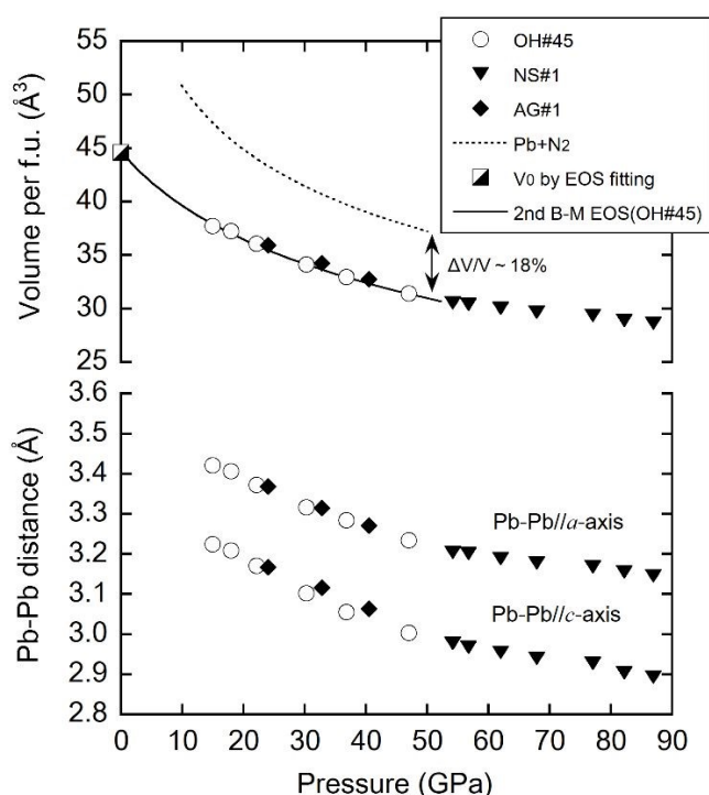
Fig.4 Pressure dependence of volume per formula unit and Pb-Pb distances. The bulk modulus volume at ambient pressure (half-filled square) was determined by fitting pressure-volume data for OH#45 to B-M EOS. The equimolar volume of Pb+N 2 is represented as a dashed line calculated from the reported P-V data for Pb and N 2 . The Pb-Pb distances parallel to the a - and c -axes correspond to the lattice parameters of the tetragonal Pb-lattice, respectively.
