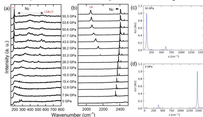
Fig.5 Pressure dependence of the measured (AG#2) and calculated Raman spectra. Two wavenumber regions are separately shown in (a) and (b). Newly appeared peaks are represented with \nu_i ( i=1-4 ). Wavenumber regions corresponding to the N 2 pressure medium are represented with horizontal arrows. Spiky peaks at low wavenumber regions at low pressures might be derived from the instruments or atmospheric species. Calculated Raman spectra of I4/mcm PbN 2 at 0 K (c) 50 GPa and (d) 0 GPa.
