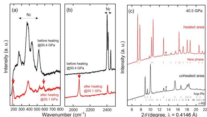
Fig.1 Raman spectra and XRD profiles under high pressures. (a) and (b) shows the Raman spectra corresponding to the \text{Pb}-\text{N}_2 sample (AG#1) before and after laser heating at approximately 50 GPa. Two wavenumber regions were separately displayed. Intense peaks after laser-heating are marked with arrows. The horizontal arrows show the wavenumber region derived from solid molecular nitrogen. (c) High-pressure in-situ X-ray diffraction profiles acquired from the heated and unheated areas. The diffraction peak positions of Pb, and \text{N}_2 are represented with tics at the bottom of the profiles. The intense peak positions derived from the new phase that appeared after laser heating are also indicated with tics. The peak marked with an asterisk might be derived from the device.
