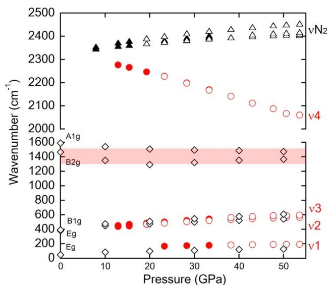
Fig.6 Pressure dependence of experimentally detected wavenumber (AG#2) together with wavenumbers of \text{PbN}_2 obtained by DFT calculation. Open and solid circles correspond to the different positions (position 1 and position 2) on the same sample, respectively. The spectra of position 2 are shown in Fig.S7. Open and solid triangles correspond to the wavenumbers of nitrogen from the same positions. The open diamond represents the wavenumbers of \text{PbN}_2 obtained by DFT calculation. The data are listed in Table S2. The Diamond-Raman band with the range of 1300-1500 \text{cm}^{-1} is hatched.
