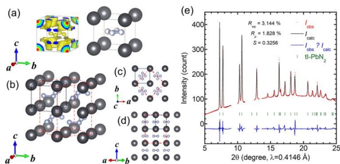
Fig.2 Charge density map, atomic arrangement, and refined XRD profile of newly synthesized \text{PbN}_2 . (a) Charge density map and corresponding atomic assignment of the tetragonal cell. Large and small half-filled balls correspond to Pb and N, respectively. (b) Atomic arrangements in the 2 \times 2 \times 2 extended cell of the initially obtained one. The nitrogen dimers alternatively align in the neighbor cell which was obtained by the energy calculation results. The initial obtained P lattice cell and extended cell ( I lattice) are represented with the dashed and dot-dashed lines, respectively. (c-d) Projected atomic arrangement along the c -axis and [110] direction, respectively. (e) LeBail refinement based on the tetragonal symmetry having the I lattice. The 2\theta regions where nitrogen diffraction peaks appeared are excluded from the refinements. The crystal structures are drawn with 3D visualization program
