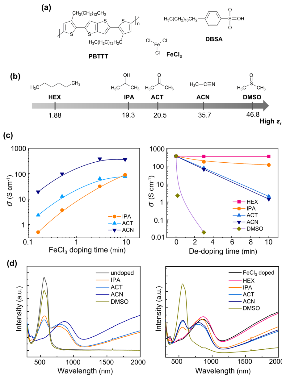
Fig. 1 (a) Chemical structures of PBTTT, FeCl 3 , and DBSA. (b) Chemical structures of solvents with different dielectric constants \epsilon_r . (c) The electrical conductivity \sigma and (d) the UV-vis-NIR spectra of PBTTT films after FeCl 3 doping with various solvents (left) and FeCl 3 -doped PBTTT films rinsed (dedoped) with various solvents (right).
