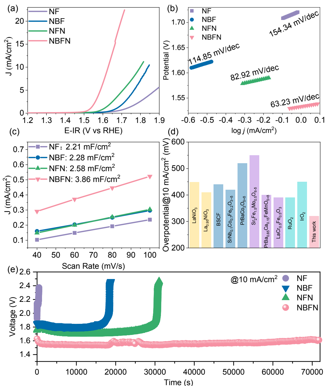
Figure 4. Electrochemical performance evaluation of perovskite catalysts. (a) LSV curves comparing OER activity of NF, NBF, NFN, and NBFN. (b) Tafel plots derived from LSV curves used to evaluate reaction kinetics. (c) Current density versus scan rate plots to determine electrochemical double-layer capacitance (Cdl) and ECSA. (d) Overpotential comparison of
