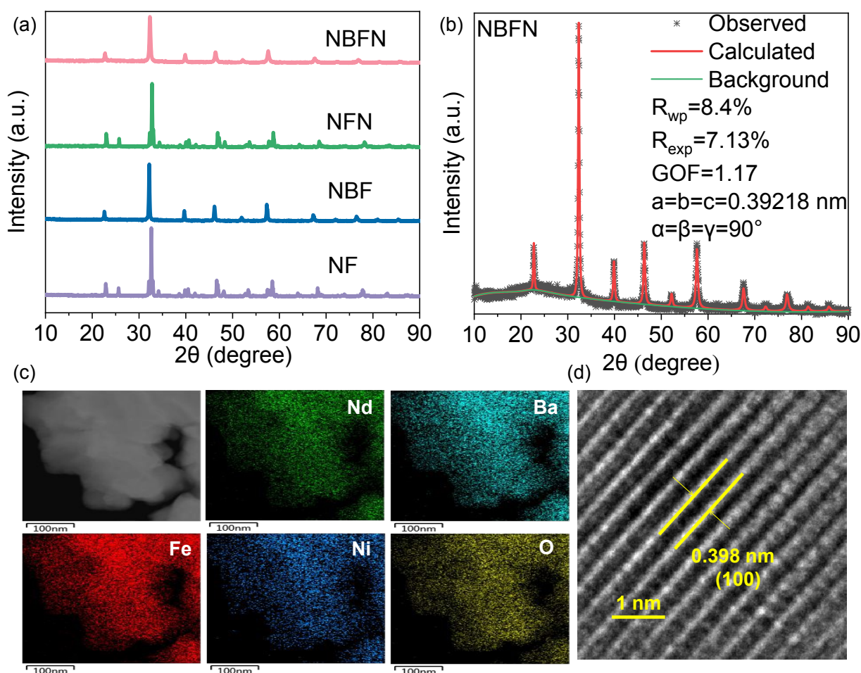
Figure 2. (a) X-ray diffraction (XRD) patterns of the synthesized NF, NBF, NFN, and NBFN perovskite powders. (b) Rietveld refinement of NBFN XRD profile. (c) Scanning transmission electron microscopy (STEM) image with corresponding energy-dispersive X-ray (EDX) elemental mapping of NBFN, showing the elemental distribution. (d) High-resolution transmission electron microscopy (HR-TEM) image showing the lattice spacing of NBFN.
