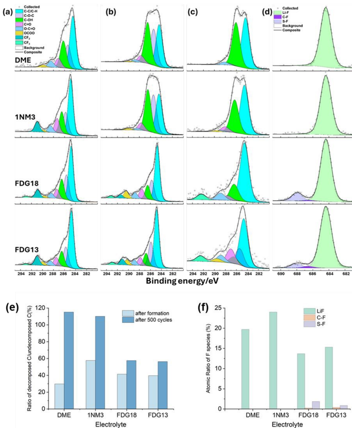
Figure 6. (a) The C 1s spectra of NMC811 cathode experiencing formation process, with sputtering time of 2 minutes; (b) The C 1s spectra of NMC811 cathodes experiencing 500 cycles, with 3 minutes of sputtering; (c) The C 1s spectra obtained on Si anode after 500 cycles, with 3 minutes of sputtering; (d) The F 1s spectra of Si anode experiencing 500 cycles, with 3 minutes of sputtering; (e) The atomic ratio between decomposed C species and undecomposed C species based on the peak analysis from (a) and (b); (f) The atomic ratio of different F species based on the peak analysis from (d).
