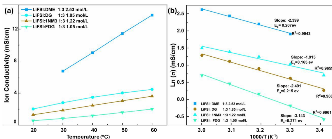
Figure 2. The (a) ion conductivity of probed electrolytes (for the LiFSI: DME 1:3 (molar: molar) electrolyte, the ion conductivity at 20 °C is missing because the electrolyte got frozen under 20 °C, as shown in Figure S4 ); (b) activation energies obtained from the Arrhenius equation for the tested electrolyte systems.
