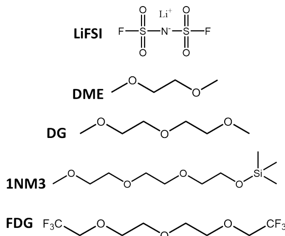
Scheme 1. Chemical structures of LiFSI salt and the other 4 etheral solvents (DME, DG, 1NM3, FDG) probed in this study
