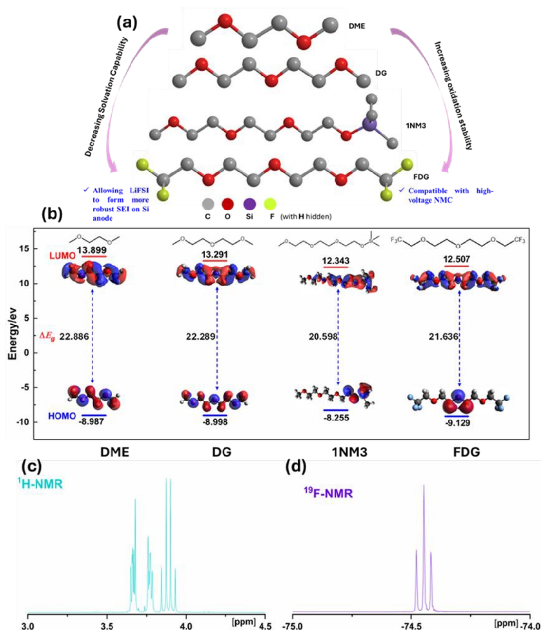
Figure 1. The rationale behind the utilization of the DME, DG, 1NM3 and FDG etheral solvent for NMC811||Si full cells (a) the chemical structures of the 4 solvents probed in this study; (b) the HOMO and LUMO levels of four solvent molecules obtained via DFT calculations with solvation effect considered; (c) the ^1\text{H-NMR} of synthesized FDG solvent; (d) the ^{19}\text{F-NMR} of synthesized FDG solvent.
