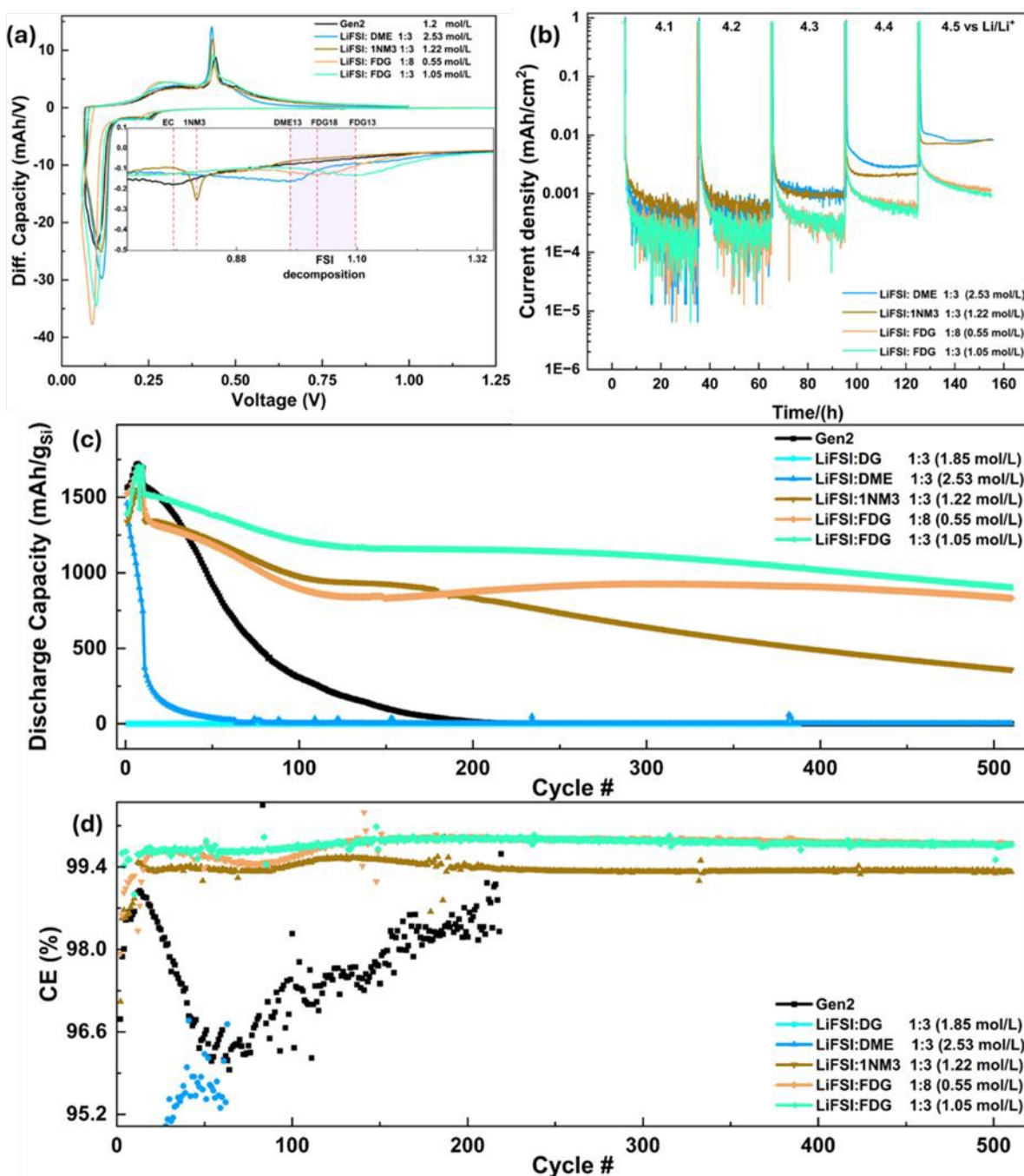
Figure 4. The electrochemical results for tested electrolyte systems: (a) the dQ/dV curves for these 5 electrolyte systems; (b) the voltage holding results on NMC811||Li half cells between 4.1–4.5 V vs. Li/Li + ; (c) the long-term cycling results for NMC811||Si full cells between 3.0–4.3 V vs. Li/Li + at C/3, the specific capacity is calculated based on the mass of Si; (d) the Coulombic efficiencies of the tested electrolytes during the long-term cycling.
