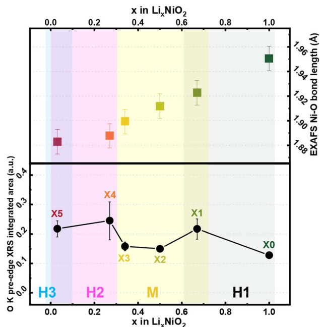
Fig. 8 The correlation between (top) the local Ni–O bond distances from EXAFS analysis and (bottom) the integrated area of the pre-edge of the O K-edge XRS spectra. Highlighted areas correspond to the global crystal phases indicated by H1, M, H2, and H3.
