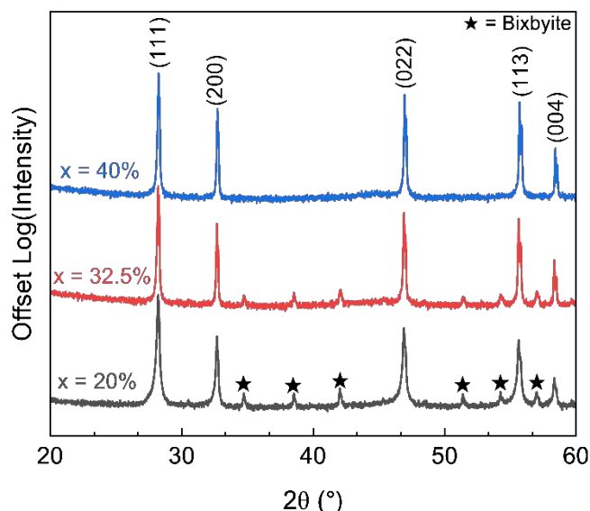
Figure 1: X-ray diffraction results of Ce_x(\text{SmPrLaY})_{1-x}\text{O}_{2-\delta} , shows that increasing the Ce content of the composition to 40% results in a single-phase fluorite structure. The black stars denote peaks related to the bixbyite, Ia\bar{3} symmetry. The main fluorite Fm\bar{3}m peak indices are indexed at the top of the figure.
