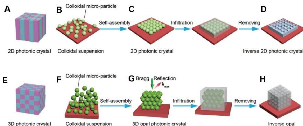
Fig. 5 (A, E) Schematic illustrations of 2D and 3D PC, respectively. (B – D) Self-assembly process of colloidal microparticles to form 2D monolayer PC and subsequently an inverse-structured crystal after removal of the template. (F – H) Self-assembly process for preparing a
