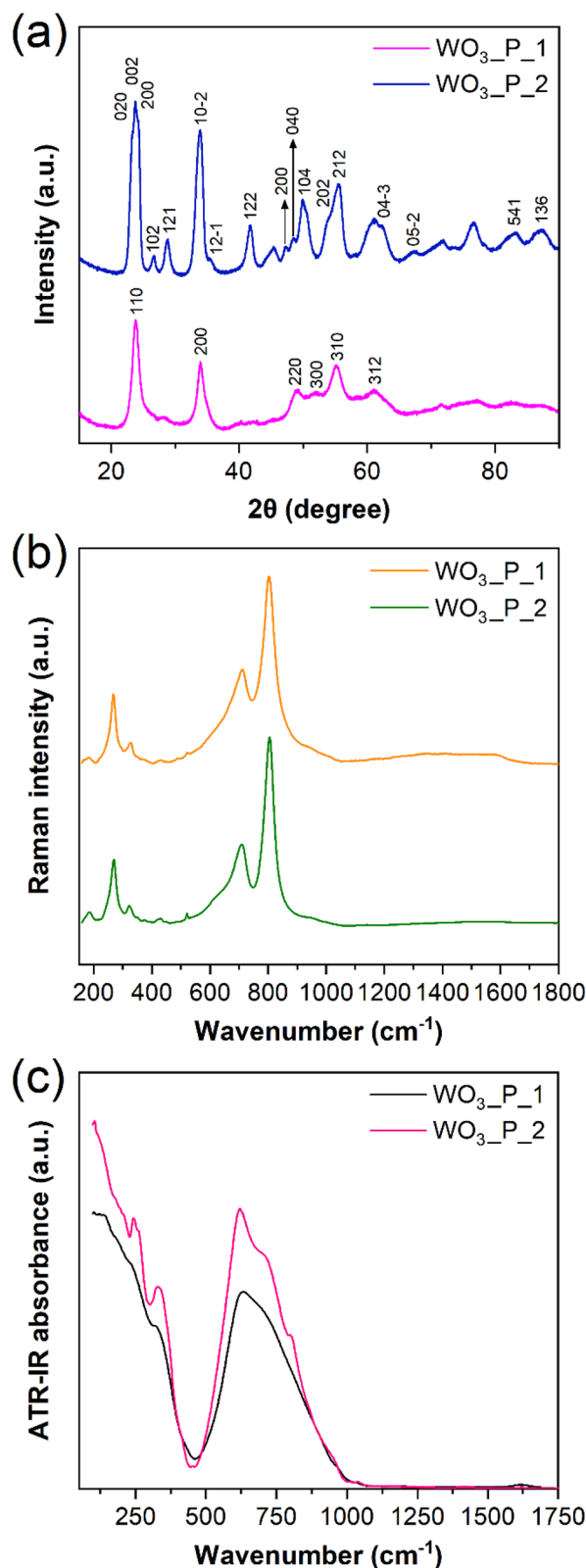
Fig. 1 (a) XRD patterns of \text{WO}_3\text{P}_1 and \text{WO}_3\text{P}_2 samples. (b) Raman spectra of \text{WO}_3\text{P}_1 and \text{WO}_3\text{P}_2 . (c) ATR-IR spectra of \text{WO}_3\text{P}_1 and \text{WO}_3\text{P}_2 .
